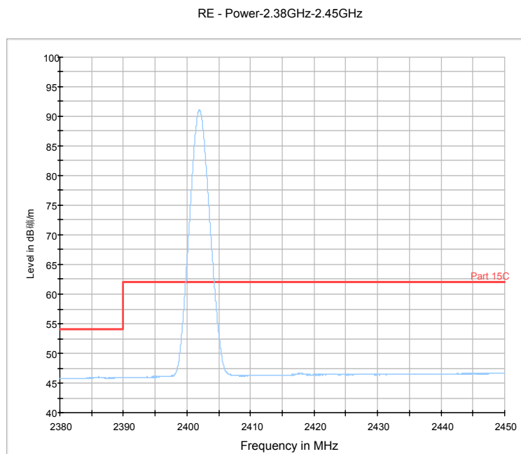
Fig.27. Radiated emission (Power): GFSK low channel
