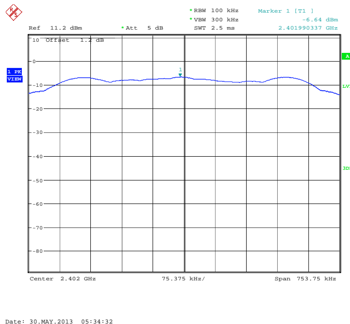
Fig.33. Maximum Power Spectral Density Level Function: GFSK, 2402 MHz
