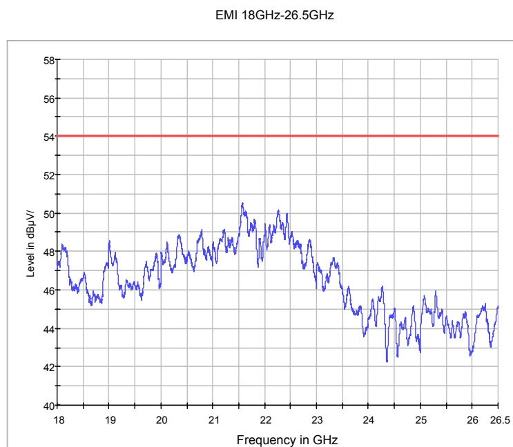
Fig.28. Radiated emission (Power): GFSK high channel
