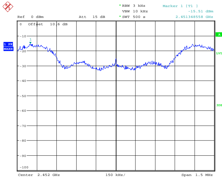
Fig. 11 Power Spectral Density (802.11n-HT40, Ch 6)
