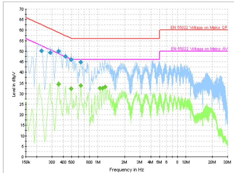
Fig. 176 AC Powerline Conducted Emission-802.11n-20MHz
