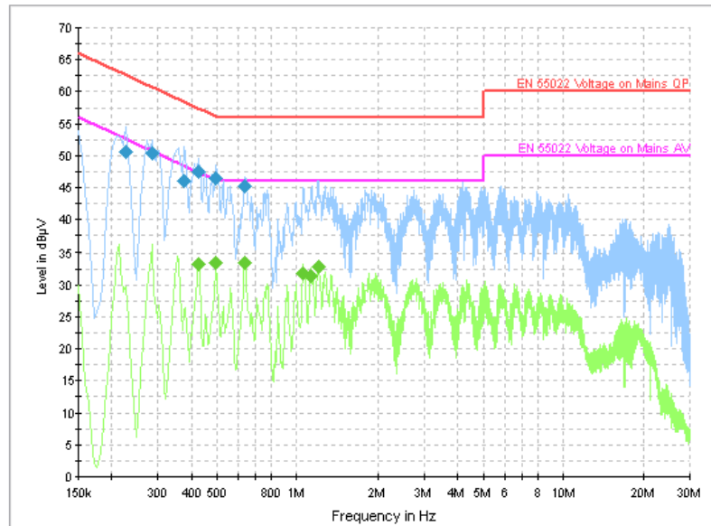
Fig. 177 AC Powerline Conducted Emission-802.11n-40MHz
