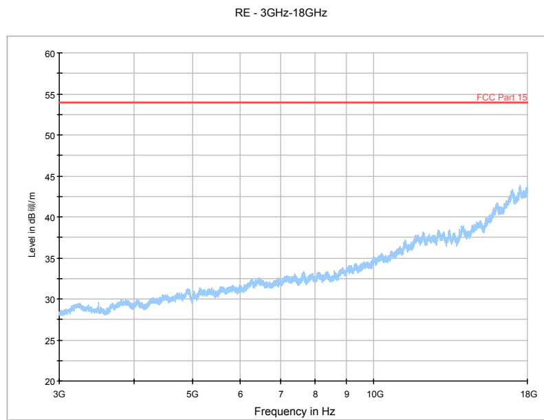
Fig. 132 Radiated Spurious Emission (802.11b, Ch1, 3 GHz-18 GHz)
