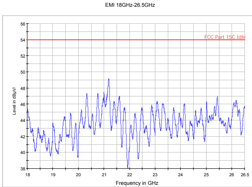
Fig. 173 Radiated Spurious Emission (All channels): 18GHz - 26.5GHz
