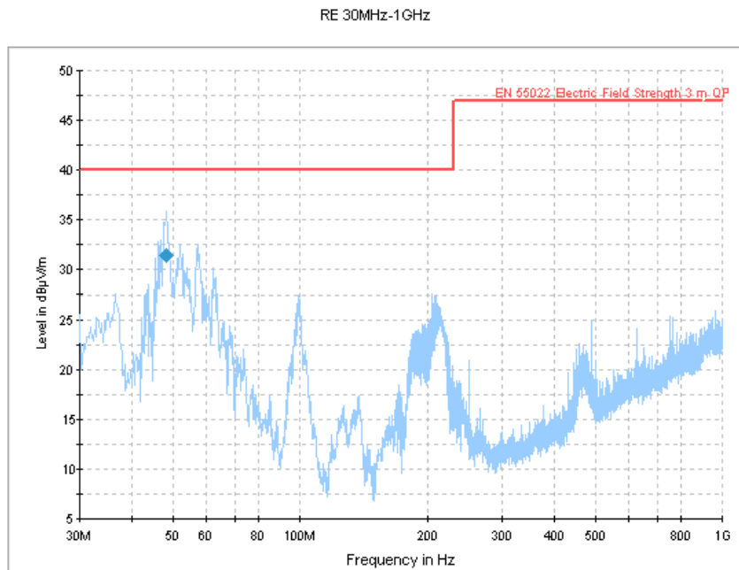
Figure B.7 Radiated Emission from 30MHz to 1GHz
