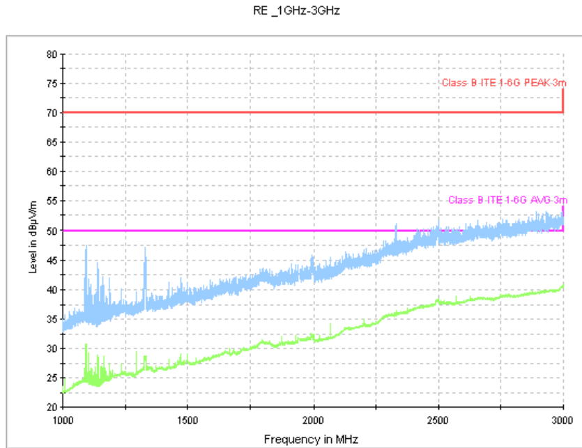
Figure B.11 Radiated Emission from 1GHz to 3GHz
