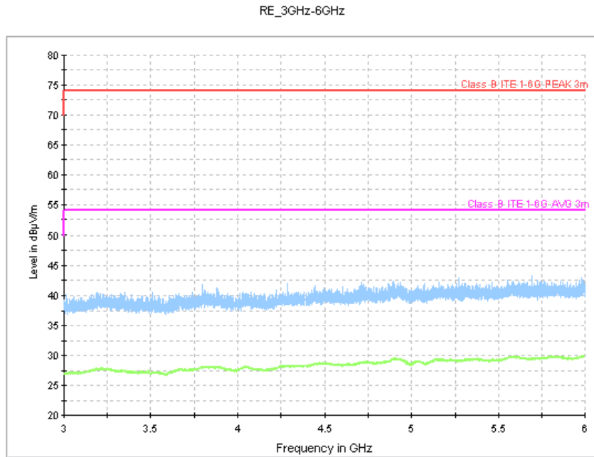
Figure B.9 Radiated Emission from 3GHz to 6GHz
