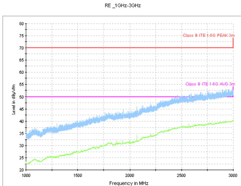
Figure B.8 Radiated Emission from 1GHz to 3GHz
