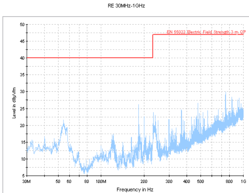
Figure B.10 Radiated Emission from 30MHz to 1GHz
