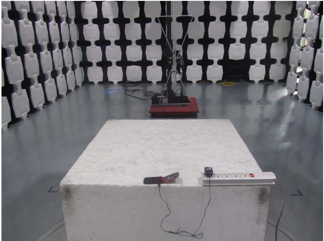
4. Radiated Emission(Charging)
