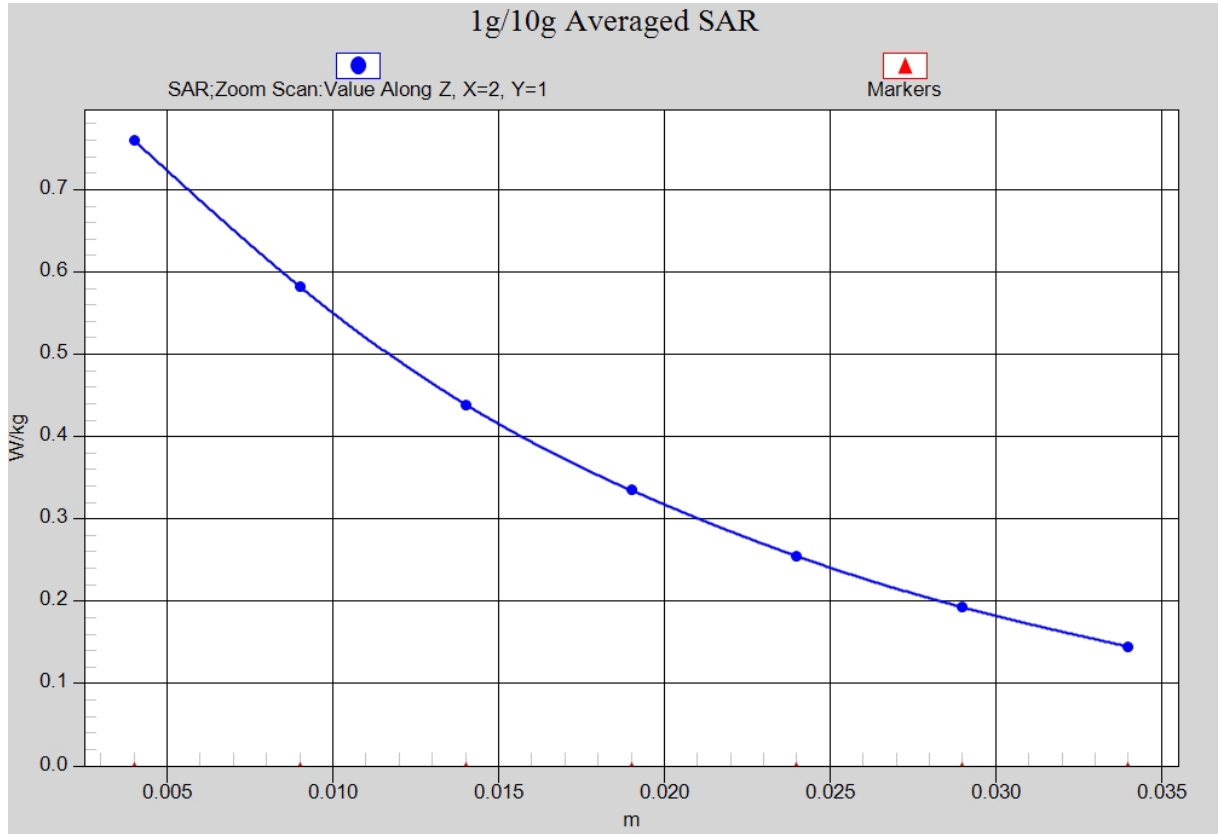
Fig. A.2-1 Z-Scan at power reference point (850 MHz CH128)
