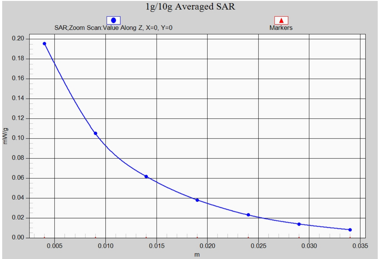
Fig. A.3-1 Z-Scan at power reference point (1900 MHz CH810)
