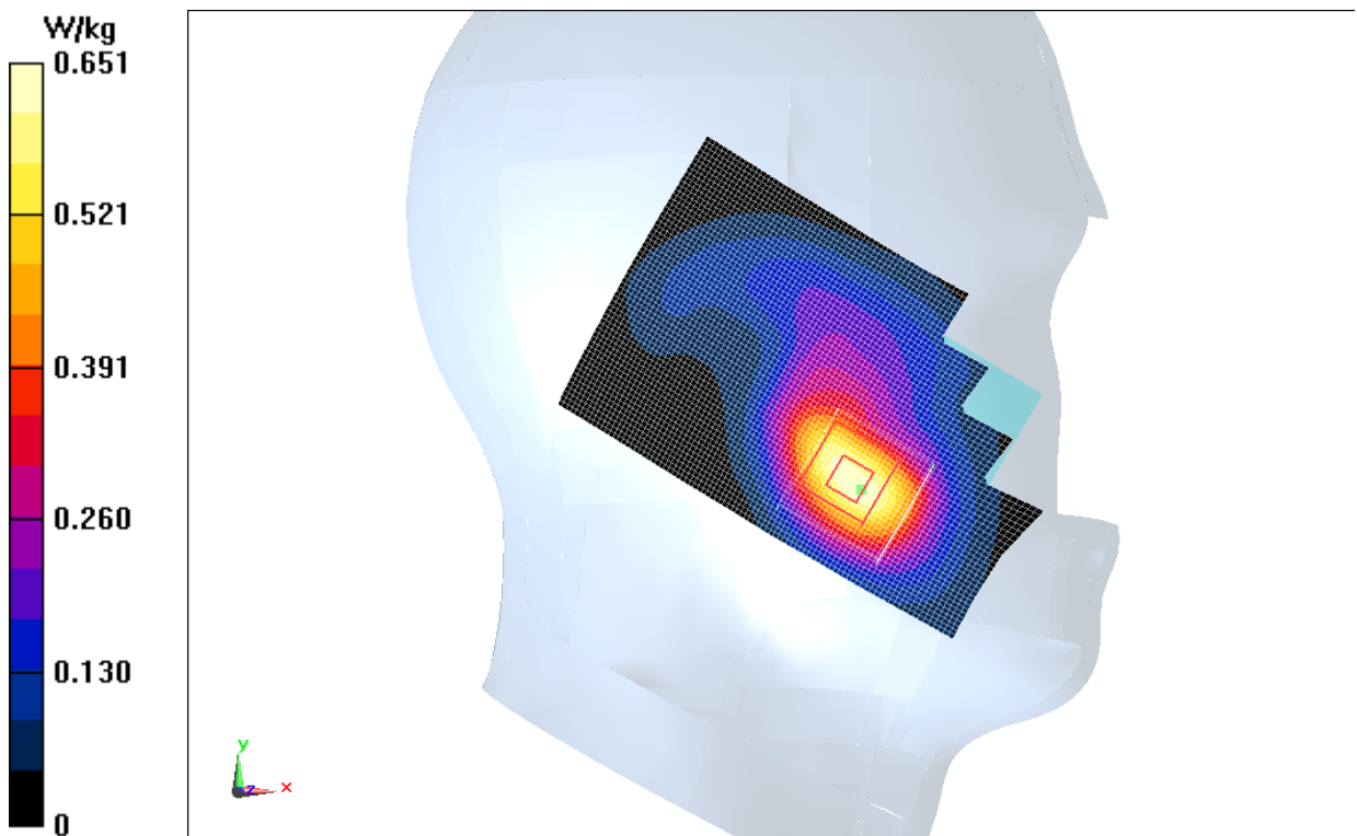
Fig.3 1900 MHz CH810
