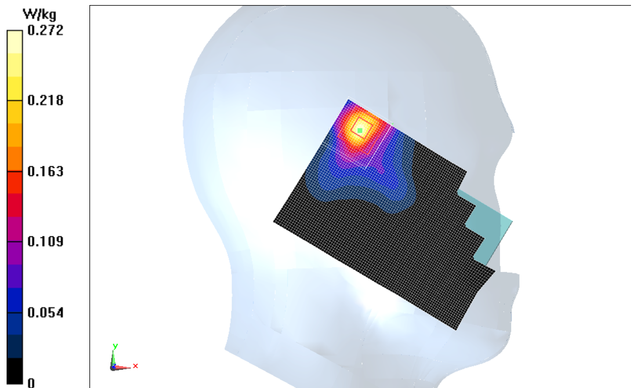
Fig.9 2450 MHz CH11
