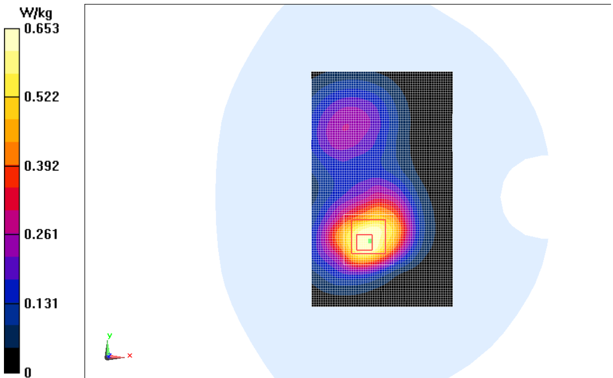
Fig.4 1900 MHz CH512
