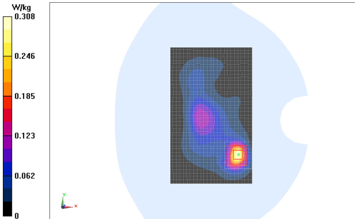
Fig.10 2450 MHz CH11
