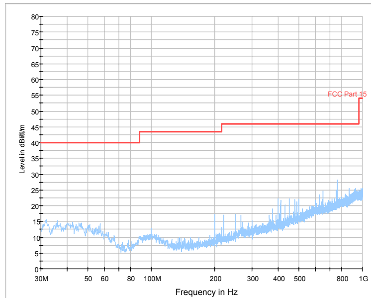
RE 30MHz-1GHz
