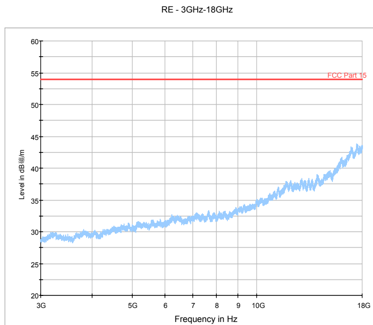
Fig.63. Radiated emission: GFSK, Channel 39, 3 GHz - 18 GHz
