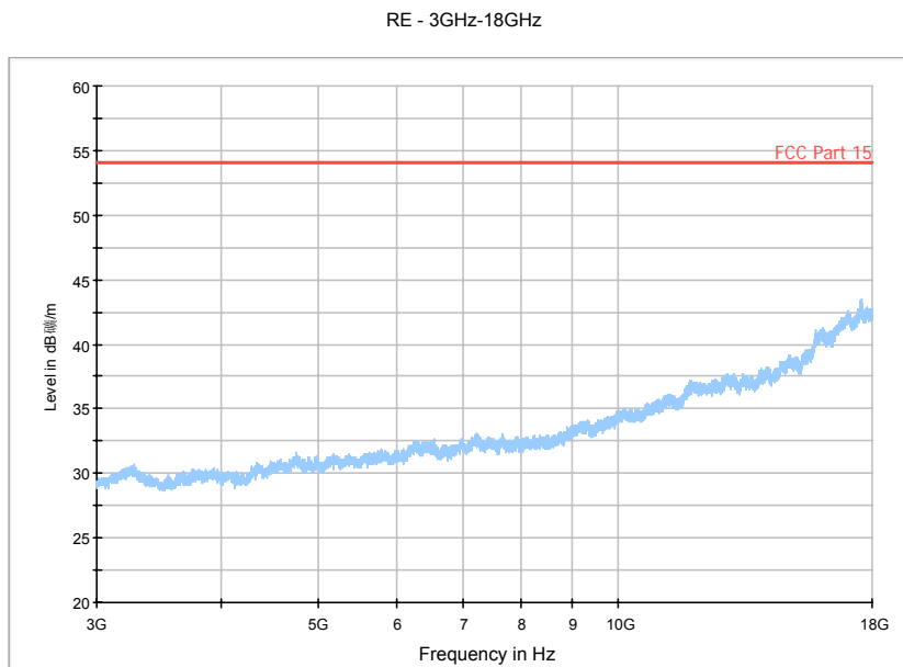
Fig. 154 Radiated Spurious Emission (802.11n-20MHz, Ch1, 3 GHz-18 GHz)
