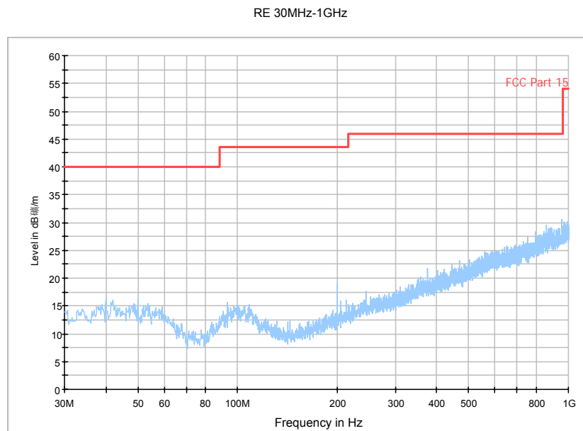
Fig. 166 Radiated Spurious Emission (802.11n-40MHz, Ch6, 30 MHz-1 GHz)
