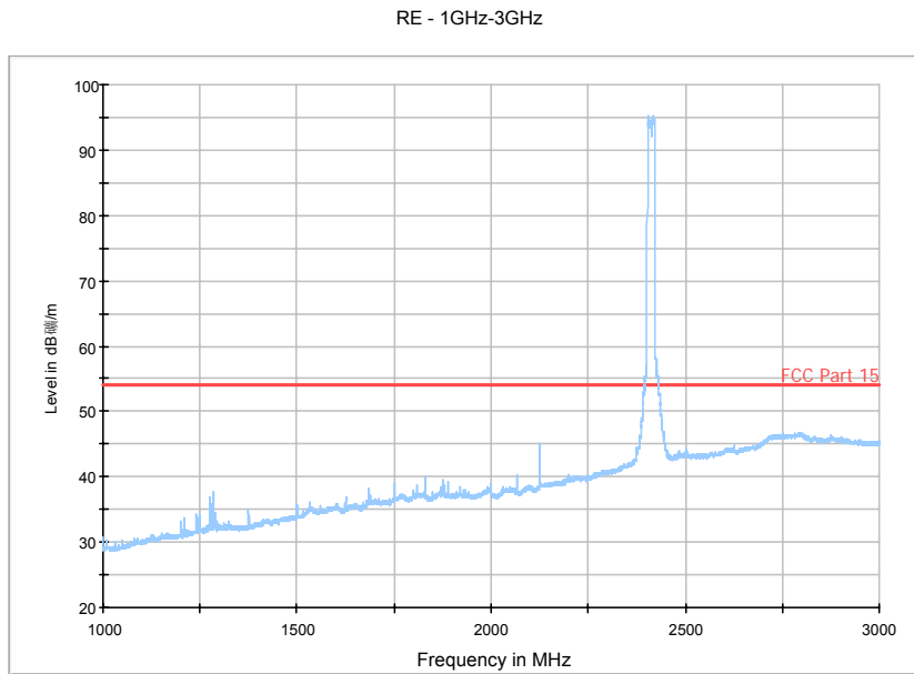
Fig. 153 Radiated Spurious Emission (802.11n-20MHz, Ch1, 1 GHz-3 GHz)
