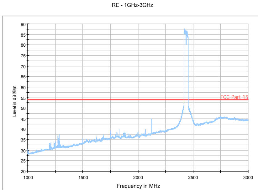
Fig. 167 Radiated Spurious Emission (802.11n-40MHz, Ch6, 1 GHz-3 GHz)
