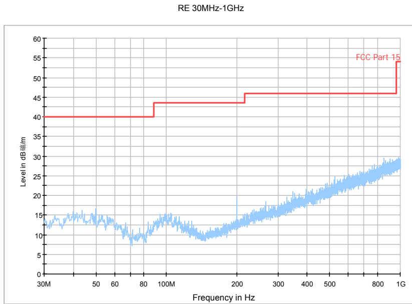
Fig. 163 Radiated Spurious Emission (802.11n-40MHz, Ch3, 30 MHz-1 GHz)
