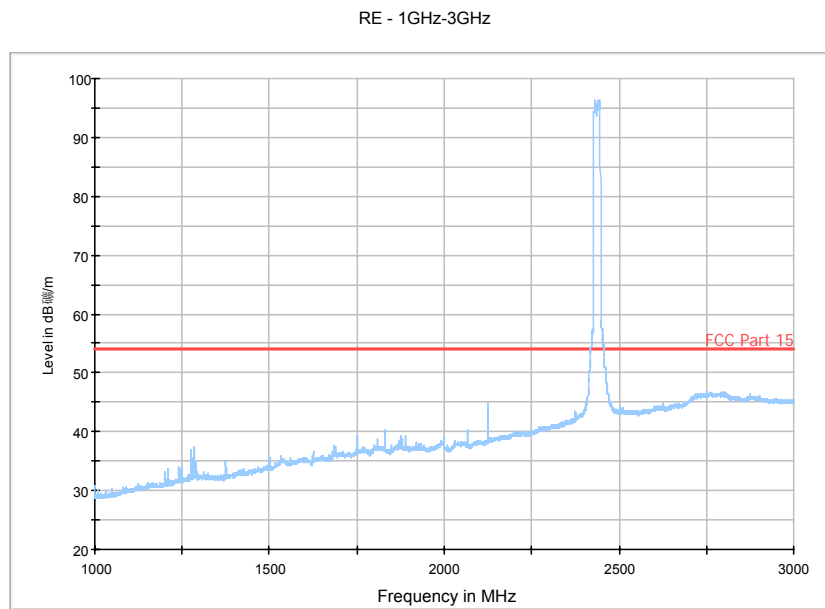
Fig. 156 Radiated Spurious Emission (802.11n-20MHz, Ch6, 1 GHz-3 GHz)
