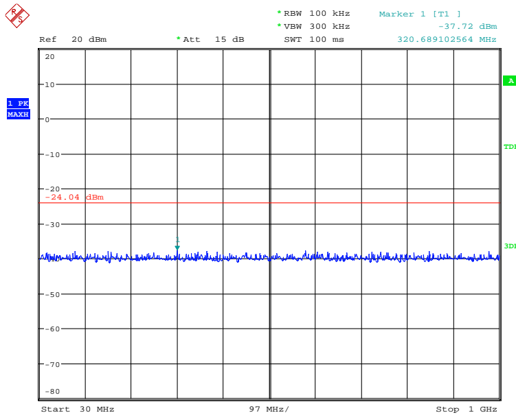
Fig. 113 Conducted Spurious Emission (802.11n-HT40, Ch6, Center Frequency)
