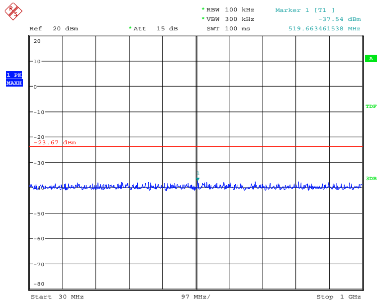
Fig. 121 Conducted Spurious Emission (802.11n-HT40, Ch9, Center Frequency)
