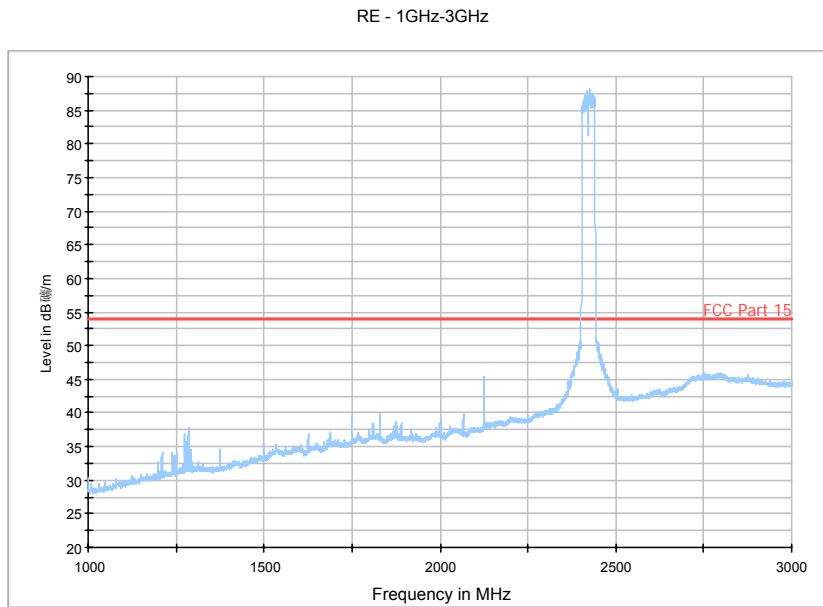
Fig. 164 Radiated Spurious Emission (802.11n-40MHz, Ch3, 1 GHz-3 GHz)
