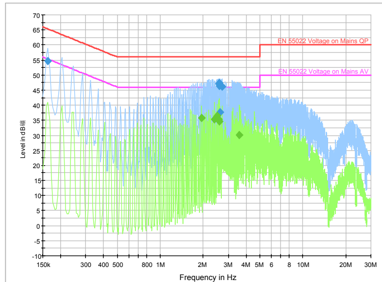
Fig. 174 AC Powerline Conducted Emission-802.11b (charger 1)
