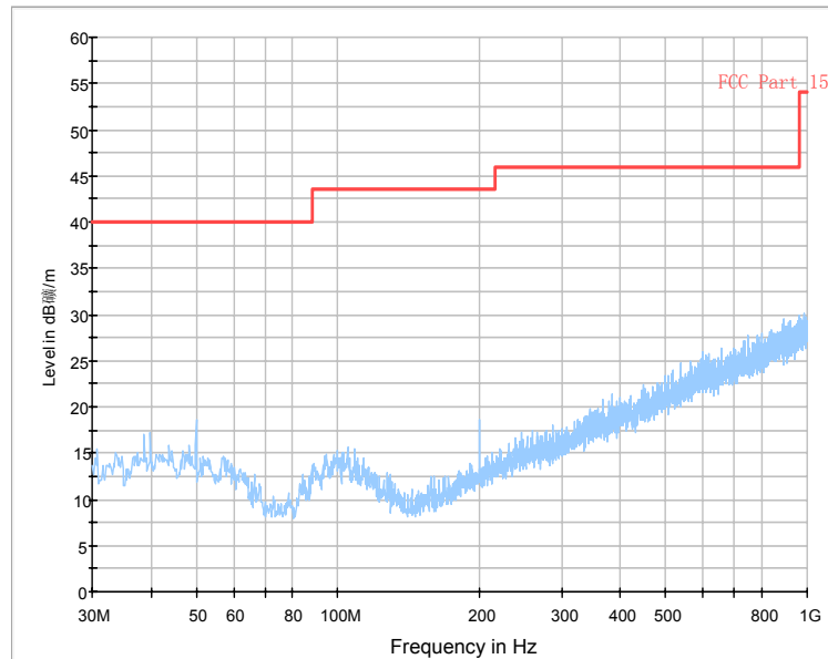
RE 30MHz-1GHz
