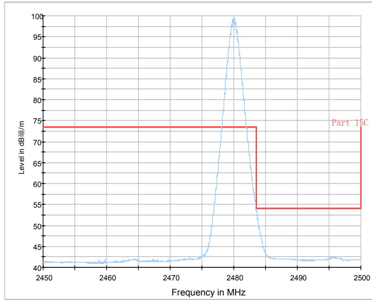
RE - Power-2.45GHz-2.5GHz
