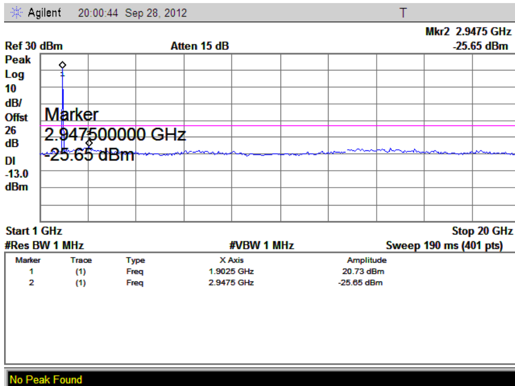
(Plot G3.1: HSUPA1900MHz Channel = 9538 1GHz to 20GHz)
