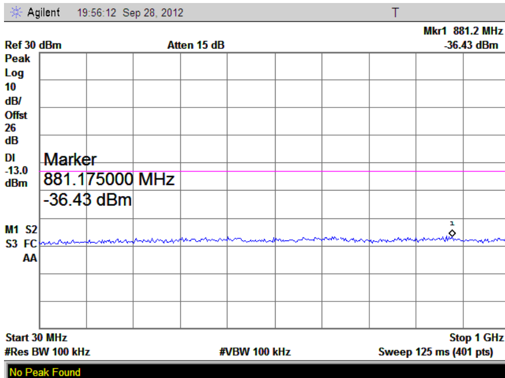
(Plot G2: HSUPA1900MHz Channel = 9400, 30MHz to 1GHz)
