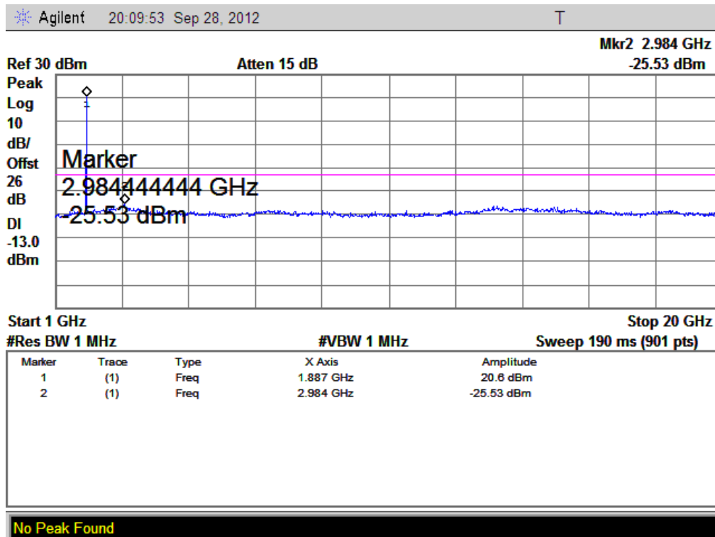
(Plot G1.1: HSUPA1900MHz Channel = 9262, 1GHz to 20GHz)
