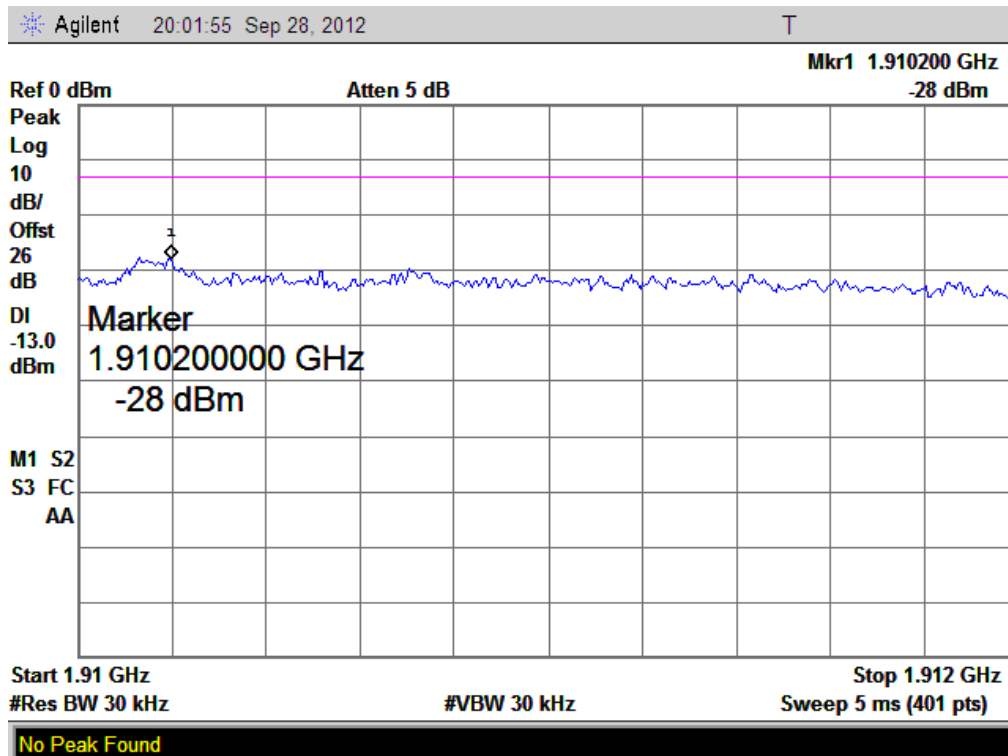
(Plot N: HSUPA 1900 Channel = 9538)
