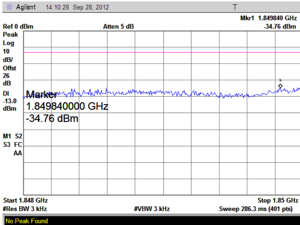
(Plot I: WCDMA 1900 Channel = 9262)
