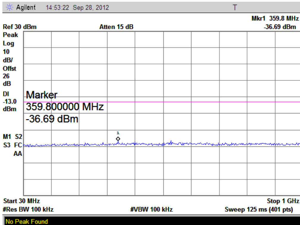
(Plot E1: WCDMA1900MHz Channel = 9262, 30MHz to 1GHz)
