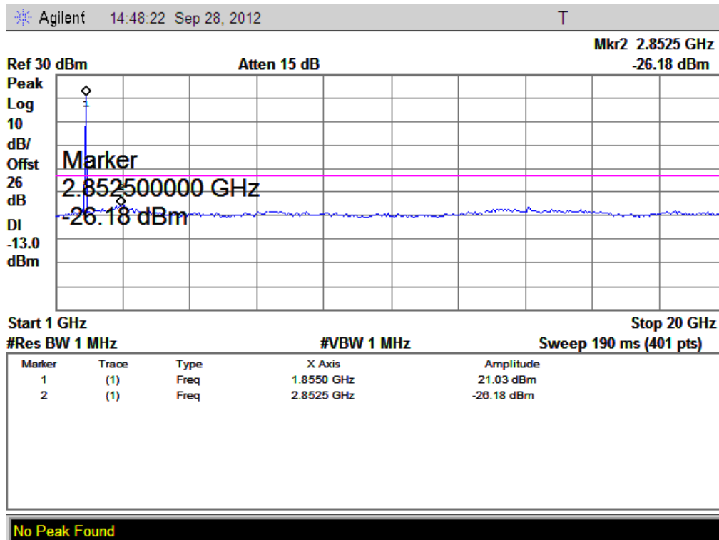
(Plot E1.1: WCDMA1900MHz Channel = 9262, 1GHz to 20GHz)
