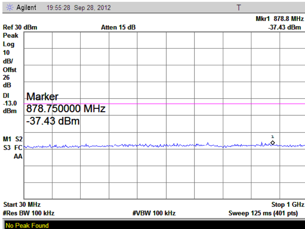
(Plot G 1: HSUPA1900MHz Channel = 9262, 30MHz to 1GHz)
