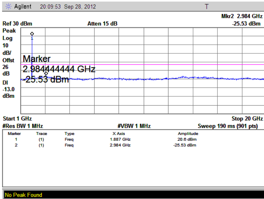
(Plot G2.1: HSUPA1900MHz Channel = 9400, 1GHz to 20GHz)
