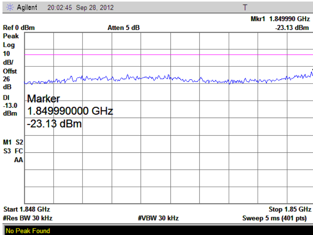
(Plot M: HSUPA 1900 Channel = 9262)
