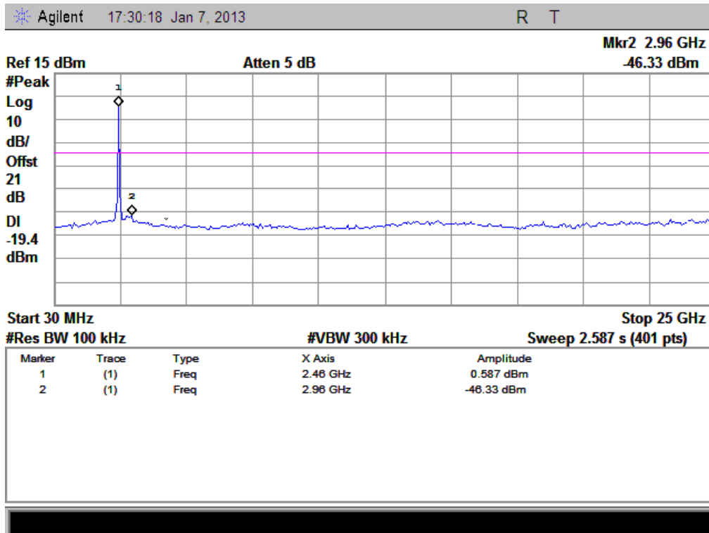
(Plot L.1: Channel = 9, 30MHz to 25GHz)
