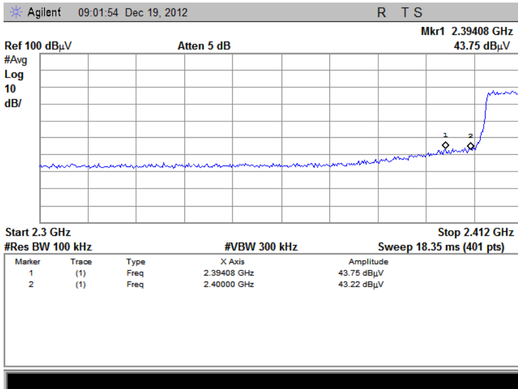
(Plot G2: Channel = 3 AVG@802.11n-40)
