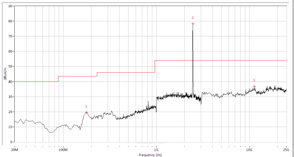
(Plot I.2: Antenna Horizontal, 30MHz to 25GHz)
