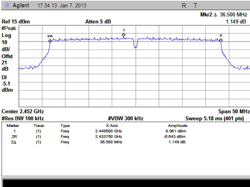
(Plot L: Channel 9: 2452MHz @ 802.11n-40)
