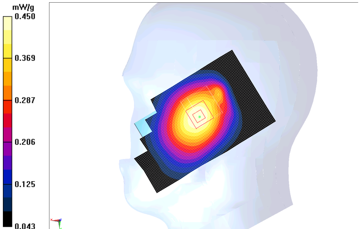
Fig.11 850 MHz CH190
