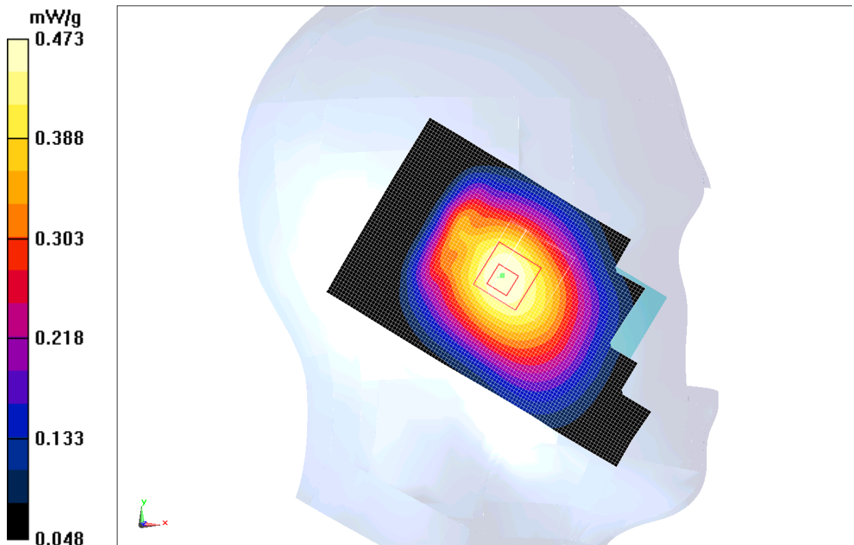
Fig.4 850 MHz CH251
