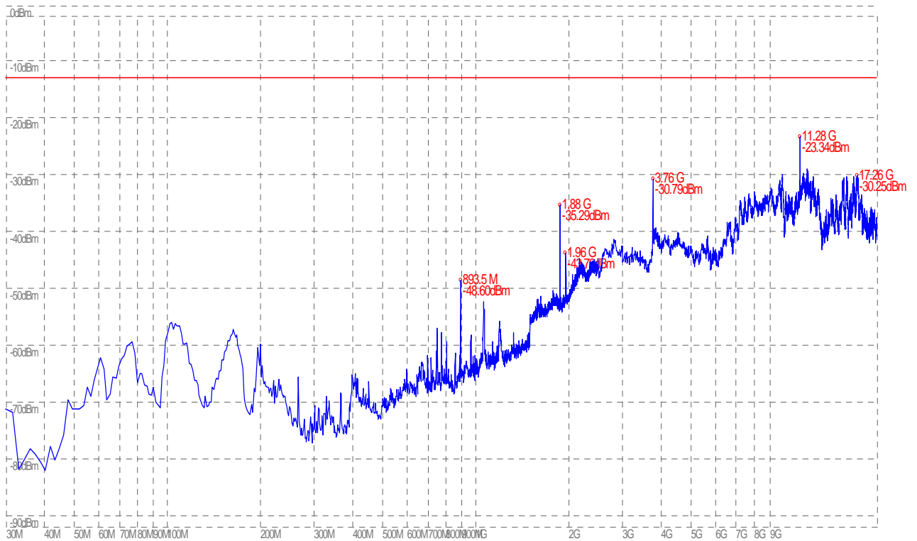
(Plot B.4: GSM 1900MHz Channel = 661, Test Antenna Vertical)
