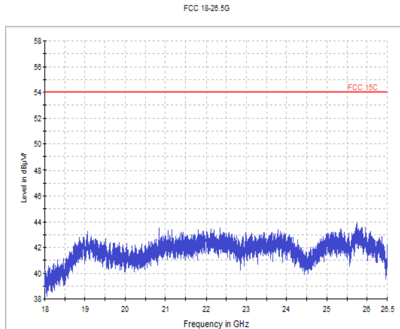
Fig.29. Radiated emission: GFSK, 18 GHz - 26 GHz
