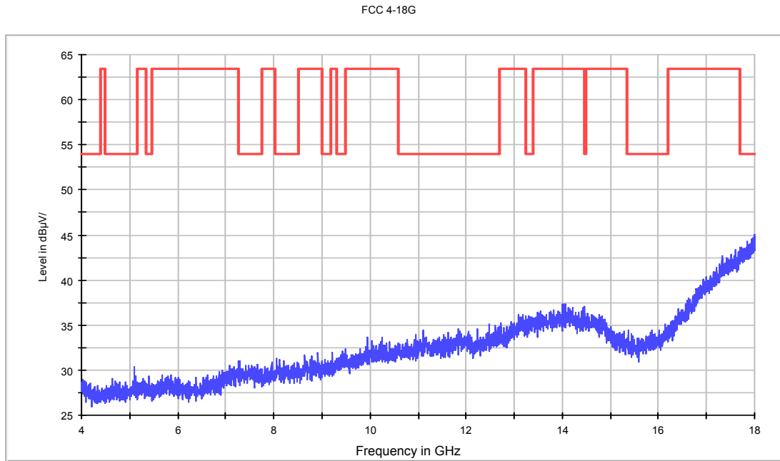
Fig.90. Radiated emission: 8DPSK, Channel 78, 4 GHz - 18 GHz
