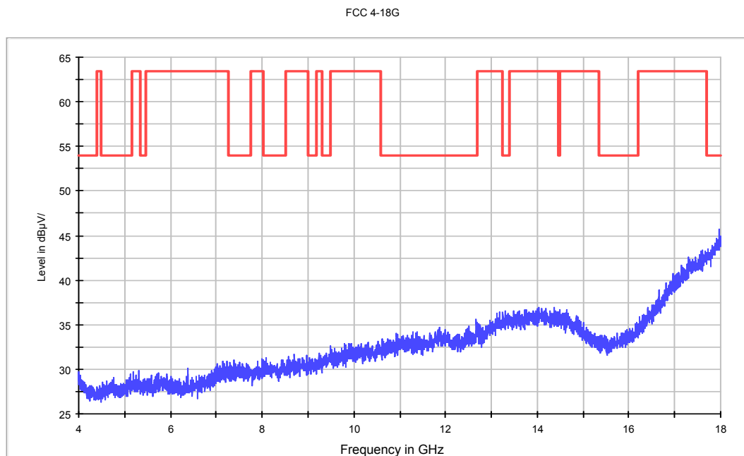
Fig.87. Radiated emission: 8DPSK, Channel 39, 4 GHz - 18 GHz
