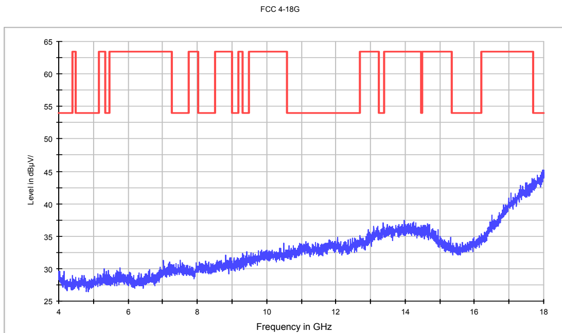
Fig.75. Radiated emission: \pi/4 DQPSK, Channel 39, 4 GHz - 18 GHz
