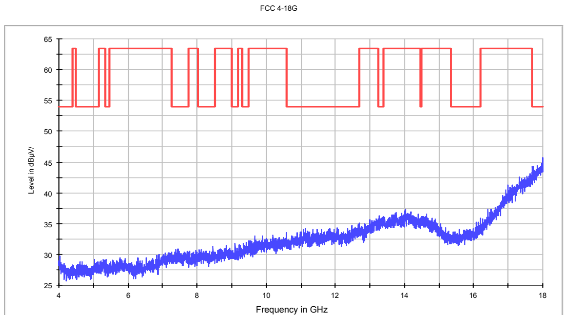
Fig.78. Radiated emission: \pi/4 DQPSK, Channel 78, 4 GHz - 18 GHz
