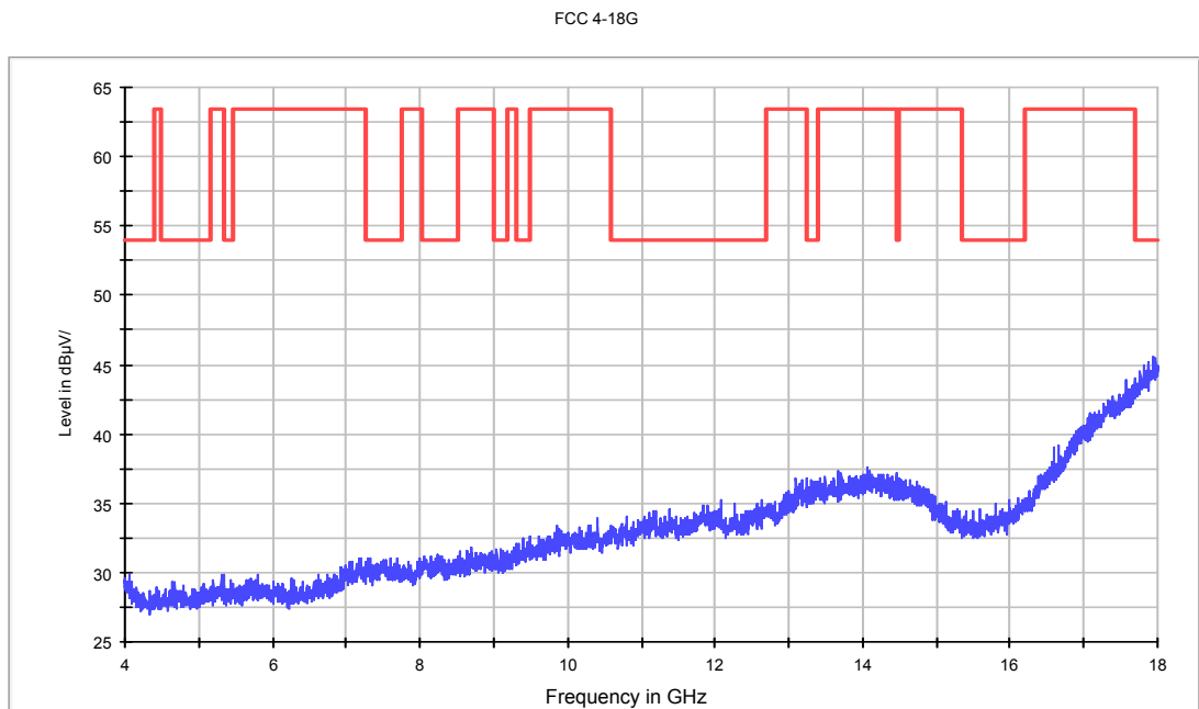
Fig.84. Radiated emission: 8DPSK, Channel 0, 4 GHz - 18 GHz
