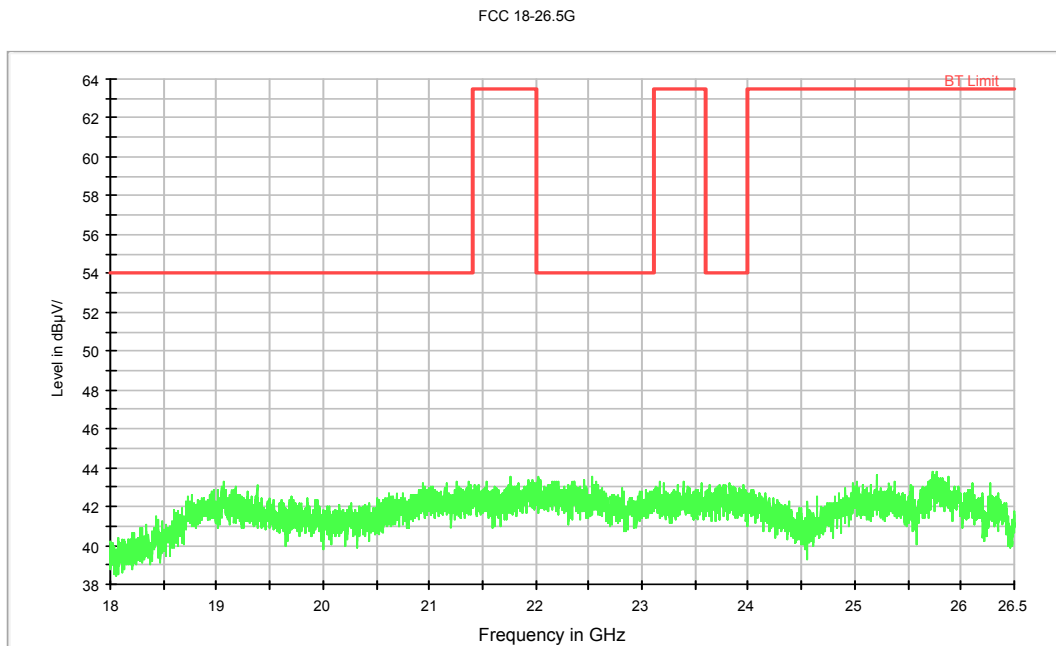
Fig.80. Radiated emission (Power): \pi/4 DQPSK, high channel
