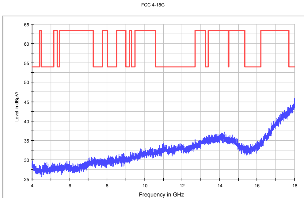
Fig.63. Radiated emission: GFSK, Channel 39, 4 GHz - 18 GHz
