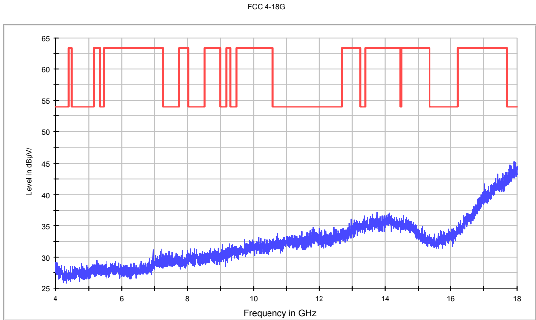
Fig.60. Radiated emission: GFSK, Channel 0, 4 GHz - 18 GHz
