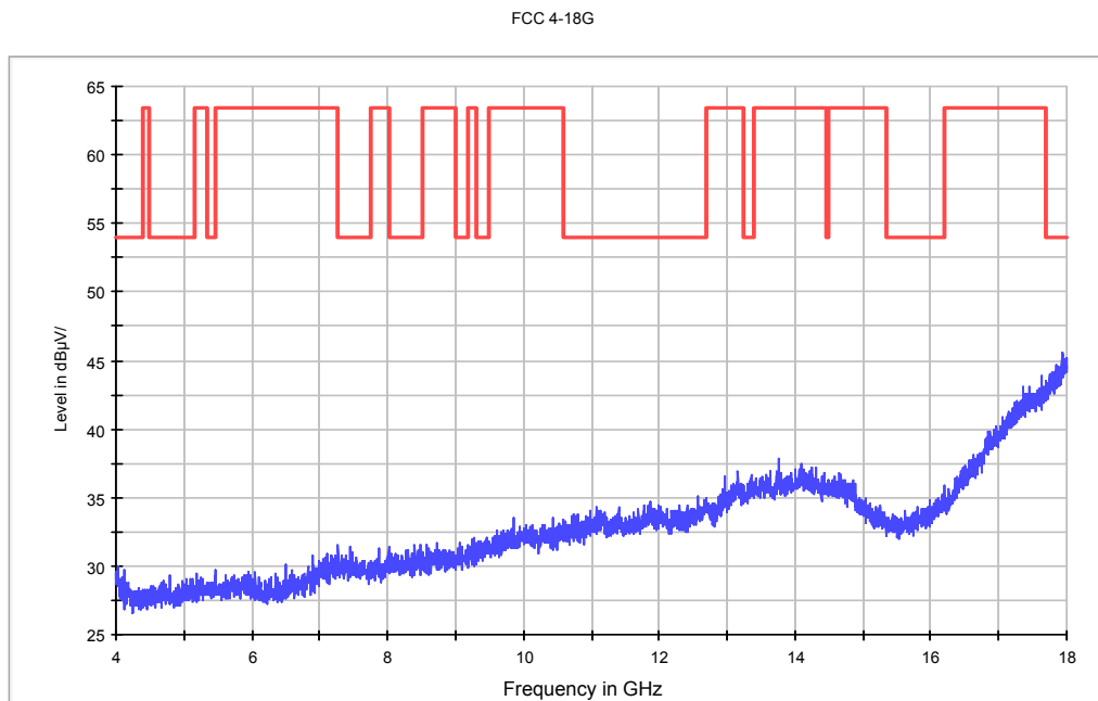
Fig.72. Radiated emission: \pi/4 DQPSK, Channel 0, 4 GHz - 18 GHz
