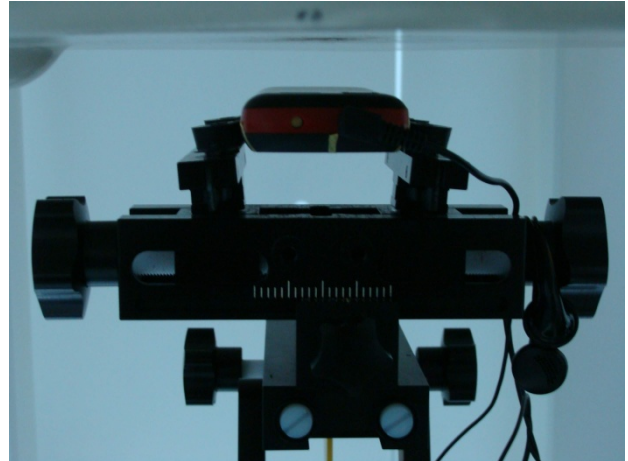
Back of the DUT with Phantom 1.5 cm Gap (with Headset)
