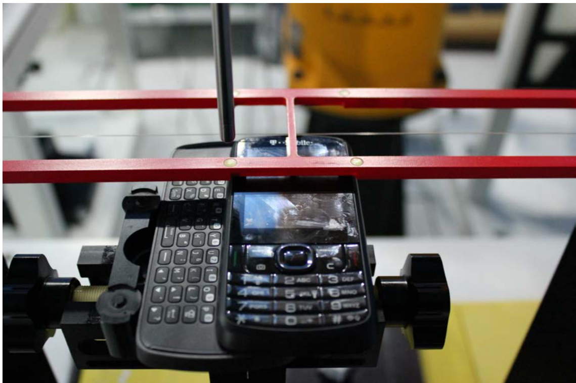
Picture 5: EUT Positioning for T-coil – Slide up
