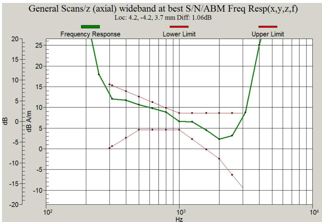
Figure C.4 Frequency Response of WCDMA 1700 – Slide down
