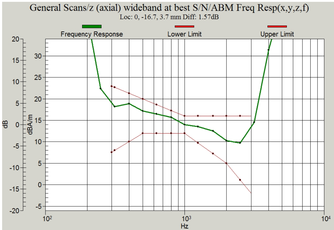
Figure C.1 Frequency Response of GSM 850 – Slide down
