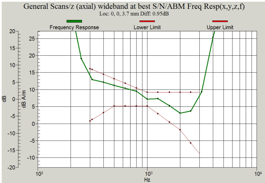
Figure C.9 Frequency Response of WCDMA 1700 – Slide up
