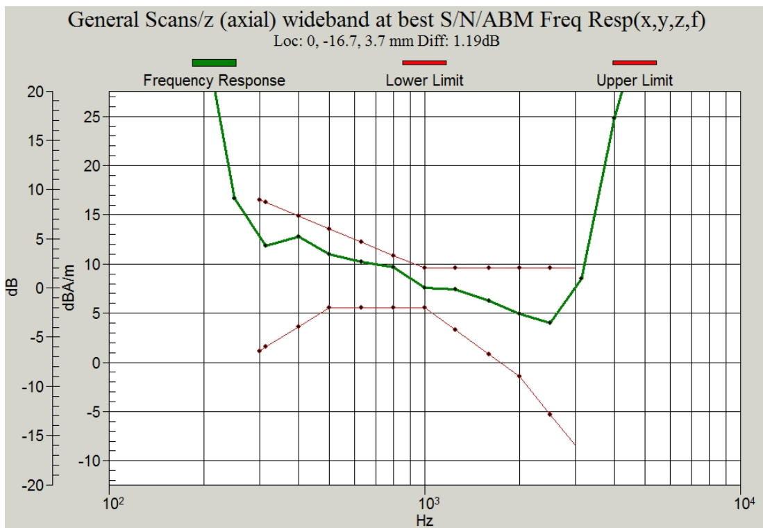
Figure C.2 Frequency Response of GSM 1900 – Slide down
