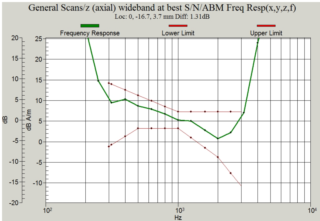
Figure C.3 Frequency Response of WCDMA 850 – Slide down
