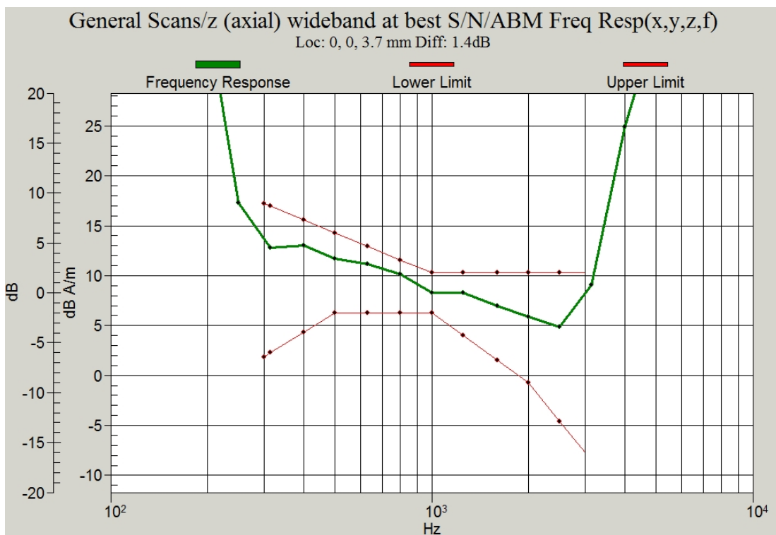
Figure C.6 Frequency Response of GSM 850 – Slide up
