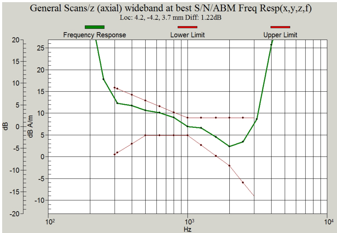
Figure C.5 Frequency Response of WCDMA 1900 – Slide down
