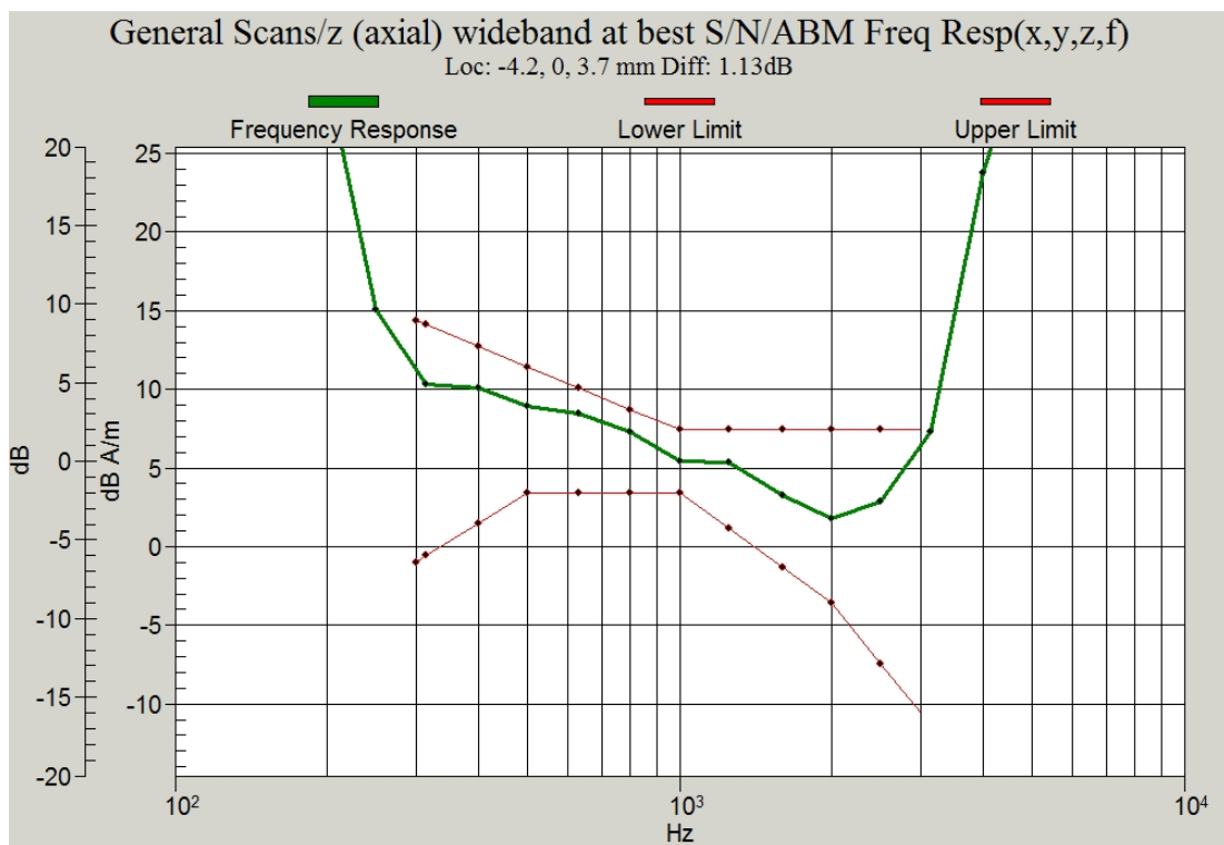
Figure C.8 Frequency Response of WCDMA 850 – Slide up
