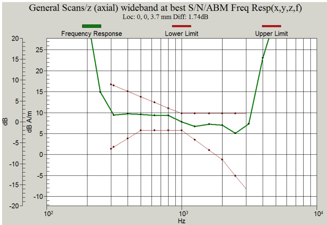
Figure C.7 Frequency Response of GSM 1900 – Slide up
