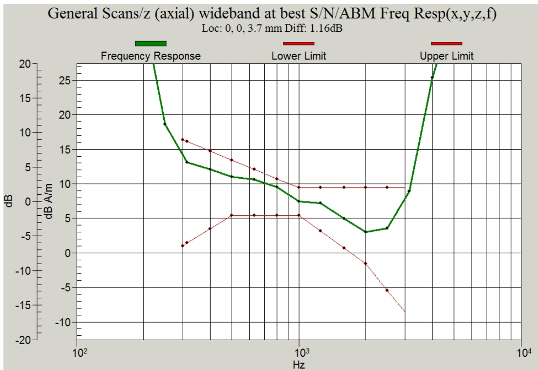
Figure C.10 Frequency Response of WCDMA 1900 – Slide up
