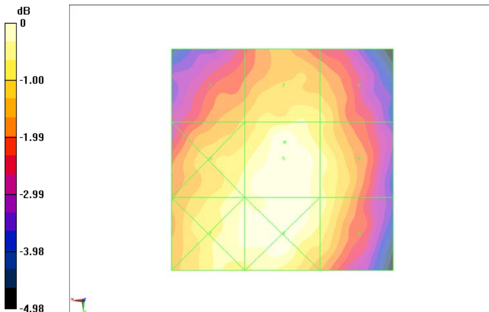
Fig B.36 HAC RF E-Field GSM 850 High
