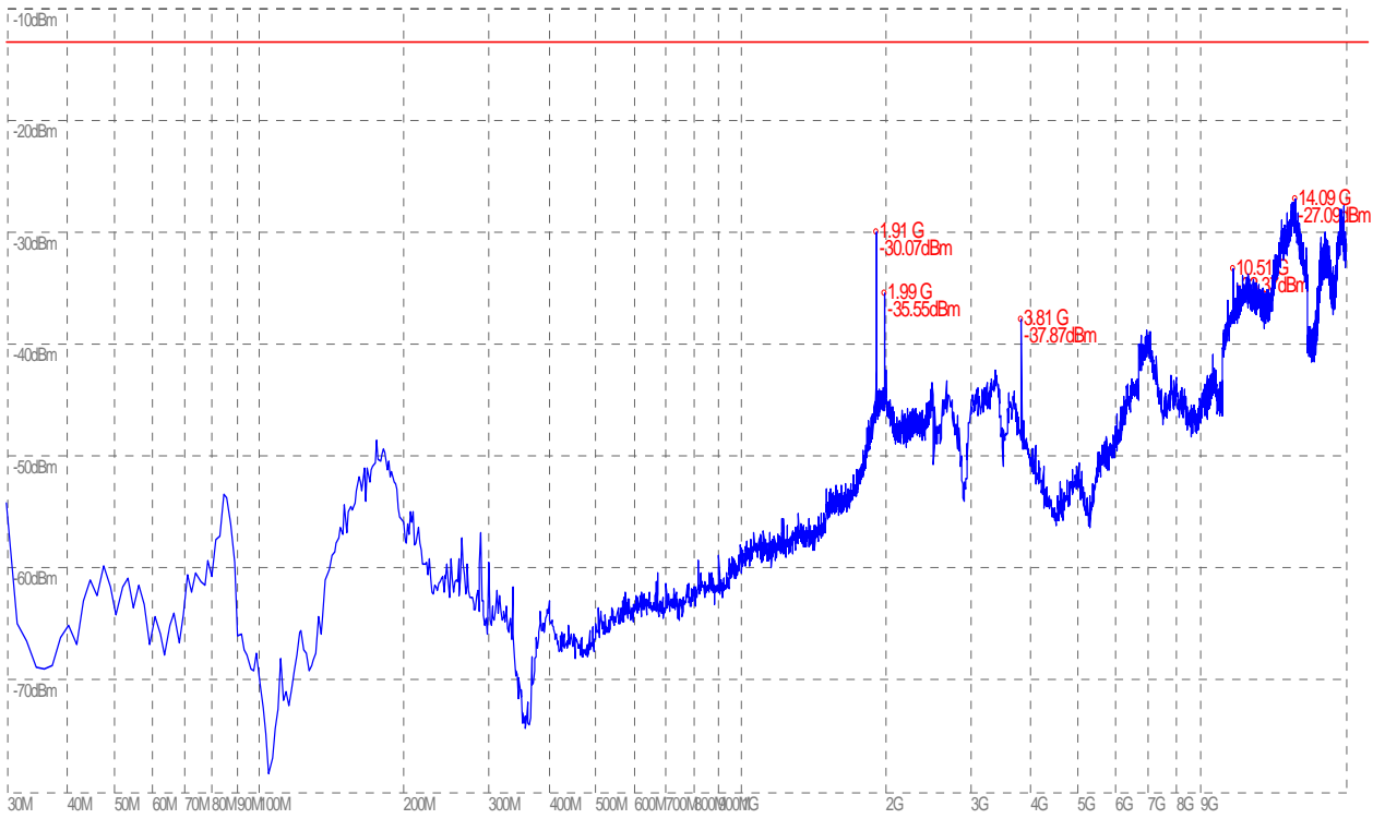
(Plot H.6: HSPA+ 1900 MHz Channel = 9938, Test Antenna Vertical)
