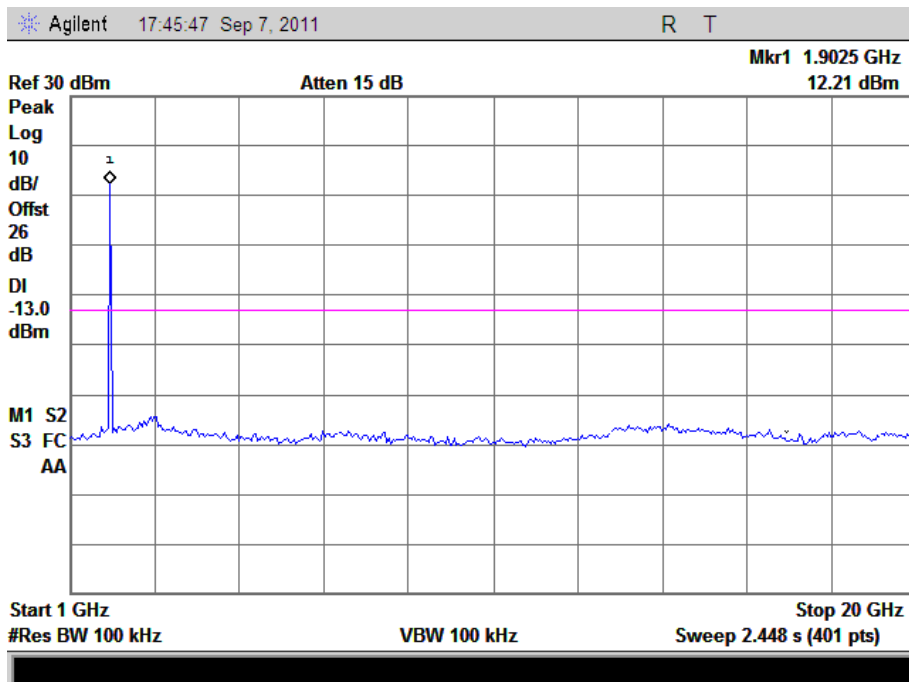
(Plot H3.1: HSPA+1900MHz Channel = 9938 1GHz to 20GHz)
