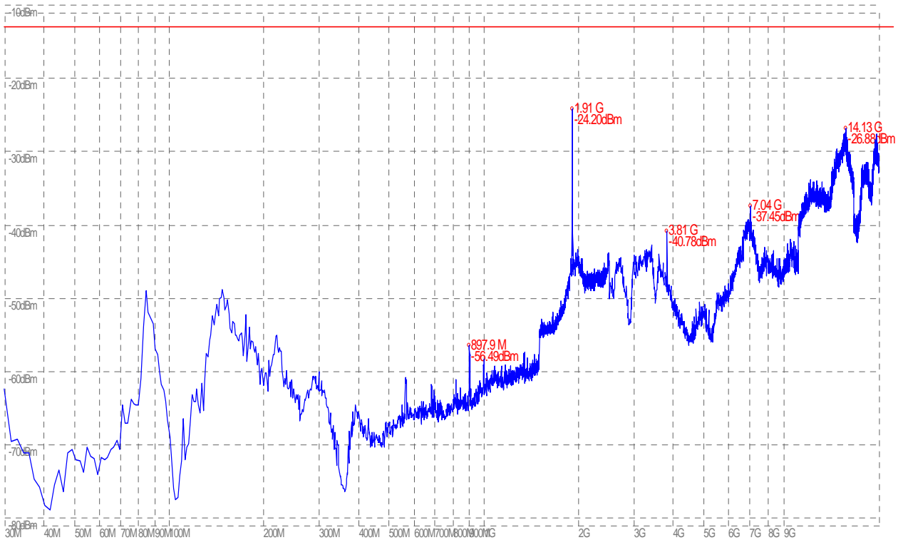
(Plot E.5: WCDMA 1900MHz Channel = 9938, Test Antenna Horizontal)
