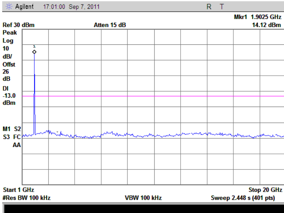
(Plot F3.1: HSDPA1900MHz Channel = 9938 1GHz to 20GHz)
