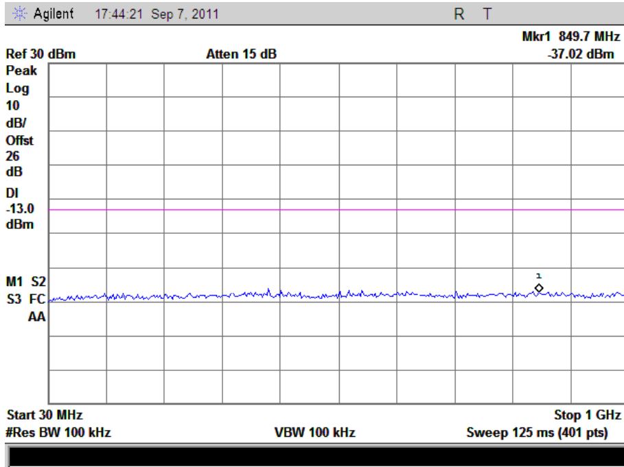
(Plot H1: HSPA+1900MHz Channel = 9662, 30MHz to 1GHz)
