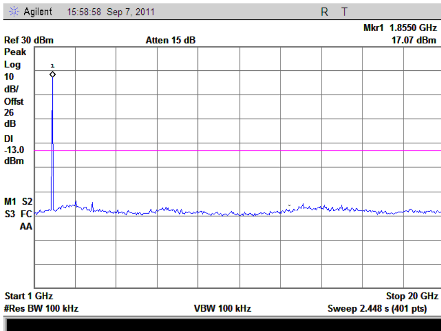
(Plot E1.1: WCDMA1900MHz Channel = 9662, 1GHz to 20GHz)
