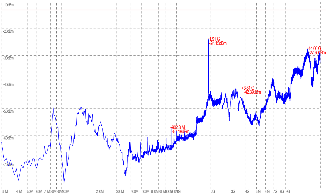
(Plot G.5: HSUPA 1900 MHz Channel = 9938, Test Antenna Horizontal)
