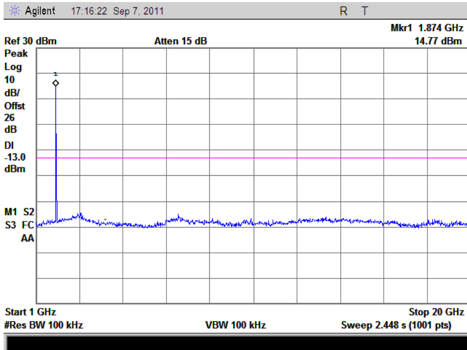
(Plot G2.1: HSUPA1900MHz Channel = 9800, 1GHz to 20GHz)
