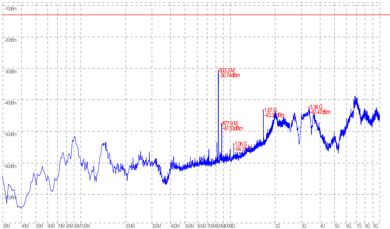
(Plot F.1: HSDPA 1900 MHz Channel = 9662, Test Antenna Horizontal)
