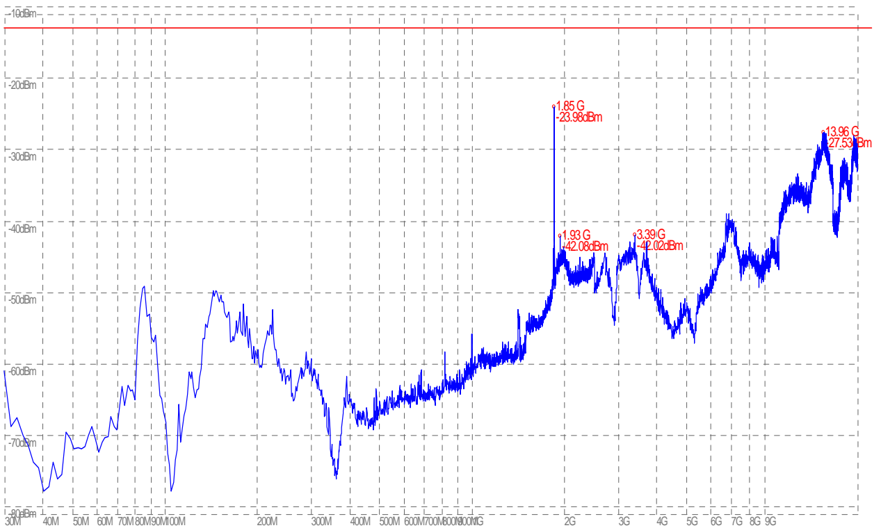
(Plot H.1: HSPA+ 1900 MHz Channel = 9662, Test Antenna Horizontal)
