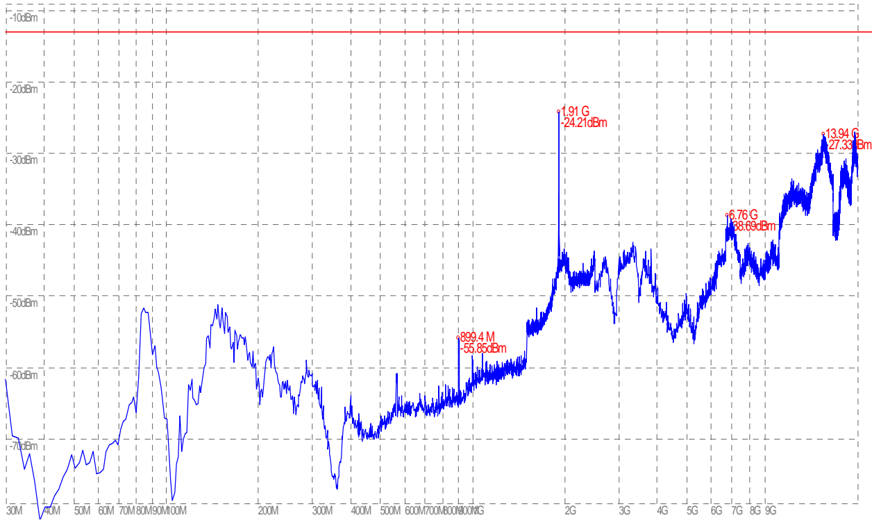
(Plot H.5: HSPA+ 1900 MHz Channel = 9938, Test Antenna Horizontal)
