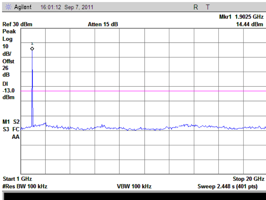
(Plot E3.1: WCDMA1900MHz Channel = 9938 1GHz to 20GHz)
