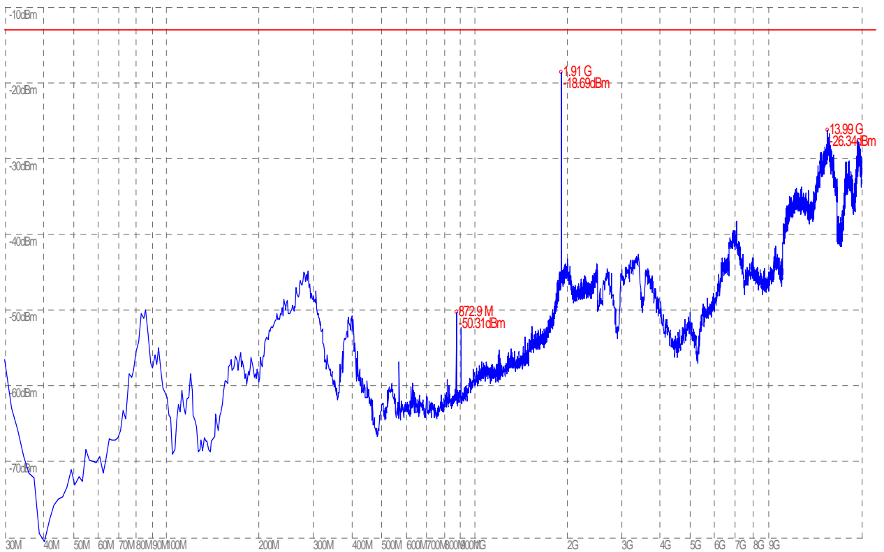
(Plot B.5: GSM 1900MHz Channel = 810, Test Antenna Horizontal)
