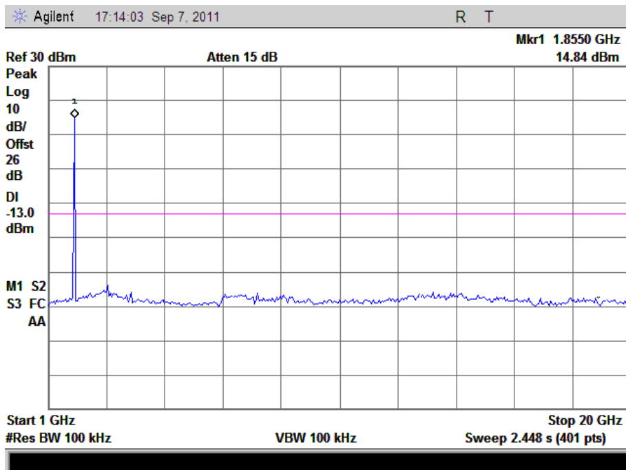
(Plot G1.1: HSUPA1900MHz Channel = 9662, 1GHz to 20GHz)
