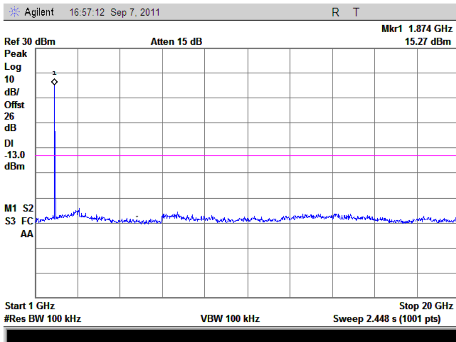
(Plot F2.1: HSDPA1900MHz Channel = 9800, 1GHz to 20GHz)
