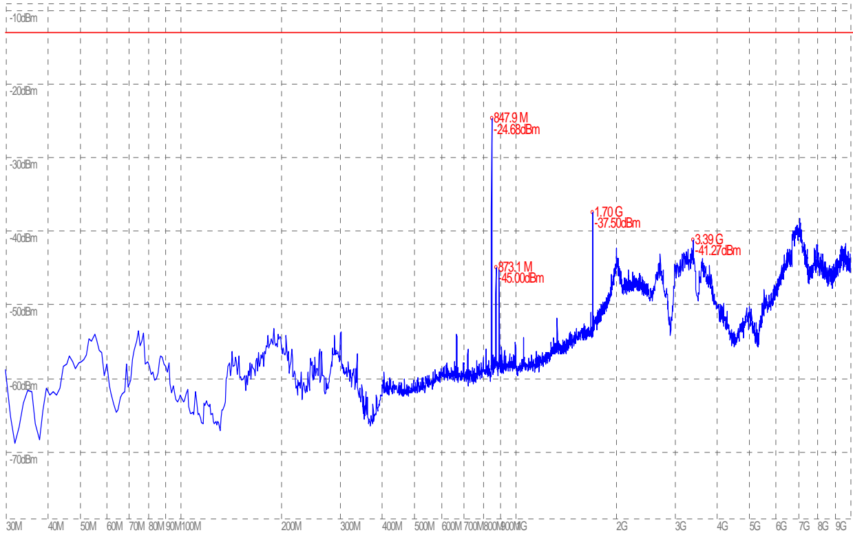
(Plot C.6: EGPRS 850MHz Channel = 251, Test Antenna Vertical)
