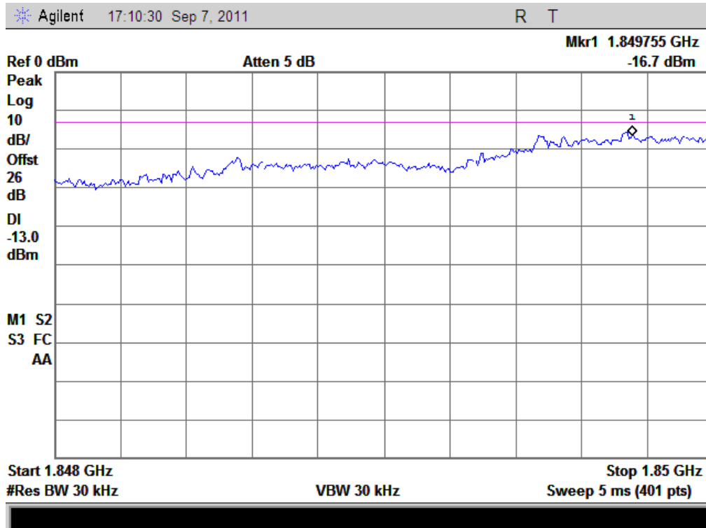
(Plot M: HSUPA 1900 Channel = 9662)
