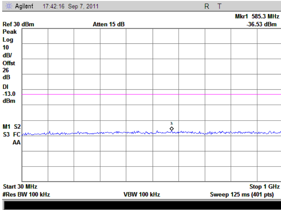
(Plot H2: HSPA+1900MHz Channel = 9800, 30MHz to 1GHz)
