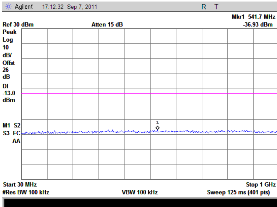
(Plot G 3: HSUPA1900MHz Channel = 9938, 30MHz to 1GHz)
