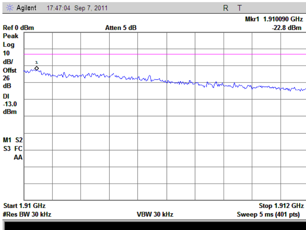
(Plot P: HSPA +1900 Channel = 9938)
