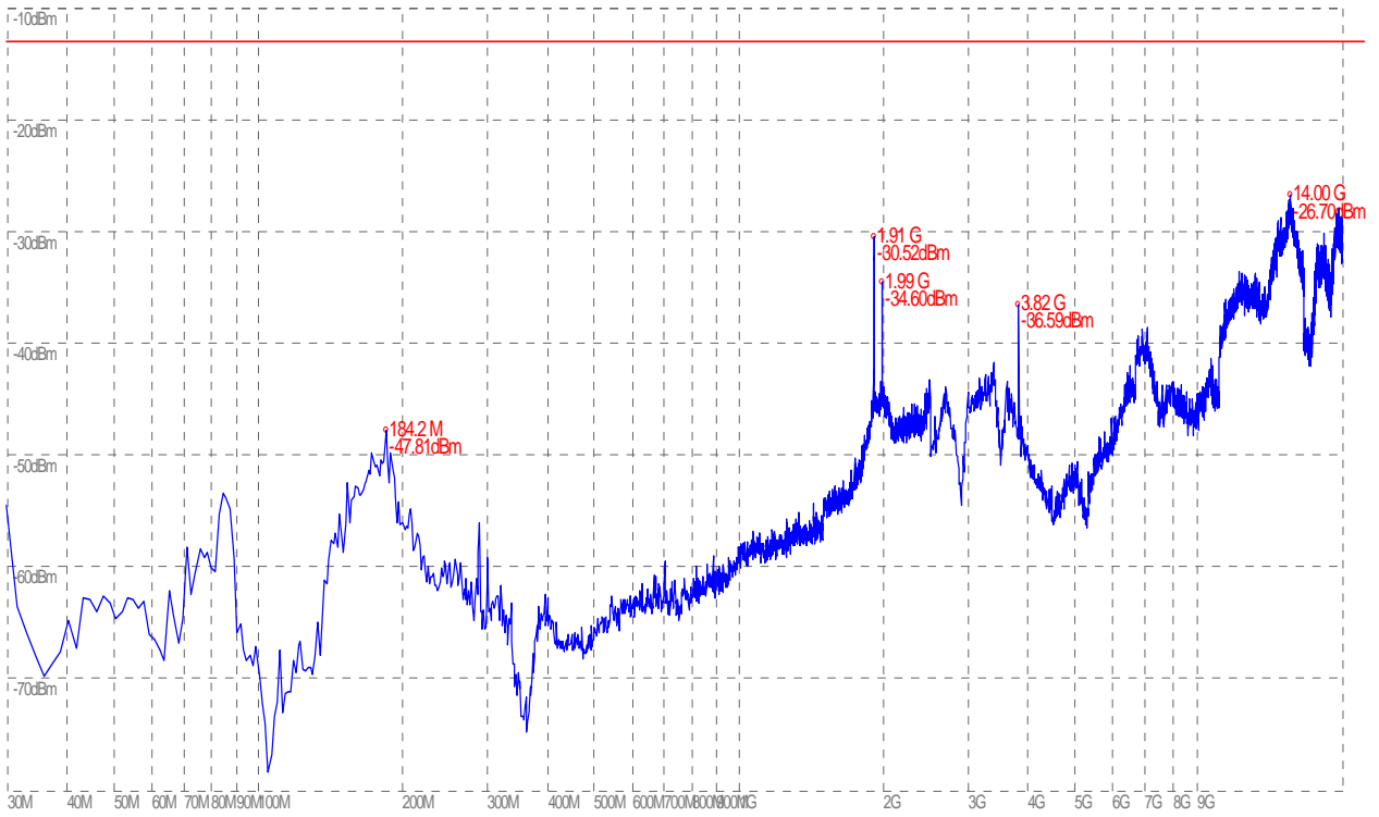
(Plot G.6: HSUPA 1900 MHz Channel = 9938, Test Antenna Vertical)
