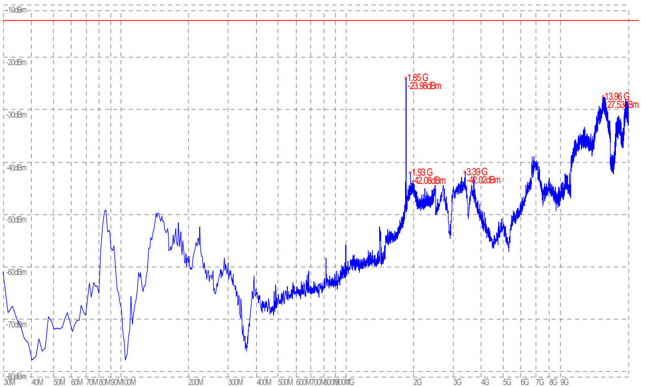
(Plot G.1: HSUPA 1900 MHz Channel = 9662, Test Antenna Horizontal)
