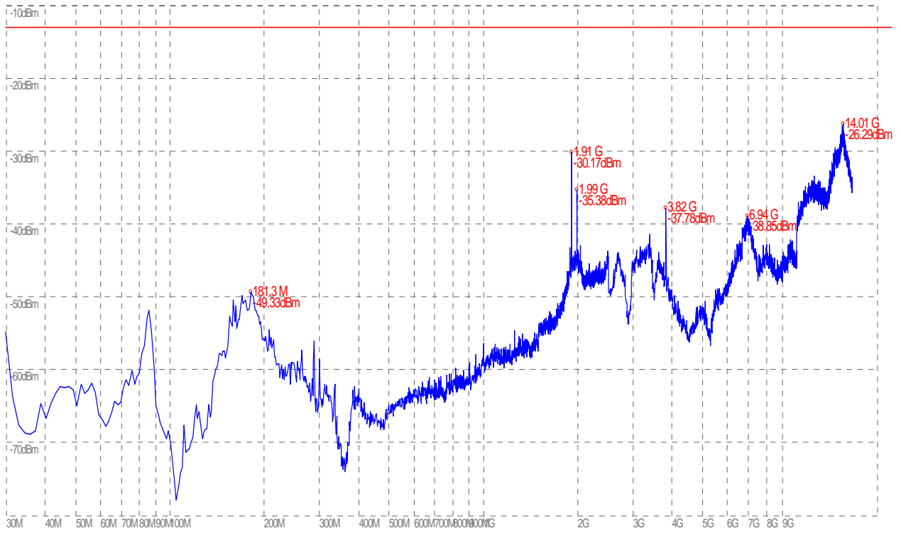
(Plot E.6: WCDMA 1900MHz Channel = 9938, Test Antenna Vertical)
