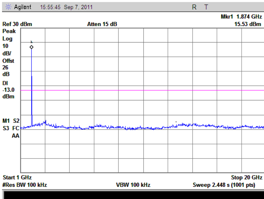
(Plot E2.1: WCDMA1900MHz Channel = 9800, 1GHz to 20GHz)
