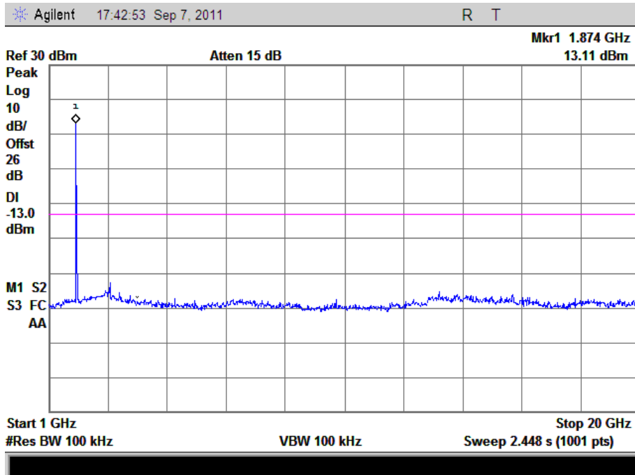
(Plot H2.1: HSPA+1900MHz Channel = 9800, 1GHz to 20GHz)
