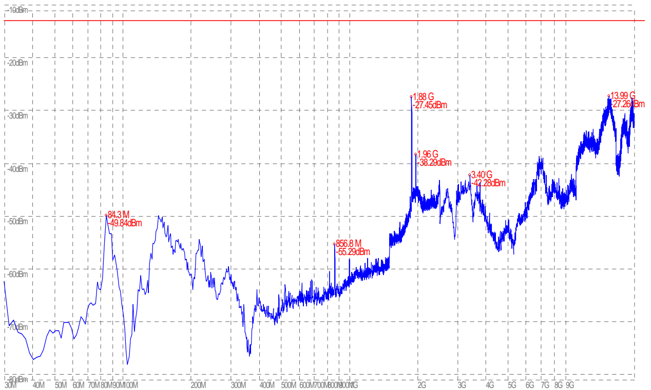
(Plot G.3: HSUPA 1900 MHz Channel = 9800, Test Antenna Horizontal)
