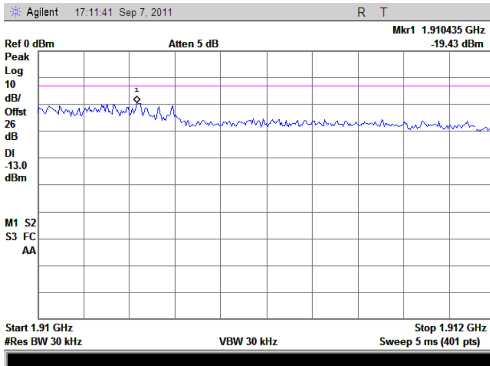
(Plot N: HSUPA 1900 Channel = 9938)
