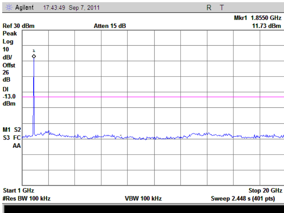
(Plot H1.1: HSPA+1900MHz Channel = 9662, 1GHz to 20GHz)
