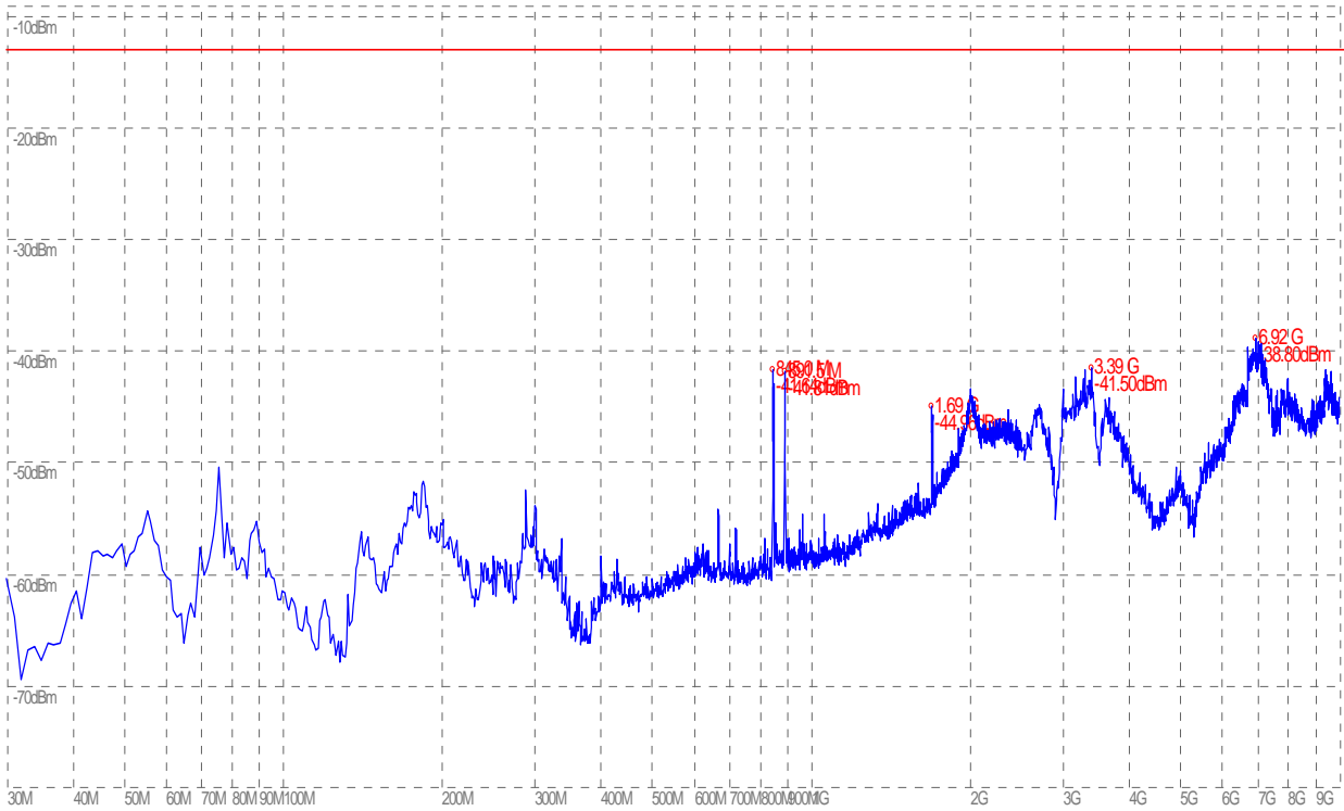
(Plot F.6: HSDPA 1900 MHz Channel = 9938, Test Antenna Vertical)
