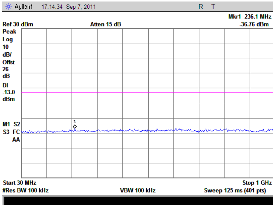
(Plot G 1: HSUPA1900MHz Channel = 9662, 30MHz to 1GHz)
