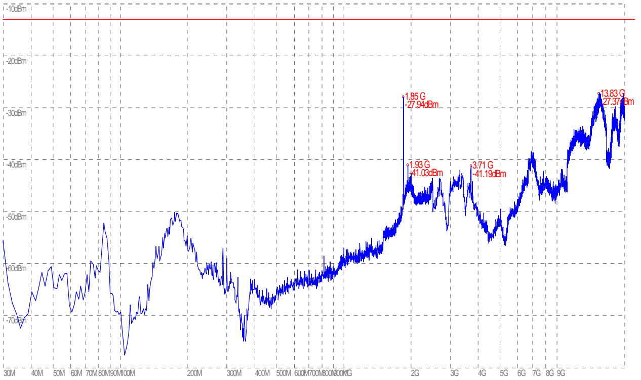
(Plot H.2: HSPA+ 1900 MHz Channel = 9662, Test Antenna Vertical)
