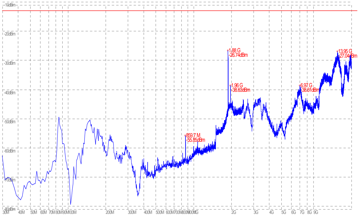
(Plot E.3: WCDMA 1900MHz Channel = 9800, Test Antenna Horizontal)
