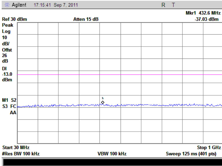
(Plot G2: HSUPA1900MHz Channel = 9800, 30MHz to 1GHz)
