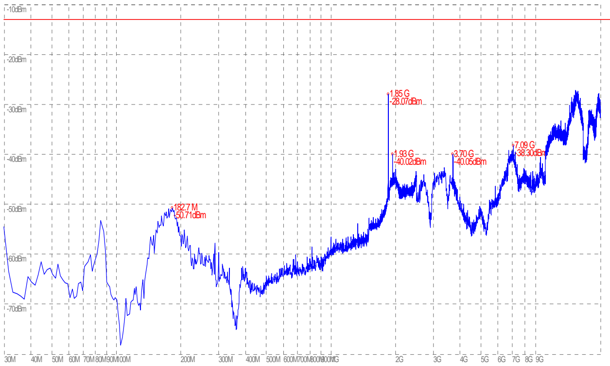
(Plot G.2: HSUPA 1900 MHz Channel = 9662, Test Antenna Vertical)
