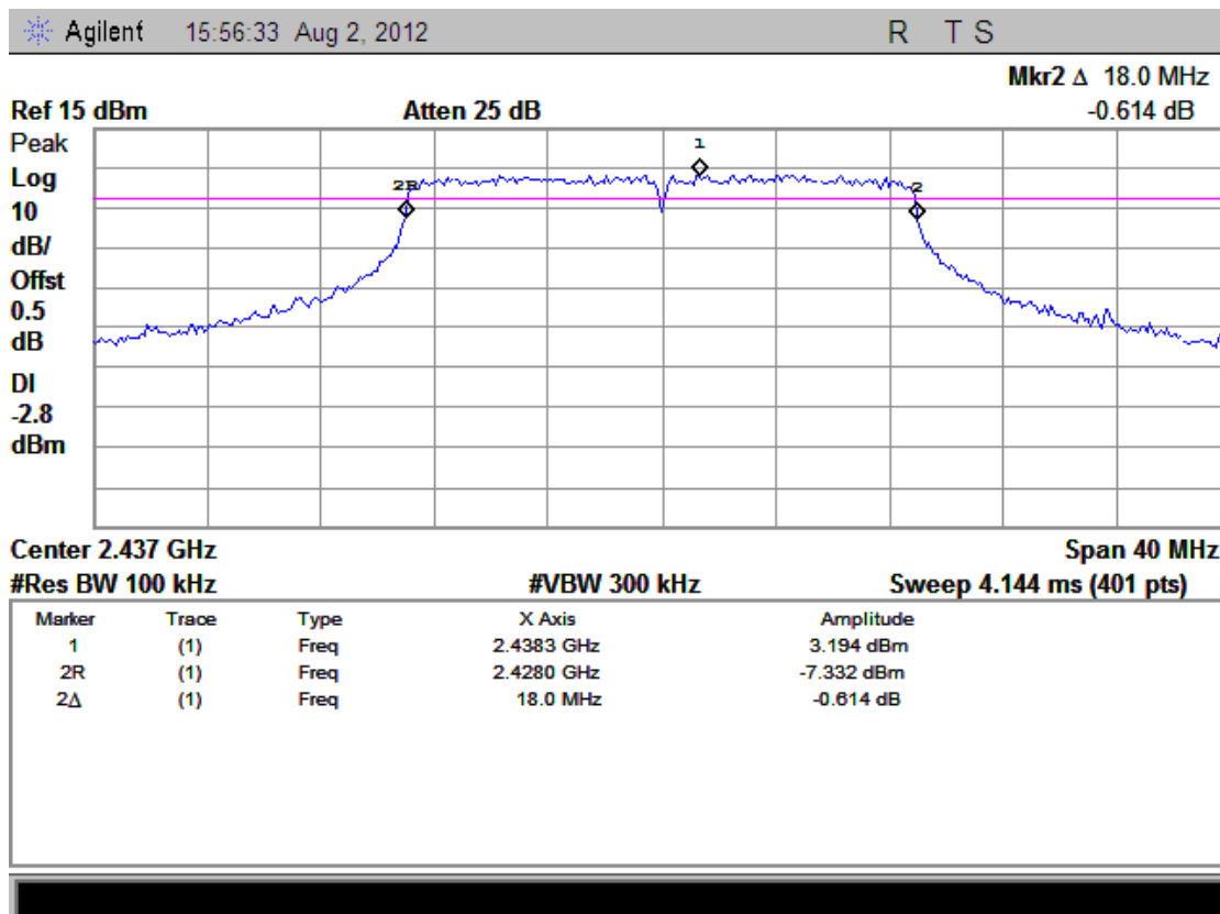
(Plot H: Channel 6: 2437MHz @ 802.11g)
