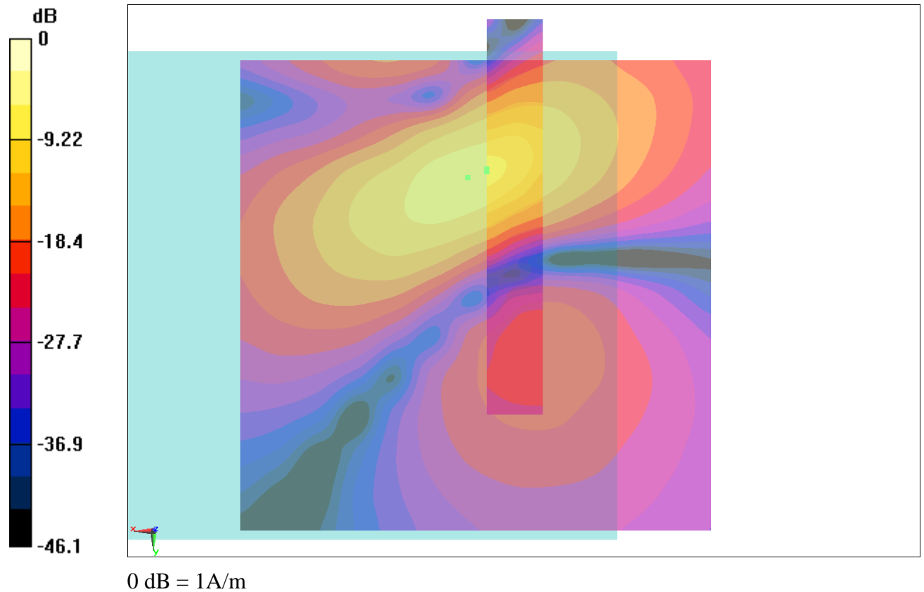
Fig B.5 T-Coil GSM 1900
