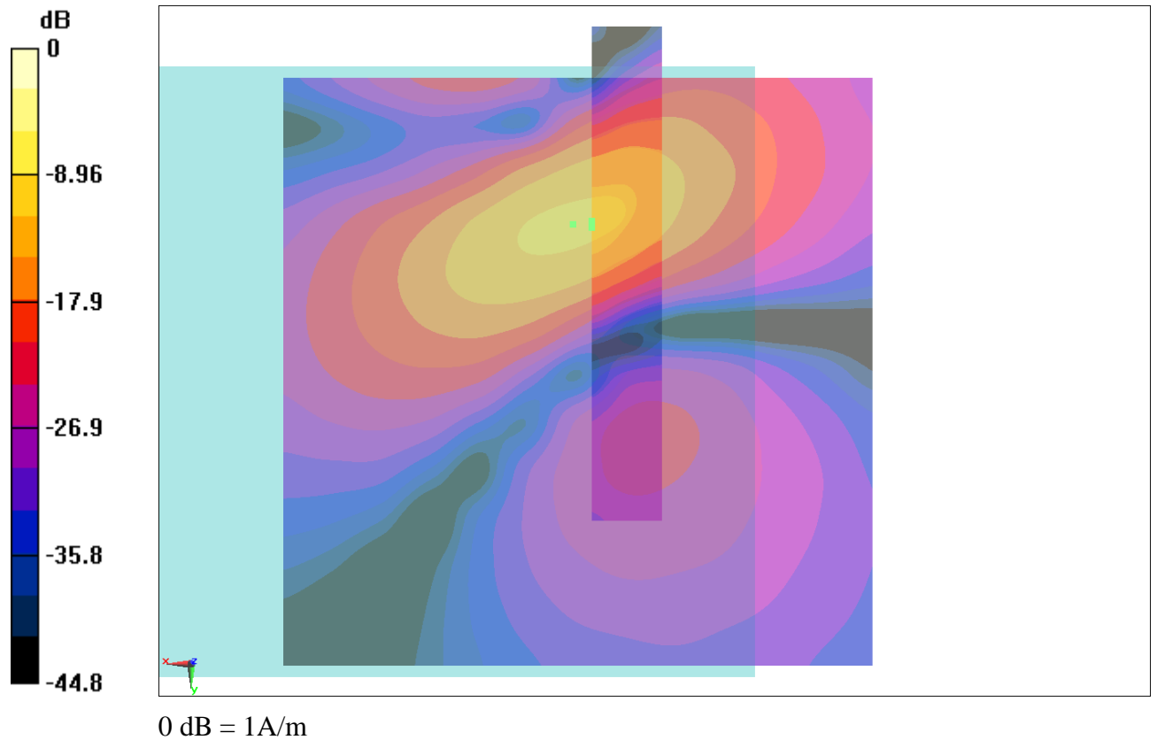
Fig B.2 T-Coil GSM 850
