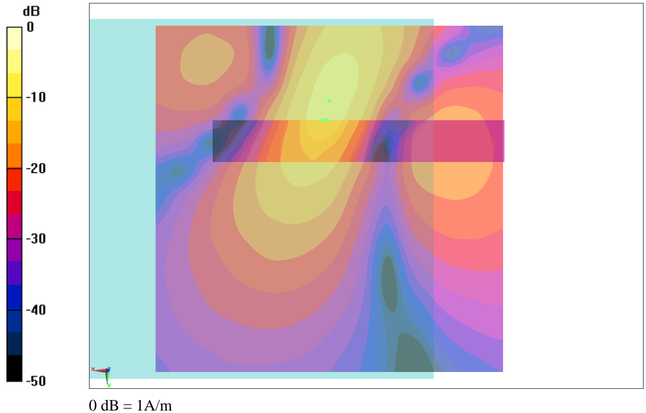
Fig B.4 T-Coil GSM 1900
