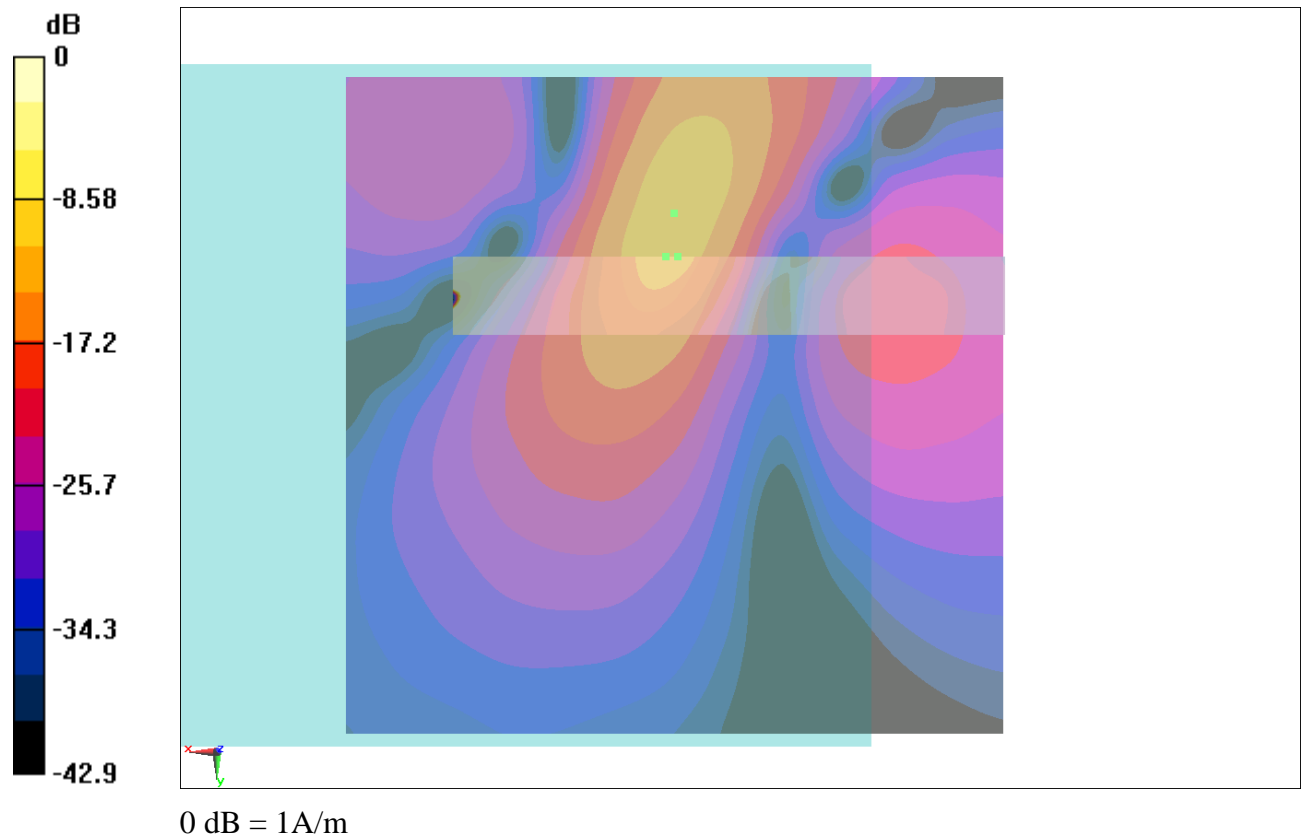
Fig B.1 T-Coil GSM 850
