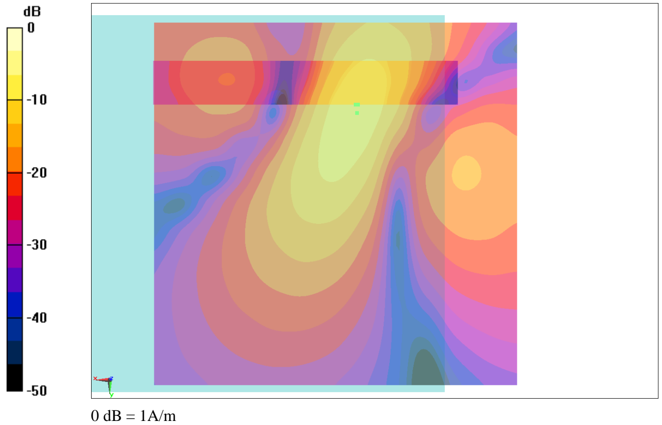
Fig B.10 T-Coil WCDMA 1700
