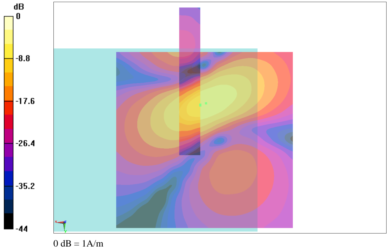
Fig B.14 T-Coil WCDMA 1900
