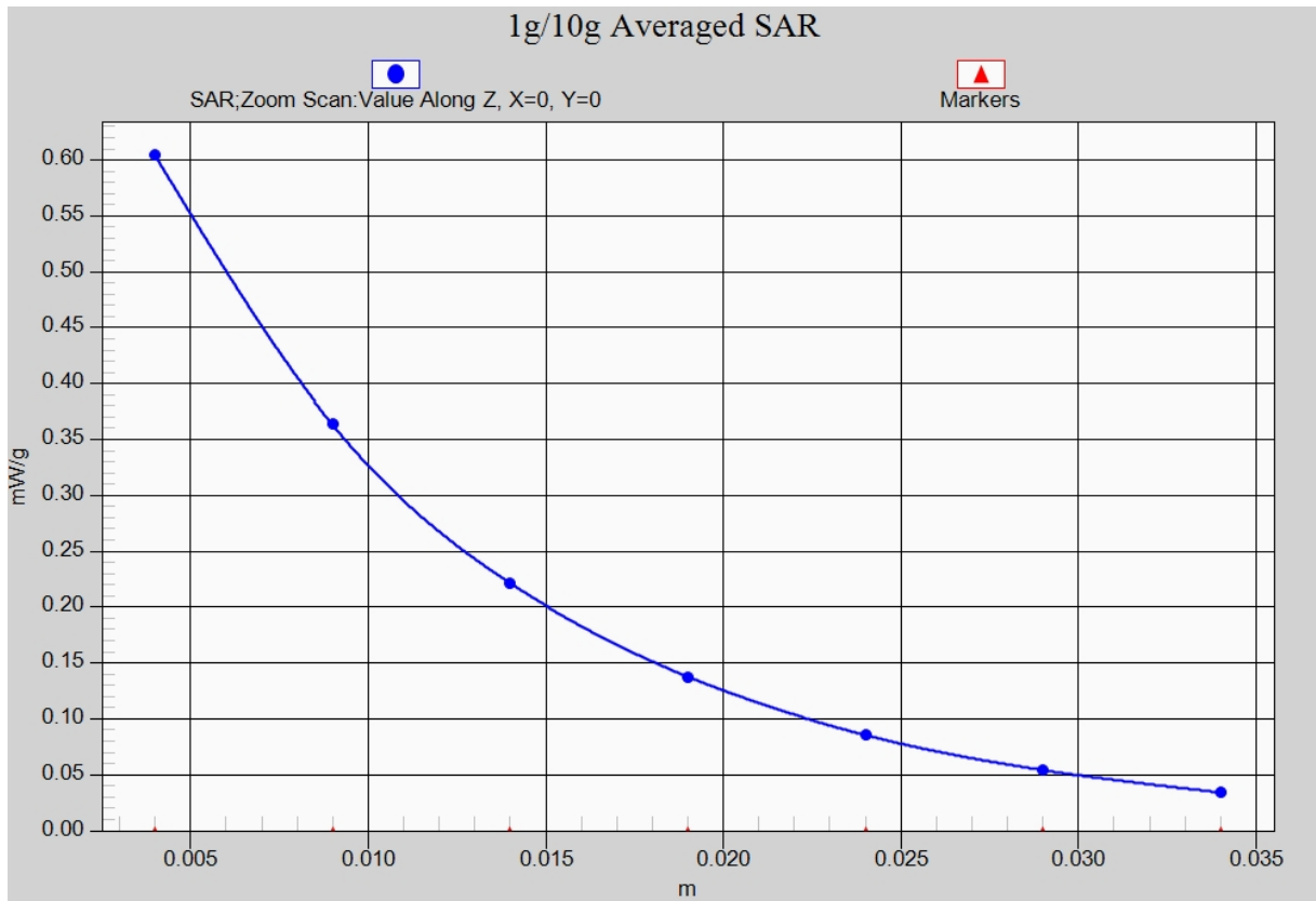
Fig. 24-1 Z-Scan at power reference point (1750 MHz CH450)
