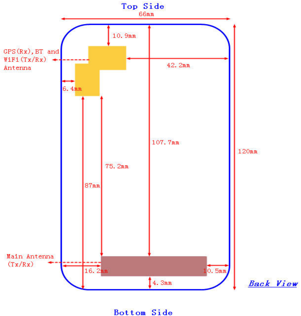
Picture 13.1 Antenna Locations
