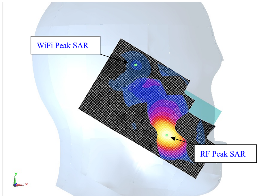
Picture 13.2 Combined for CDMA1700 and WiFi
