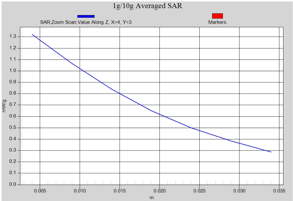
Fig. 8-1 Z-Scan at power reference point (850 MHz CH384)
