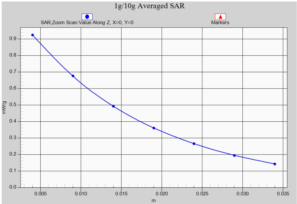
Fig. 18-1 Z-Scan at power reference point (850 MHz CH1013)
