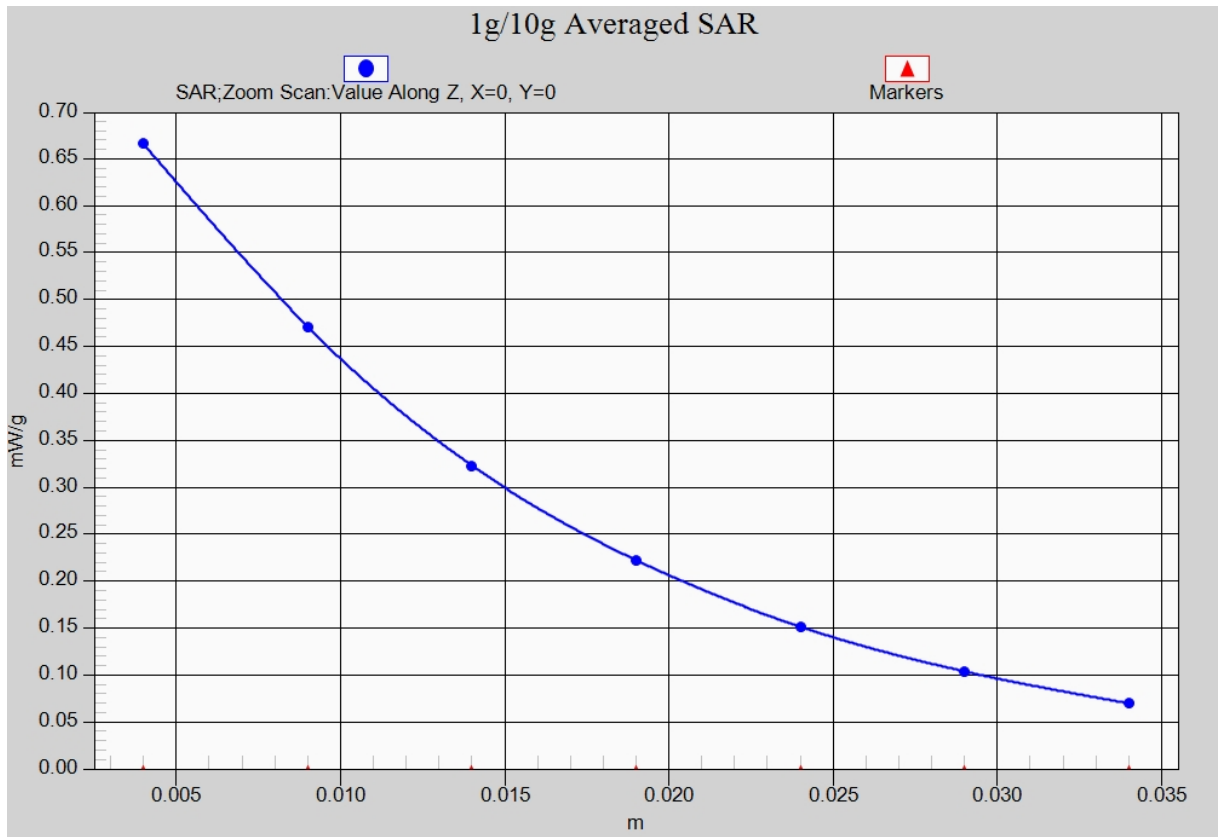
Fig. 37-1 Z-Scan at power reference point (1750 MHz CH450)
