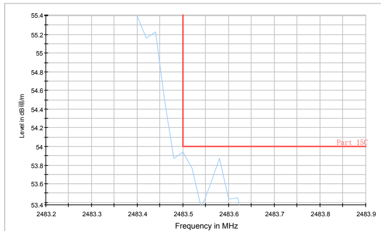
Fig.68. Radiated emission (Power) GFSK, high channel
