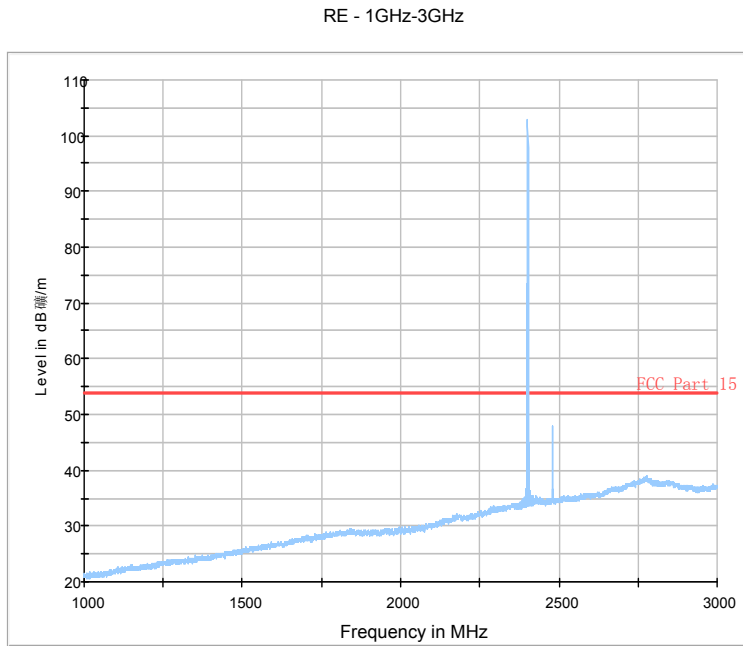
Fig.71. Radiated emission: \pi/4 DQPSK, Channel 0, 1 GHz - 3 GHz
