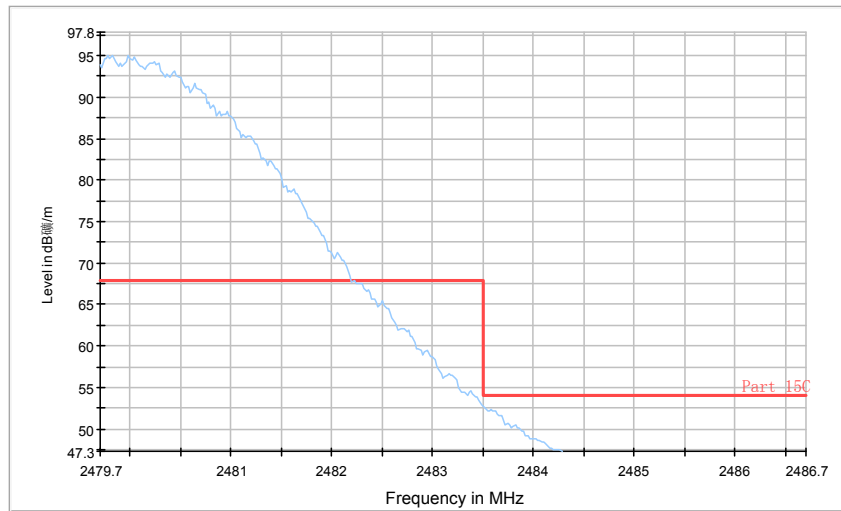
Fig.80. Radiated emission (Power): \pi/4 DQPSK, high channel
