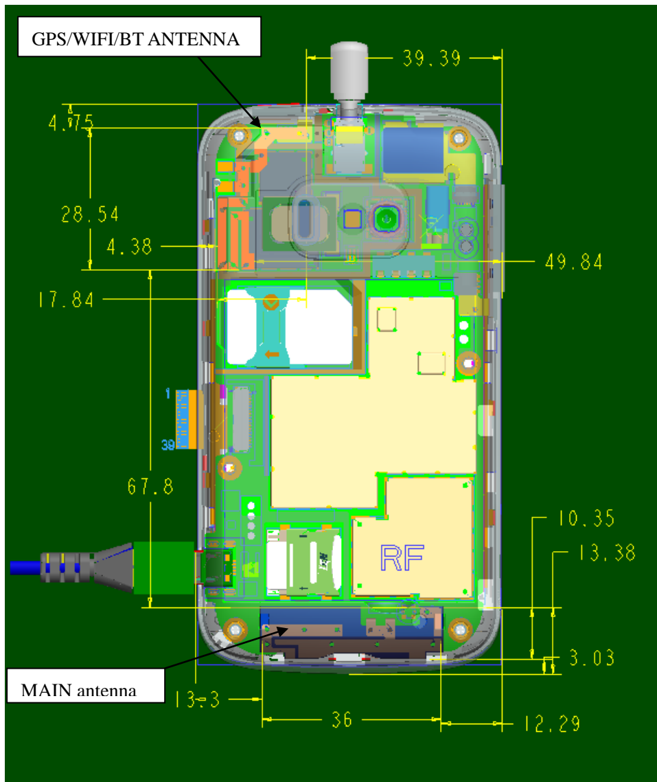
Picture 13.1 Antenna Locations
