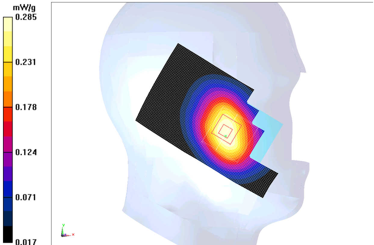
Fig. 3 850 MHz CH128
