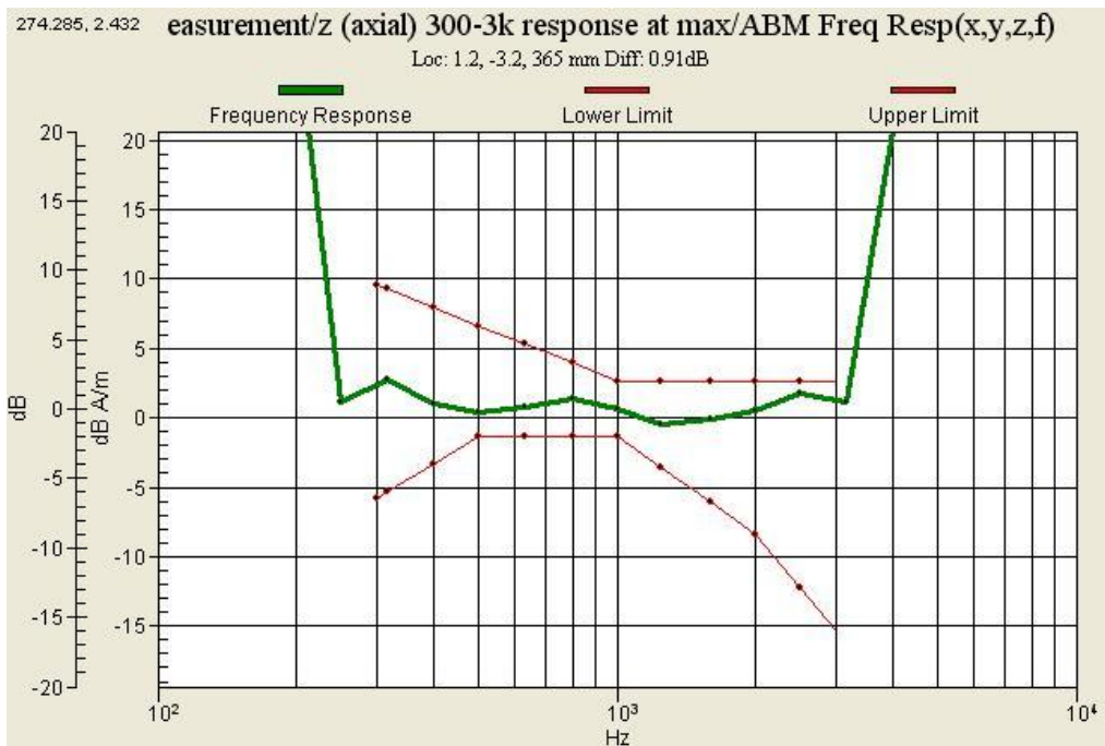
Graph 8 : AWS 1700 (CH 450) Frequency Response
