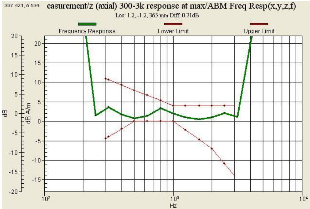
Graph 7 : AWS 1700 (CH 25) Frequency Response
