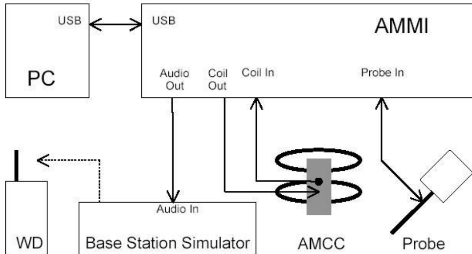
Figure 2: T-Coil setup cabling.
