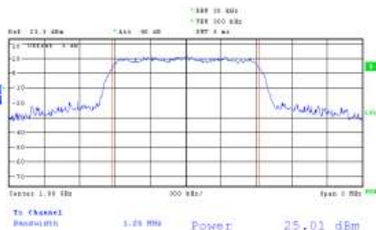
Figure. 8 Wireless Device Modulated Signal
