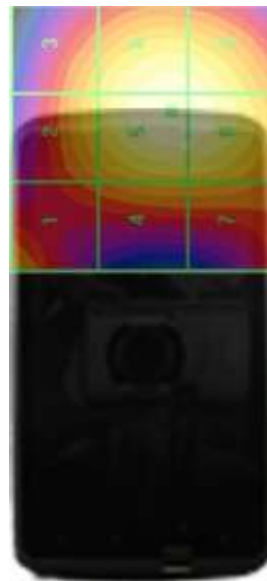
H-Field PCS Scan overlay
