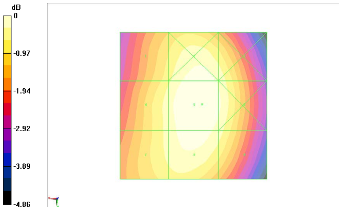
Fig B.7 HAC RF E-Field WCDMA 850 High
