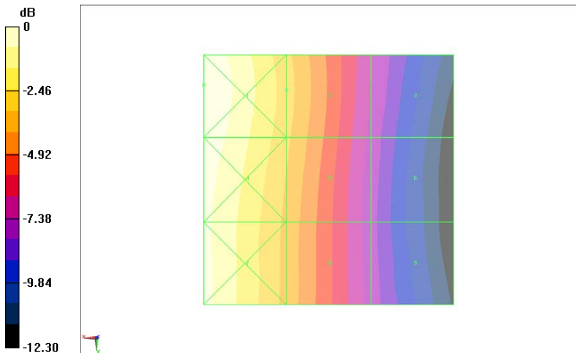
Fig B.21 HAC RF H-Field WCDMA 850 Low
