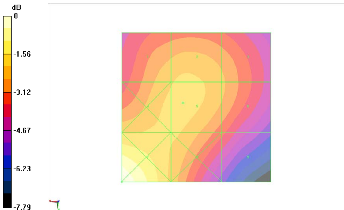
Fig B.22 HAC RF H-Field WCDMA 1900 High
