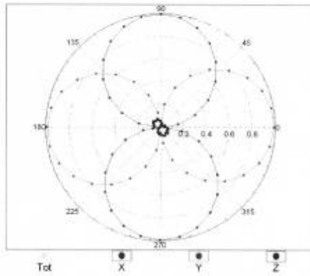
f=600 MHz,TEM,0°
