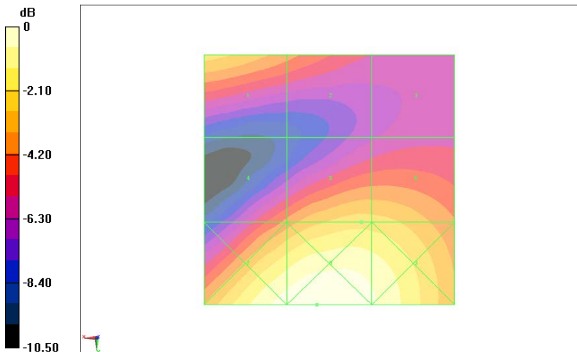
Fig B.12 HAC RF E-Field WCDMA 1900 Low
