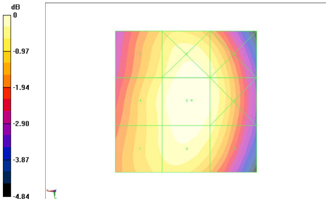
Fig B.8 HAC RF E-Field WCDMA 850 Middle
