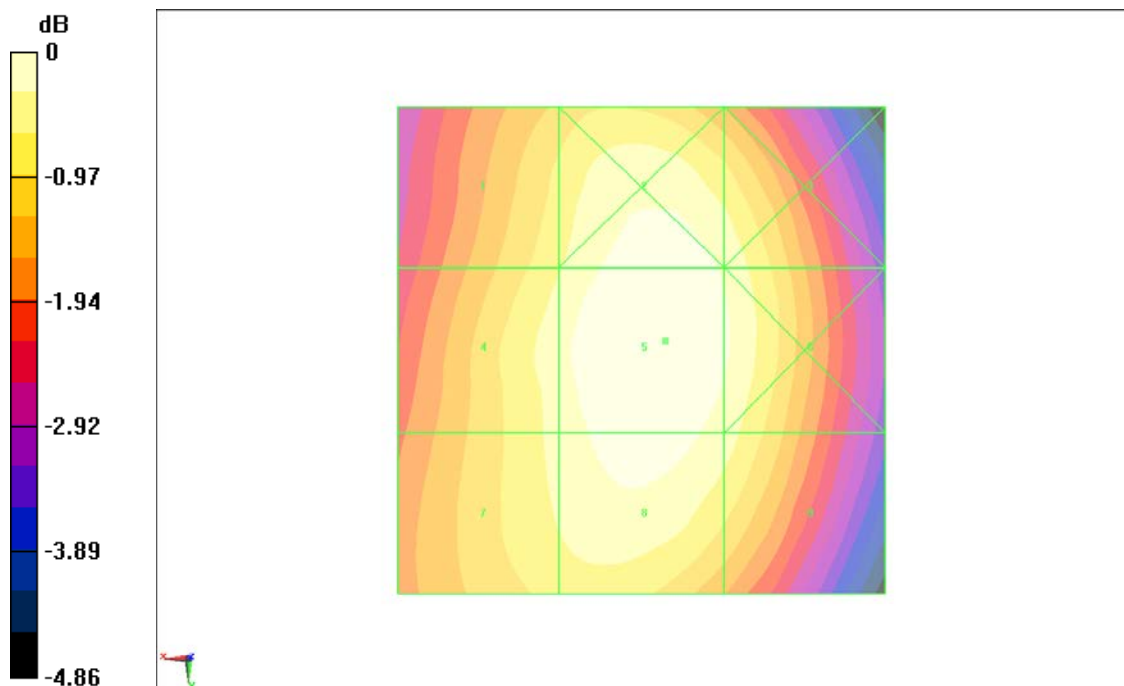
Fig B.9 HAC RF E-Field WCDMA 850 Low
