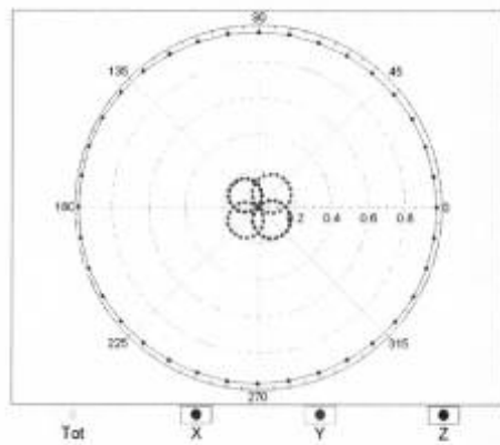
f=2500 MHz,R22,90°
