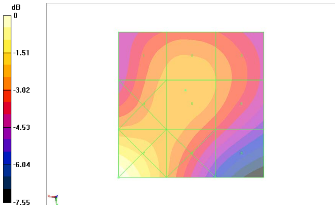
Fig B.23 HAC RF H-Field WCDMA 1900 Middle
