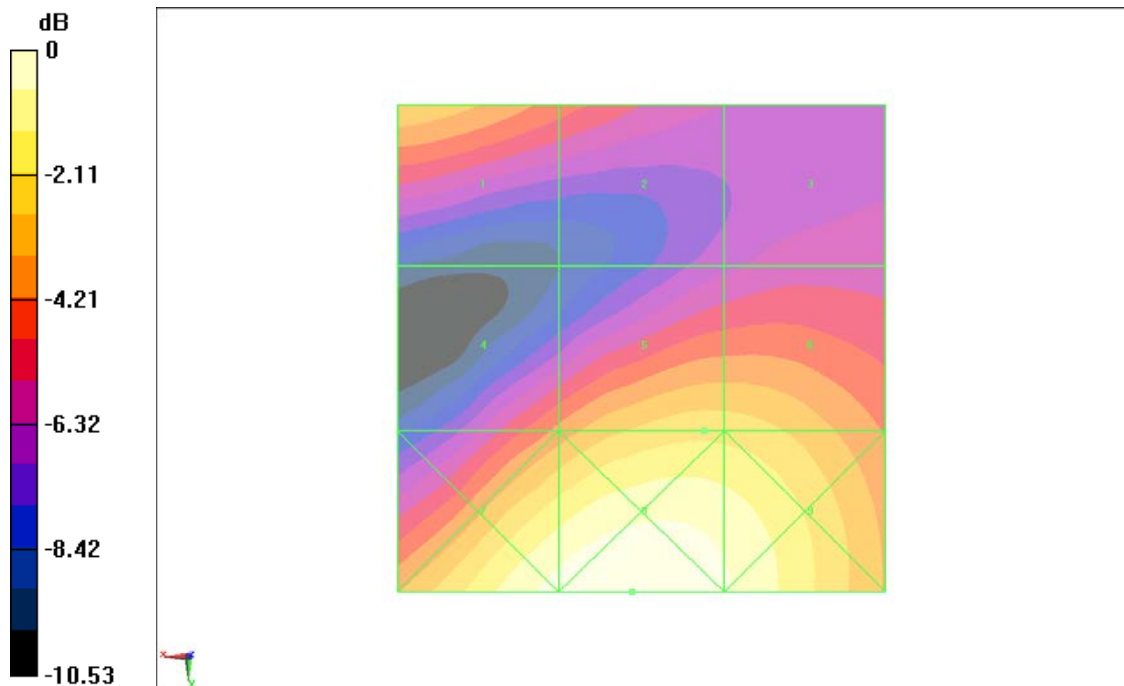
Fig B.11 HAC RF E-Field WCDMA 1900 Middle
