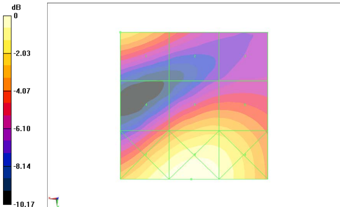
Fig B.10 HAC RF E-Field WCDMA 1900 High
