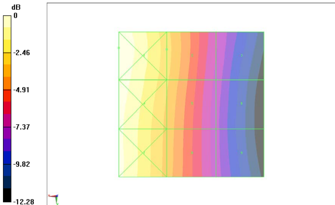
Fig B.19 HAC RF H-Field WCDMA 850 High
