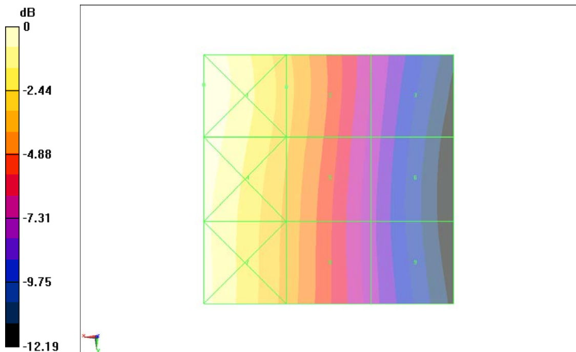
Fig B.20 HAC RF H-Field WCDMA 850 Middle
