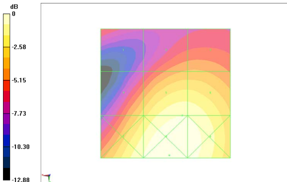
Fig B.20 HAC RF E-Field GSM 1900 Low
