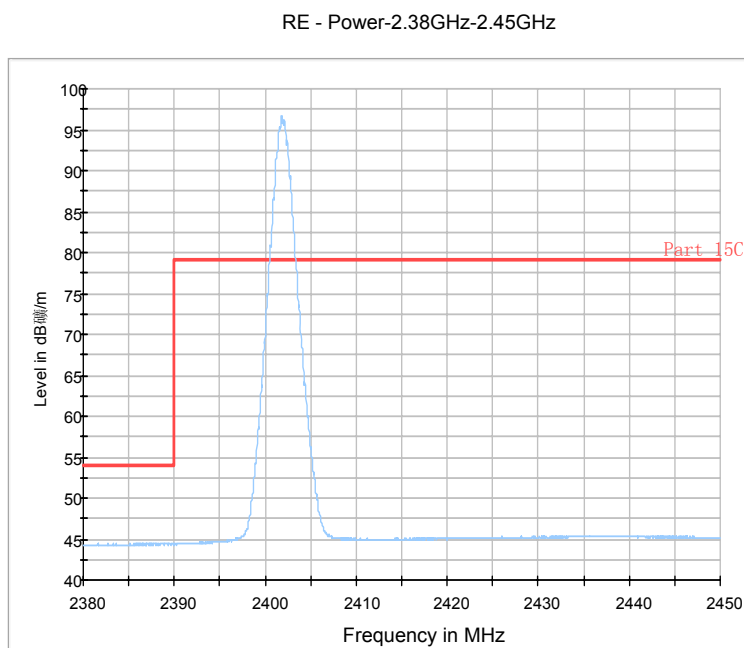
Fig.79. Radiated emission (Power): \pi/4 DQPSK, low channel
