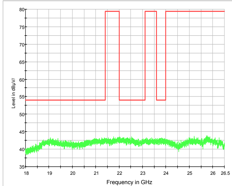
Fig.81. Radiated emission: \pi/4 DQPSK, 18 GHz - 26 GHz
