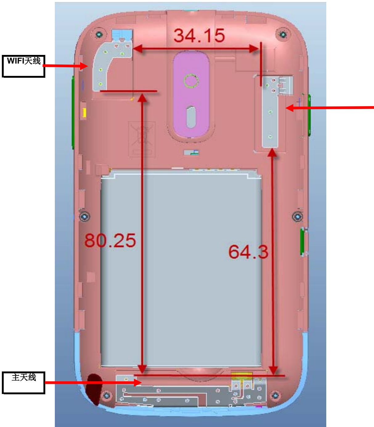
ONETOUCH 838 Antenna gain
