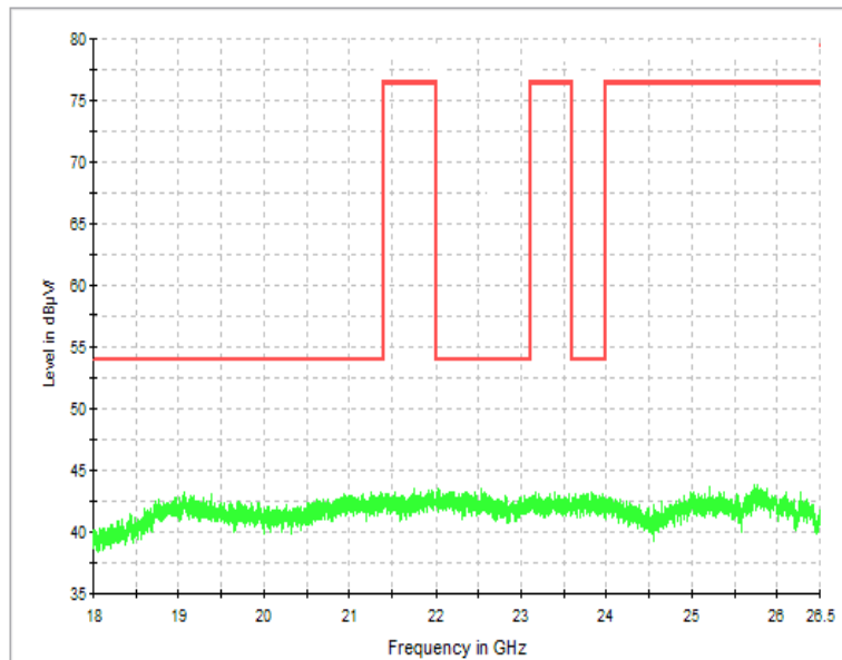
Fig.93. Radiated emission: 8DPSK, 18 GHz - 26 GHz
