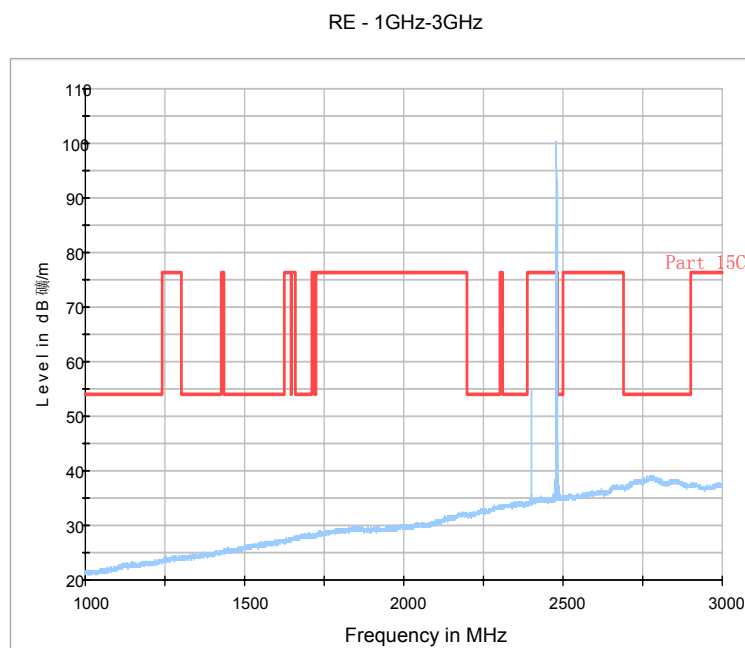
Fig.65. Radiated emission: GFSK, Channel 78, 1 GHz - 3 GHz
