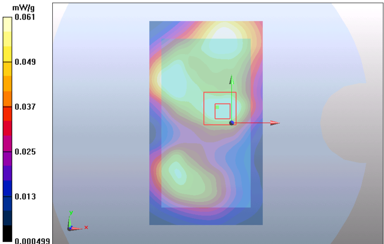
Figure 62 Body, Towards Phantom, 802.11b Channel 11
