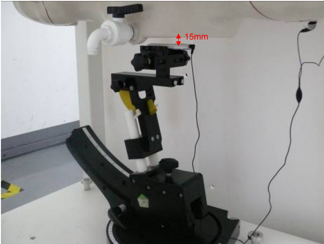
Picture 13: Body with Stereo Headset 1, The EUT display towards ground, the distance from EUT to the bottom of the Phantom is 15mm
