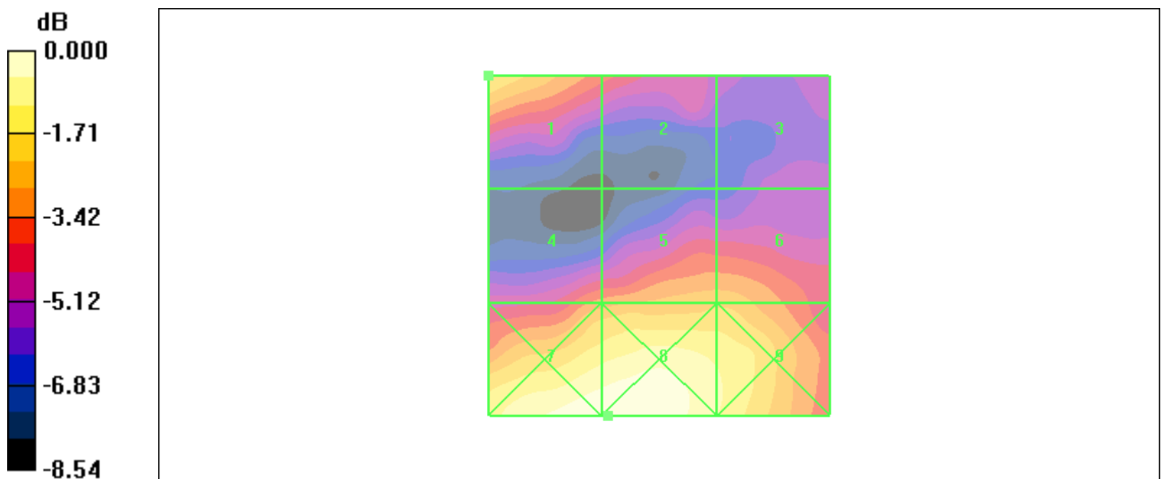
Figure 25 HAC RF E-Field GSM 1900 Channel 512
