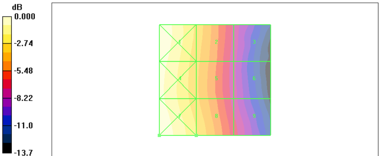
Figure 45 HAC RF H-Field WCDMA Band V Channel 4233
