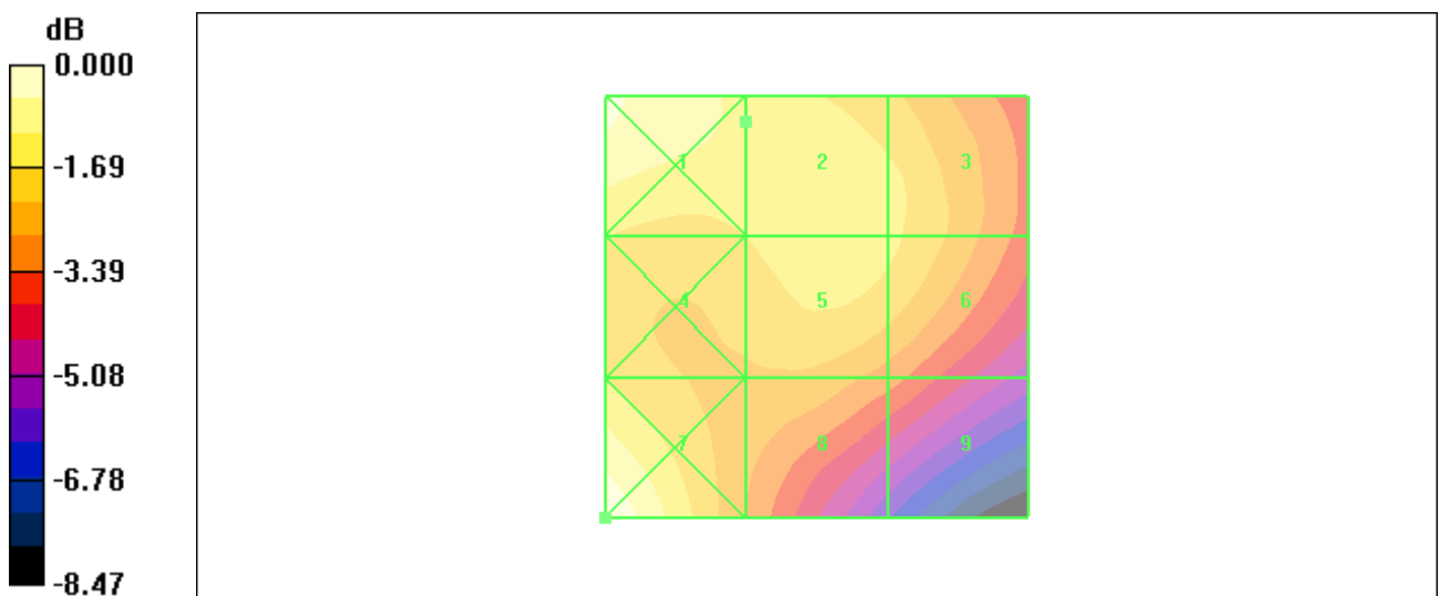
Figure 29 HAC RF H-Field GSM 1900 Channel 512
