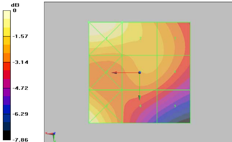
Figure 37 HAC RF H-Field WCDMA Band II Channel 9400
