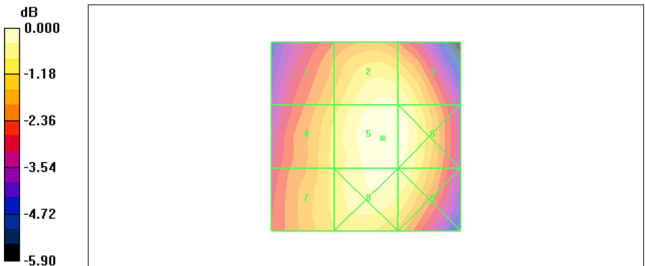
Figure 15 HAC RF E-Field GSM 850 Channel 190
