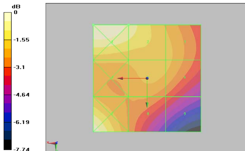
Figure 34 HAC RF H-Field WCDMA Band II Channel 9538
