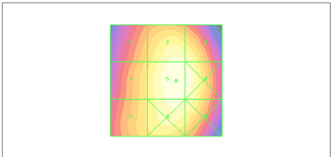
Figure 38 HAC RF E-Field WCDMA Band V Channel 4233
