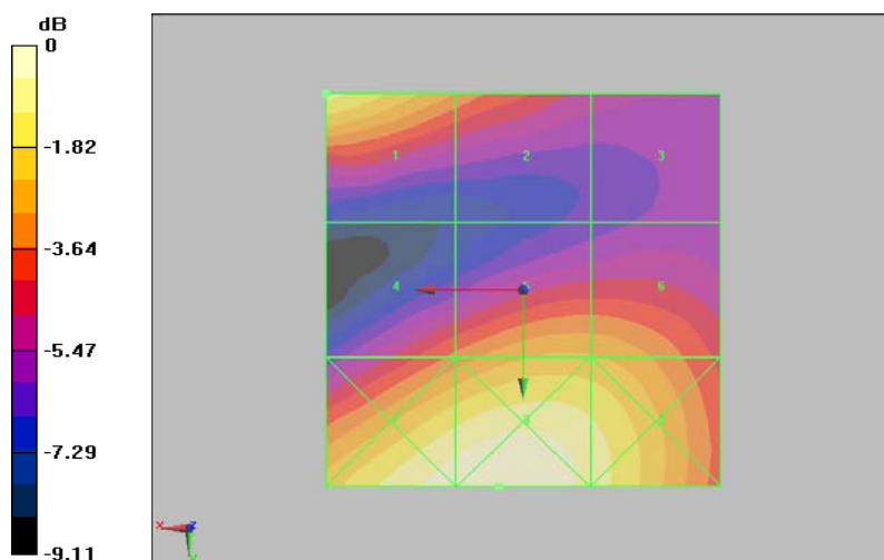
Figure 31 HAC RF E-Field WCDMA Band II Channel 9400
