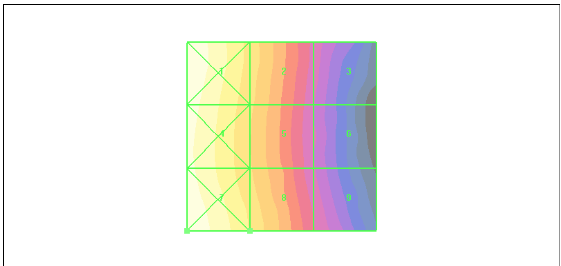
Figure 43 HAC RF H-Field WCDMA Band V Channel 4183
