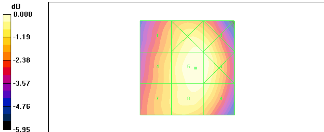
Figure 14 HAC RF E-Field GSM 850 Channel 251
