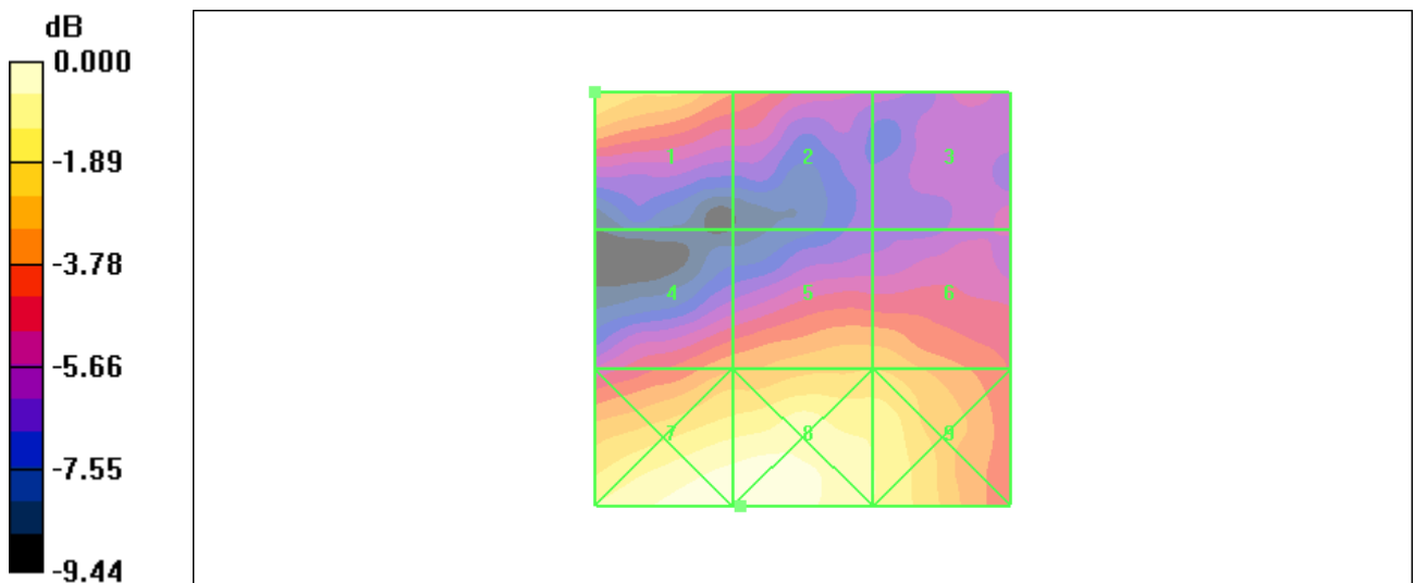
Figure 24 HAC RF E-Field GSM 1900 Channel 512
