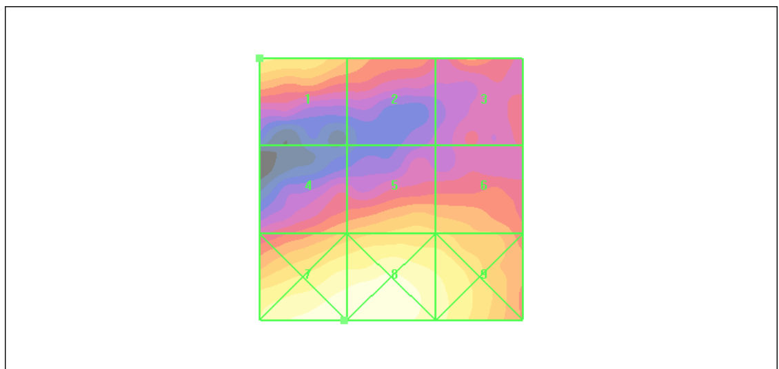
Figure 23 HAC RF E-Field GSM 1900 Channel 661
