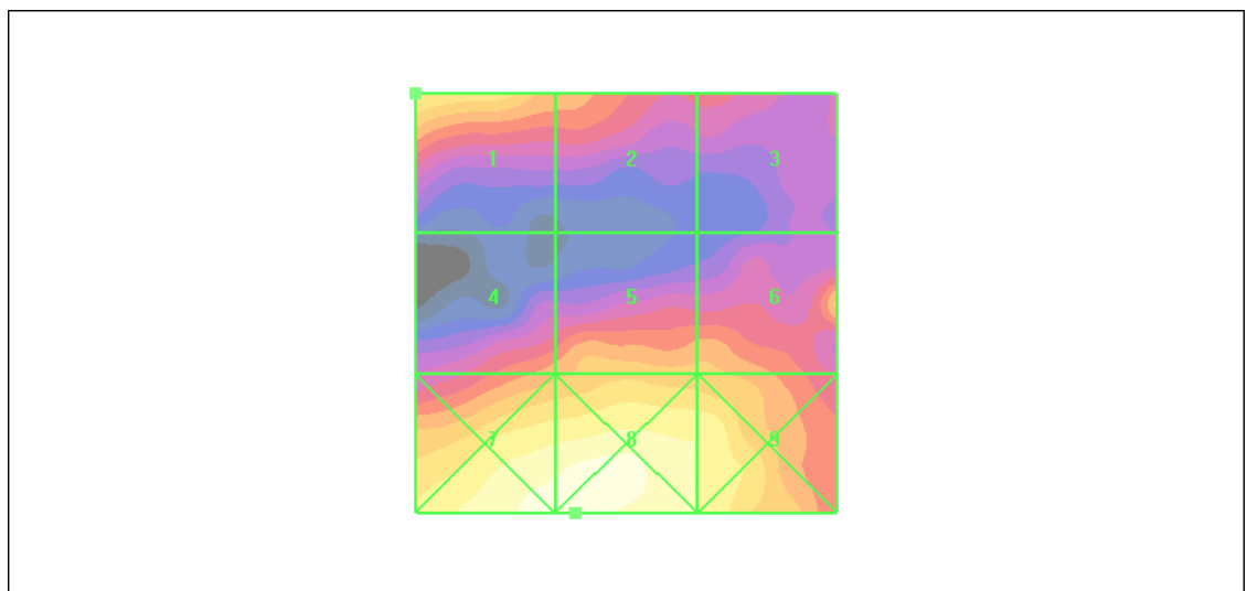
Figure 22 HAC RF E-Field GSM 1900 Channel 810
