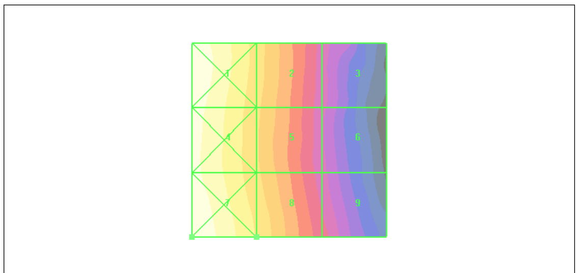
Figure 21 HAC RF H-Field GSM 850Channel 251
