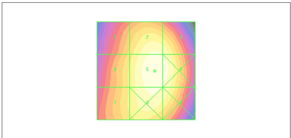
Figure 40 HAC RF E-Field WCDMA Band V Channel 4132
