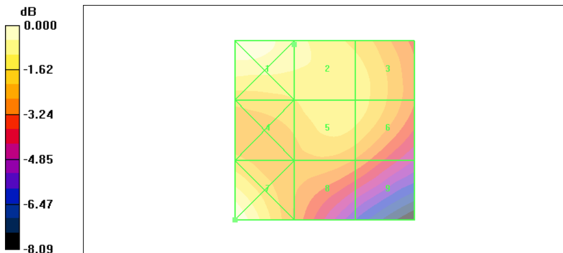
Figure 26 HAC RF H-Field GSM 1900 Channel 810
