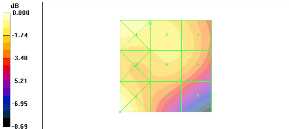
Figure 28 HAC RF H-Field GSM 1900 Channel 512
