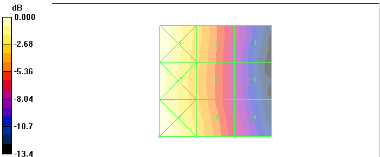
Figure 18 HAC RF H-Field GSM 850Channel 251
