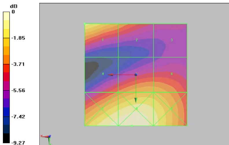
Figure 33 HAC RF E-Field WCDMA Band II Channel 9400
