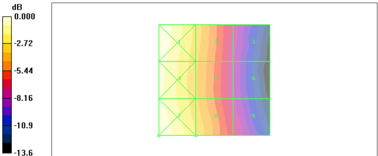
Figure 42 HAC RF H-Field WCDMA Band V Channel 4233
