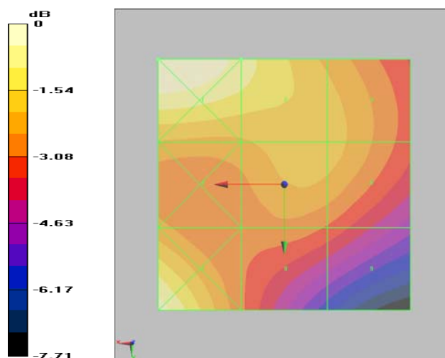
Figure 35 HAC RF H-Field WCDMA Band II Channel 9400
