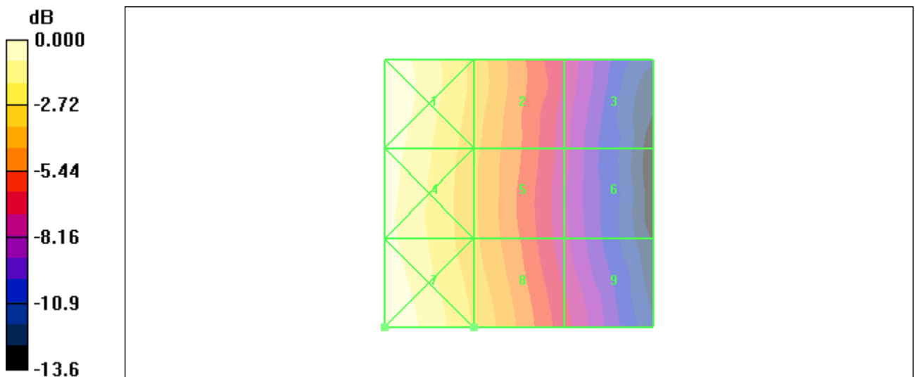
Figure 19 HAC RF H-Field GSM 850 Channel 190
