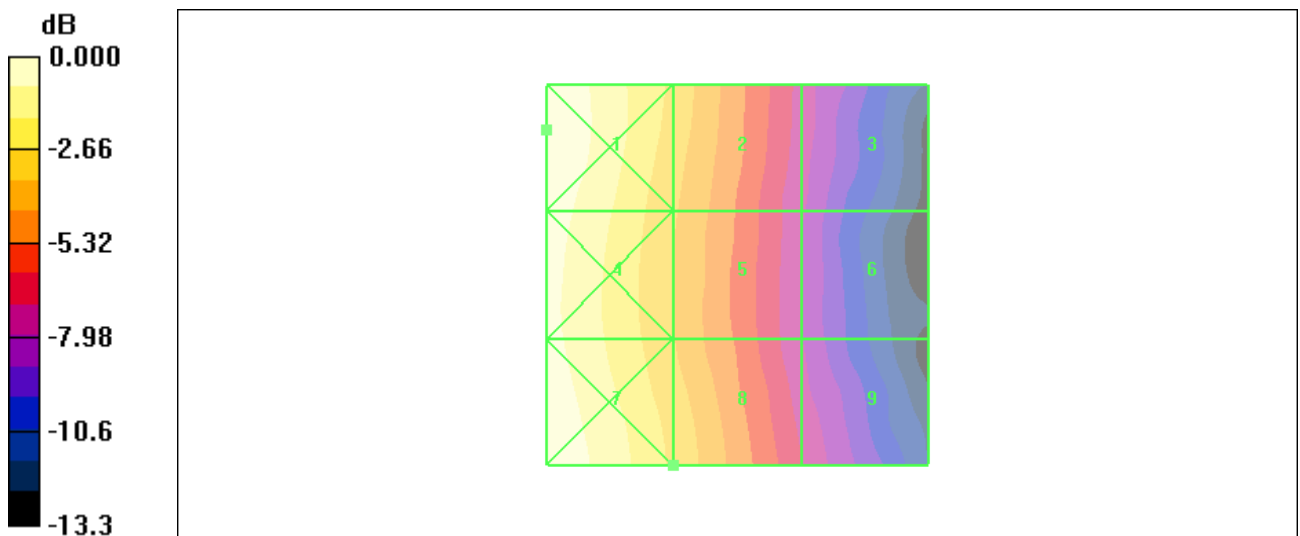
Figure 20 HAC RF H-Field GSM 850 Channel 128
