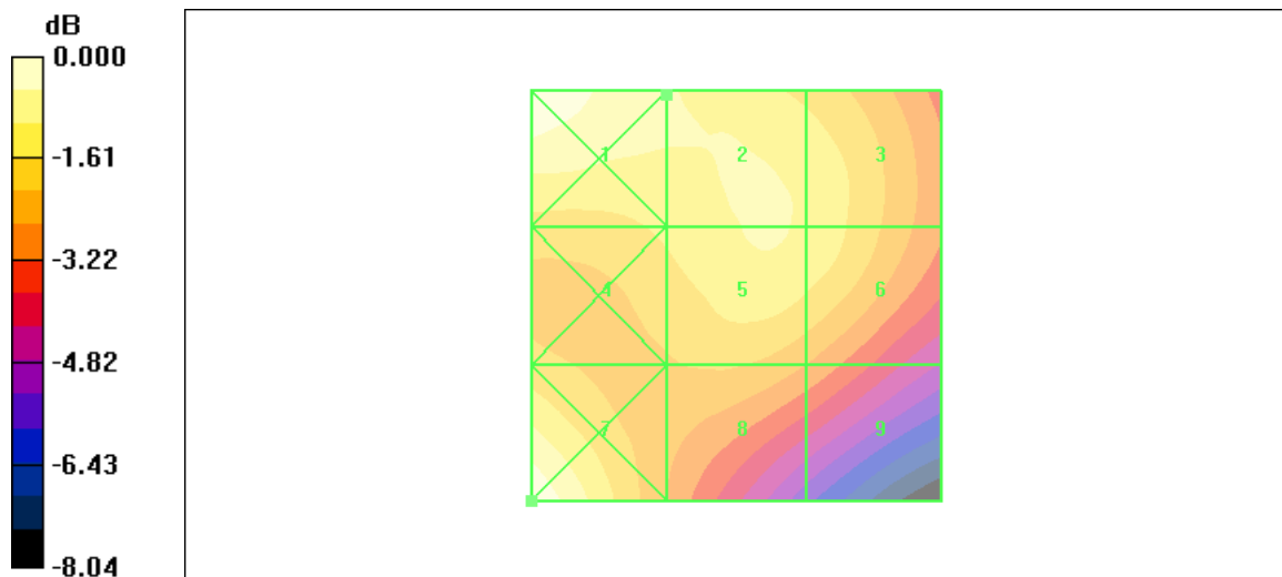
Figure 27 HAC RF H-Field GSM 1900 Channel 661
