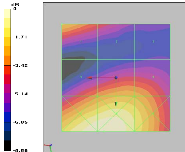
Figure 32 HAC RF E-Field WCDMA Band II Channel 9262
