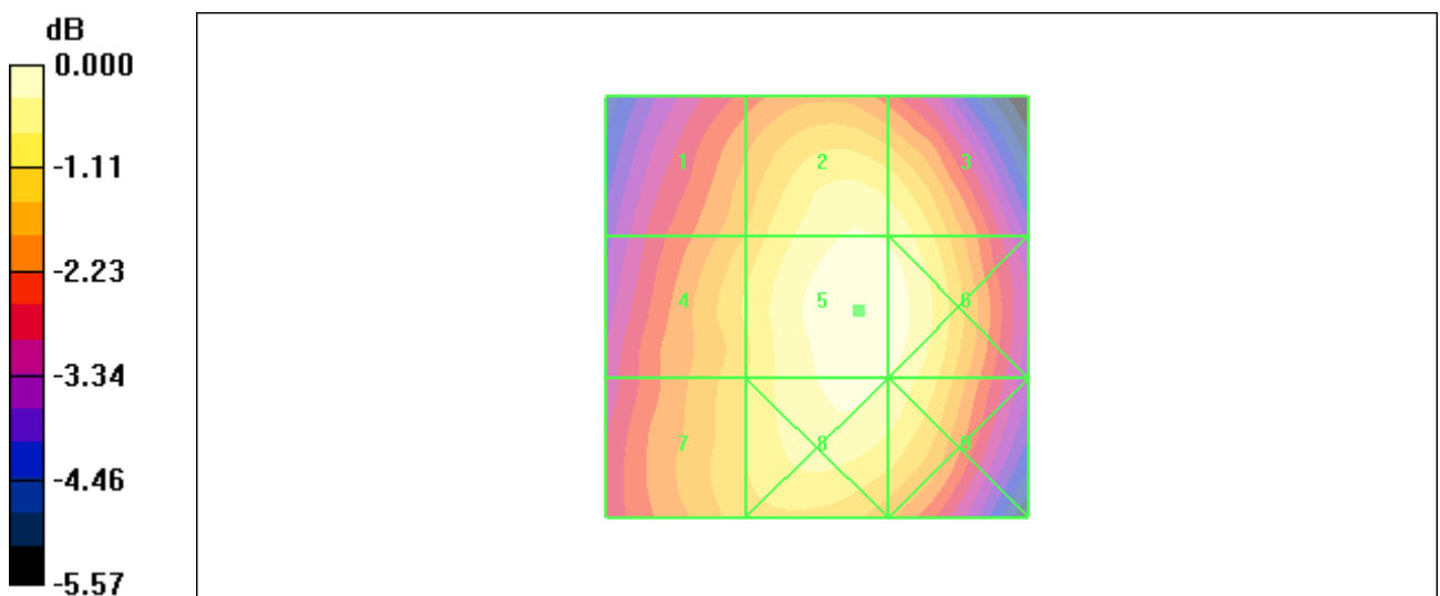
Figure 17 HAC RF E-Field GSM 850 Channel 190
