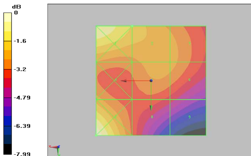
Figure 36 HAC RF H-Field WCDMA Band II Channel 9262
