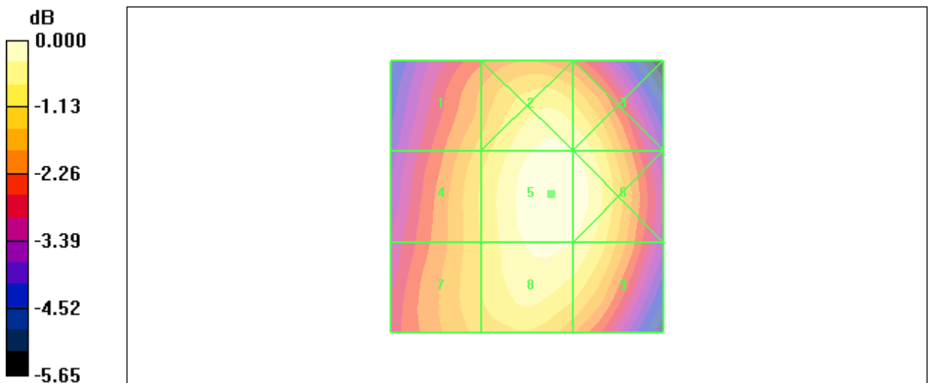
Figure 41 HAC RF E-Field WCDMA Band V Channel 4233
