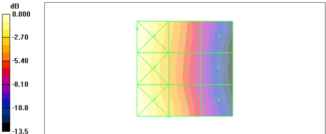
Figure 44 HAC RF H-Field WCDMA Band V Channel 4132
