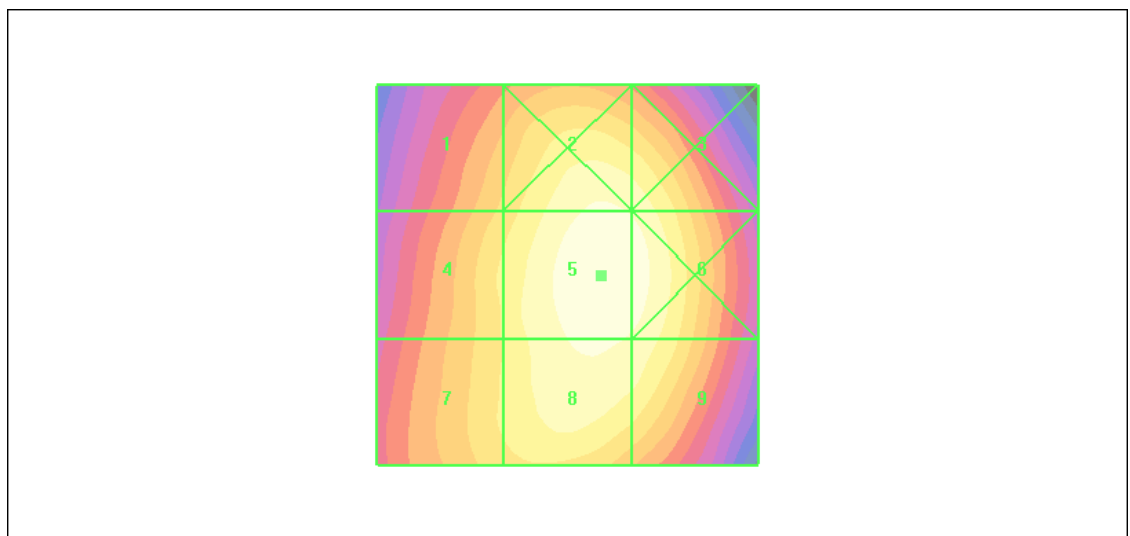
Figure 39 HAC RF E-Field WCDMA Band V Channel 4183
