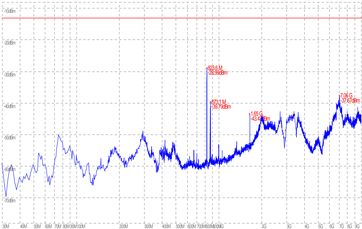
(Plot A.2: GSM 850MHz Channel = 128, Test Antenna Vertical)
