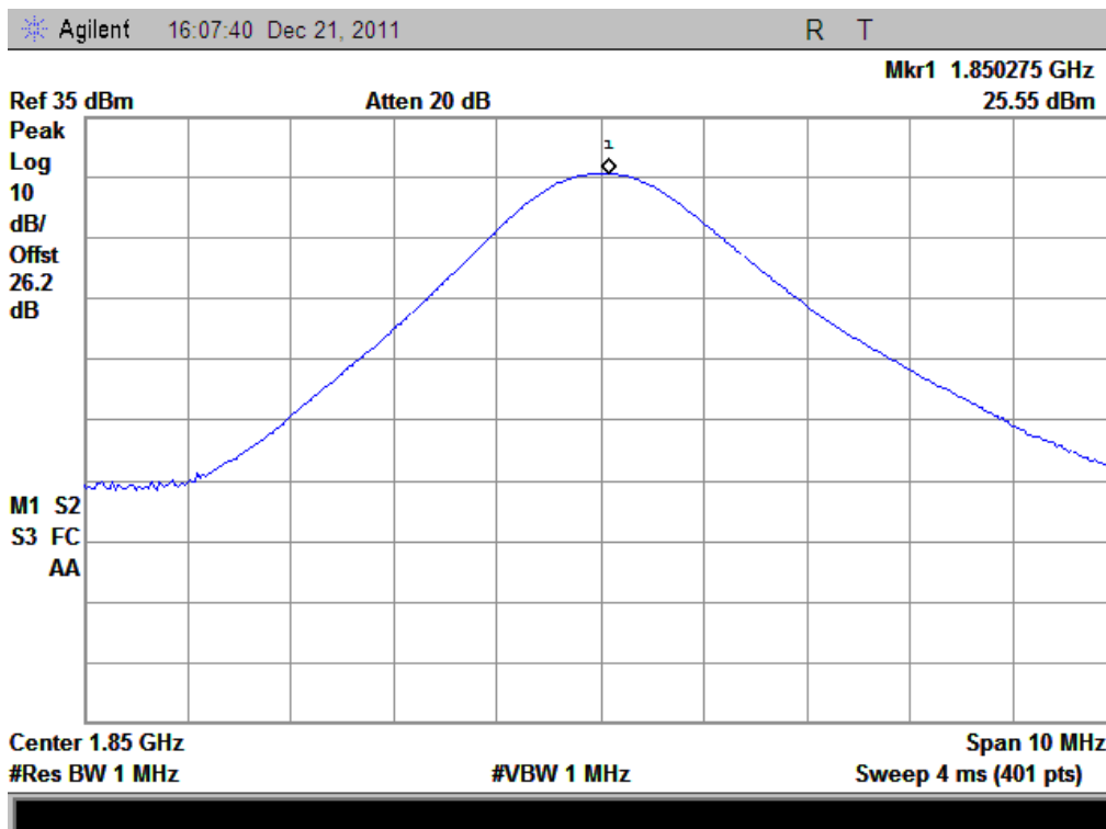
Plot F1: EGPRS 190MHz Channel = 512
