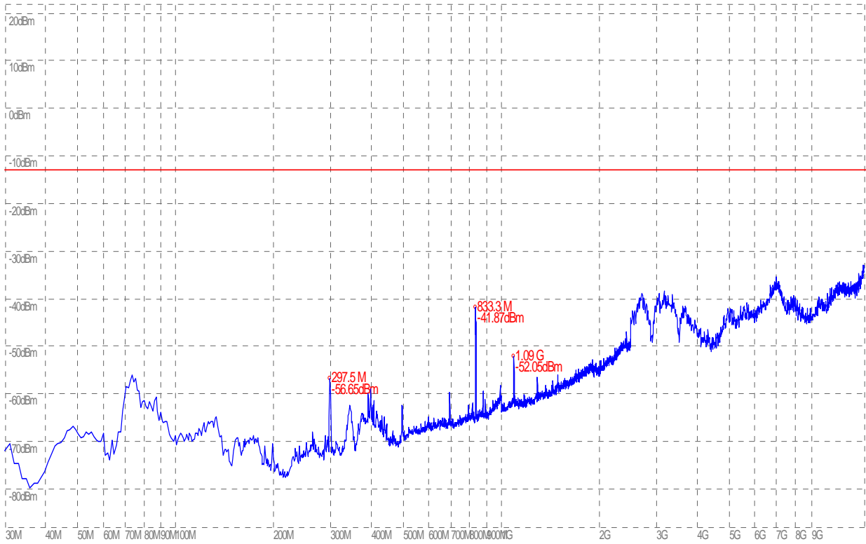
(Plot E.3: WCDMA 850MHz Channel = 4157, Test Antenna Horizontal)
