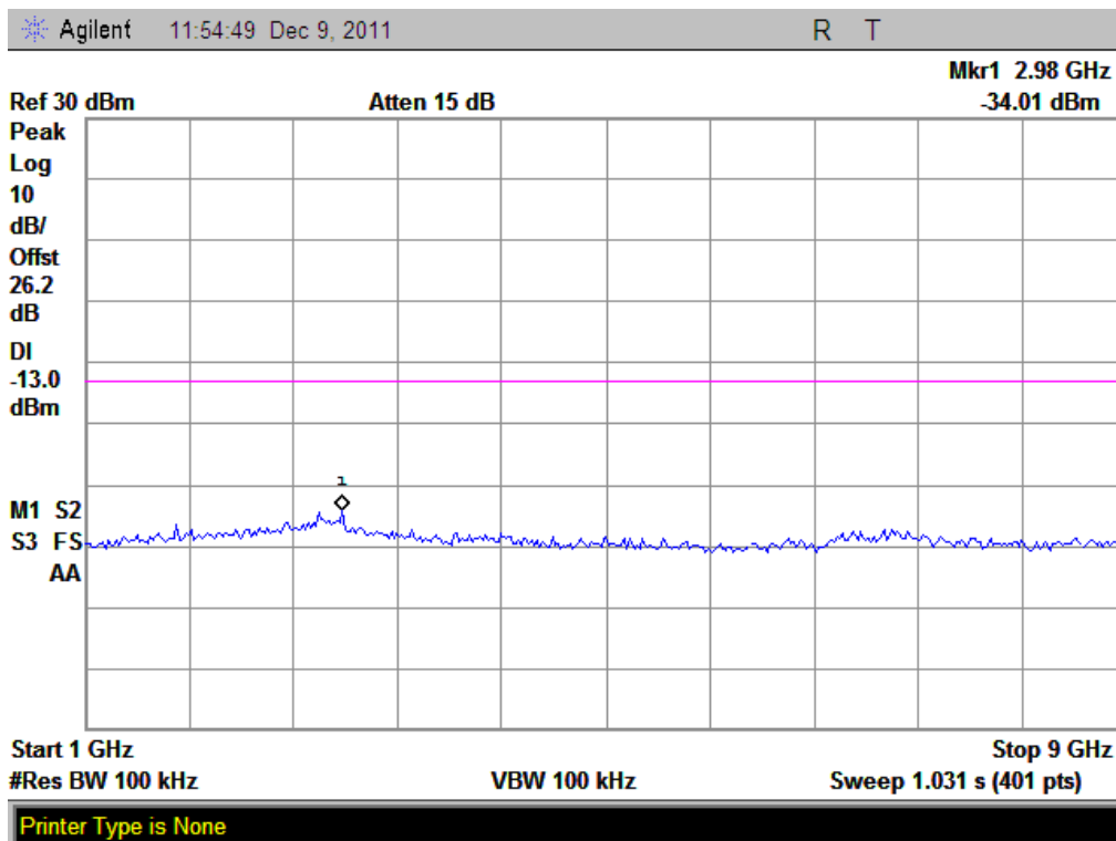
(Plot G2.1: HSDPA 850MHz Channel = 4157, 1GHz to 9GHz)
