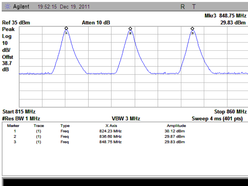
(Plot C: EGPRS 850 MHz Channel = 512, 661, 810)
