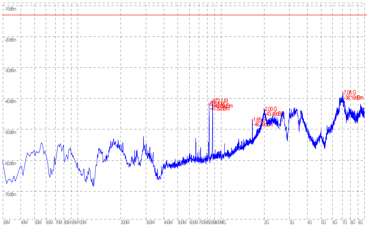
(Plot G.4: HSDPA 850MHz Channel = 4157 Test Antenna Vertical)
