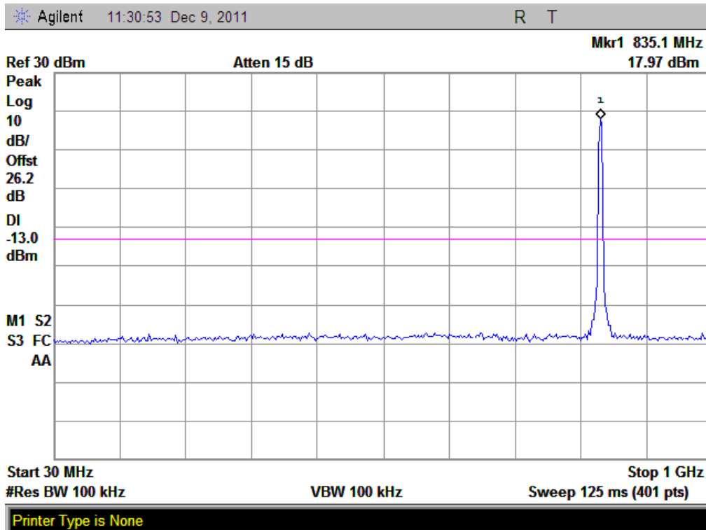
(Plot I 2: HSUPA 850MHz Channel = 4157, 30MHz to 1GHz)
