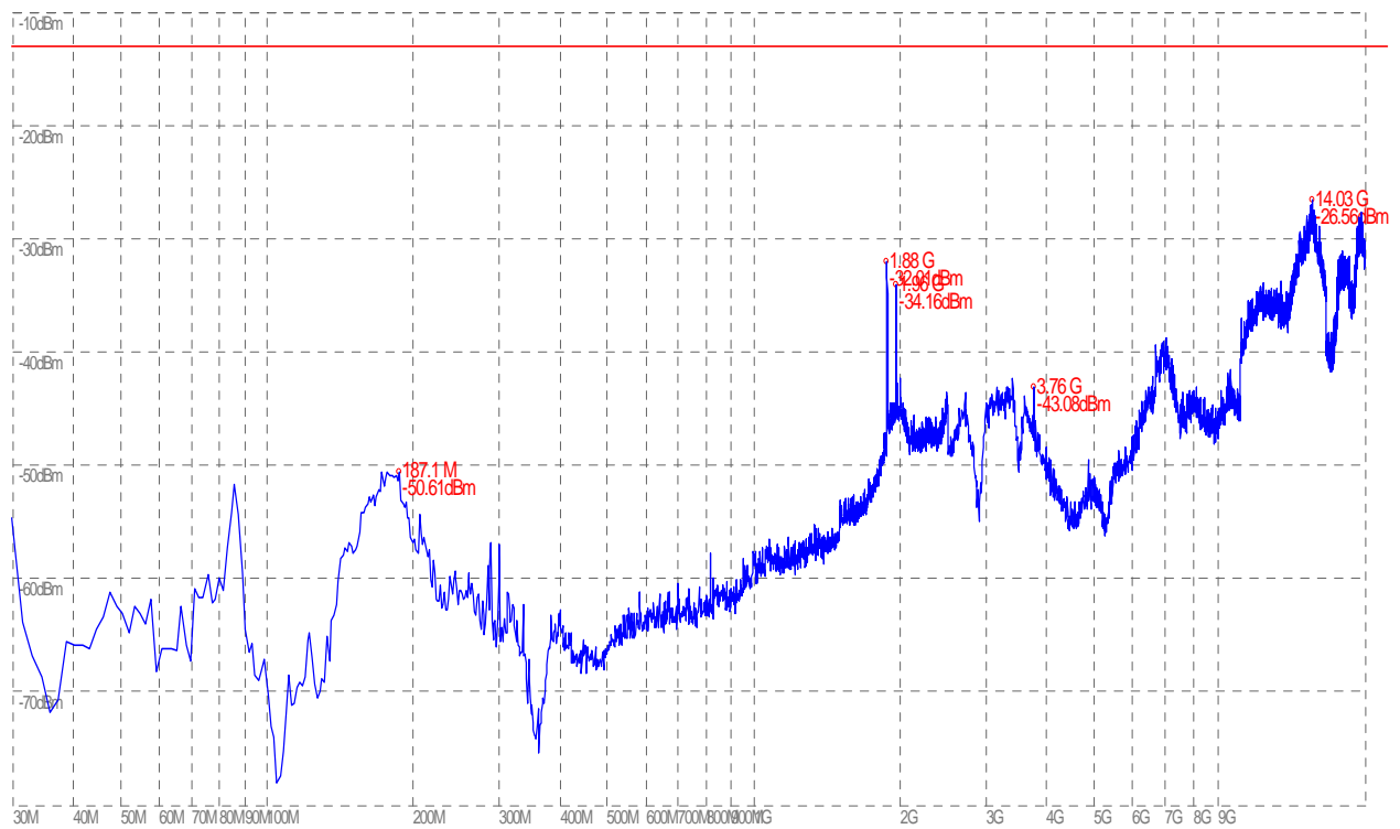
(Plot J.4: HSUPA 1900 MHz Channel = 9400, Test Antenna Vertical)
