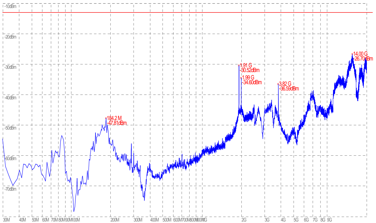
(Plot J.6: HSUPA 1900 MHz Channel = 9538, Test Antenna Vertical)
