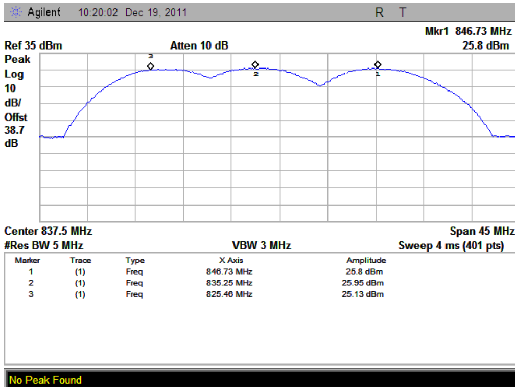
(Plot H: HSDPA 850MHz Channel = 4132, 4157, 4233)
