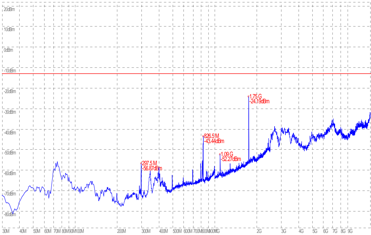
(Plot E.1: WCDMA 850MHz Channel = 4132, Test Antenna Horizontal)
