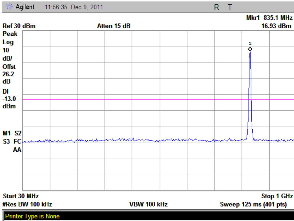
(Plot G2: HSDPA 850MHz Channel = 4157, 30MHz to 1GHz)
