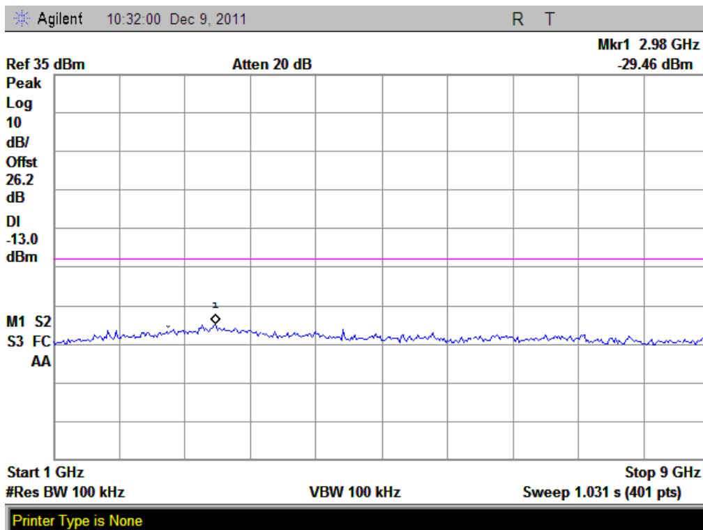
(Plot E2.1: WCDMA850MHz Channel = 4157, 1GHz to 9GHz)
