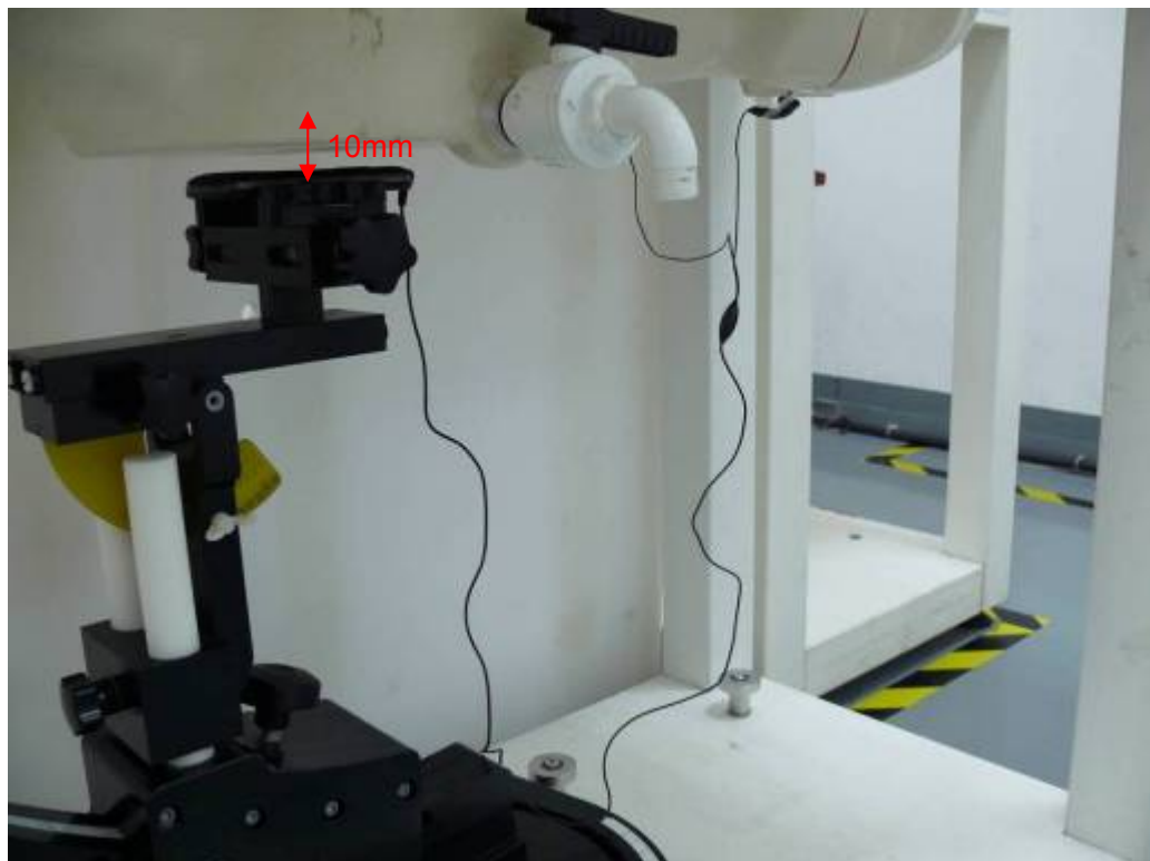
Picture 24: Back Side with Stereo Headset 2, the distance from handset to the bottom of the Phantom is 10mm(Battery 1)
