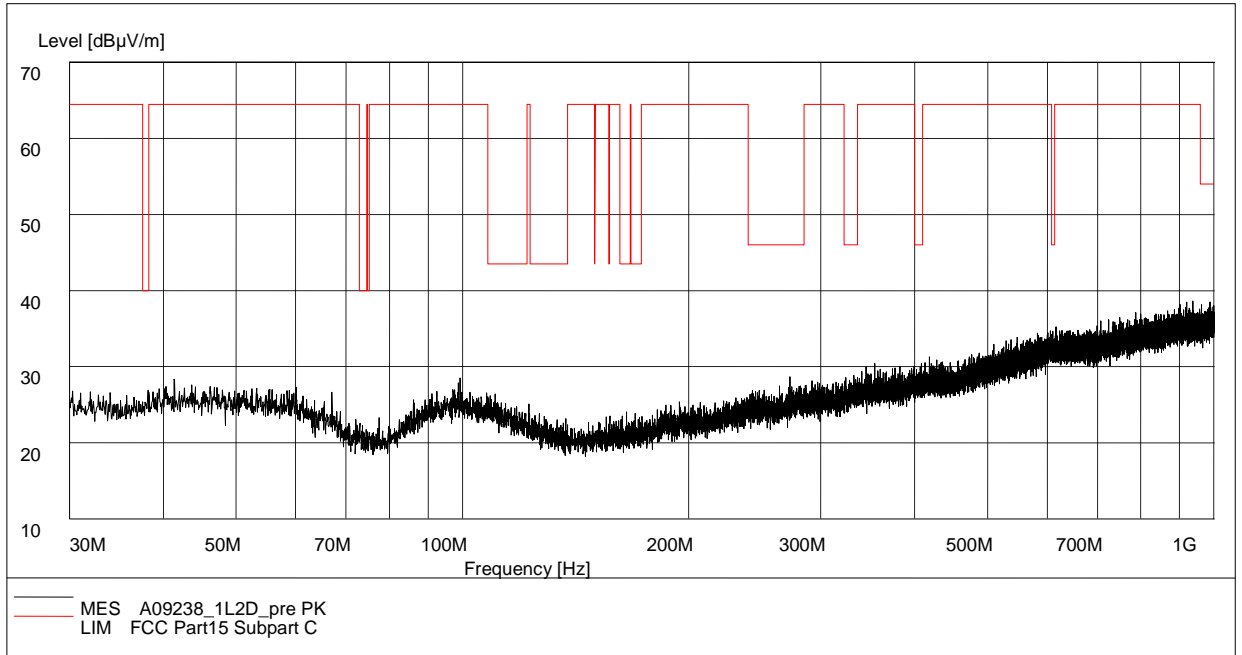
Fig.74. Radiated emission: \pi/4 DQPSK, Channel 0, 30 MHz - 1 GHz
