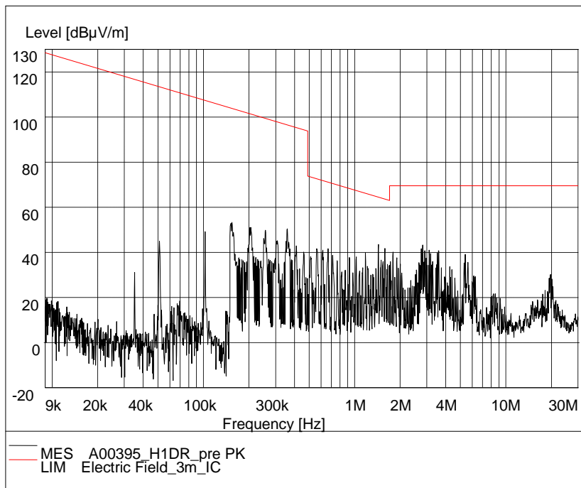
Fig.66. Radiated emission: GFSK, Channel 78, 9 KHz – 30MHz
