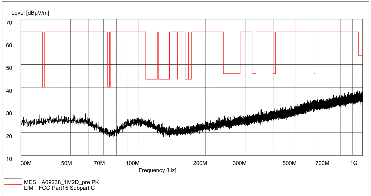
Fig.78. Radiated emission: \pi/4 DQPSK, Channel 39, 30 MHz - 1 GHz
