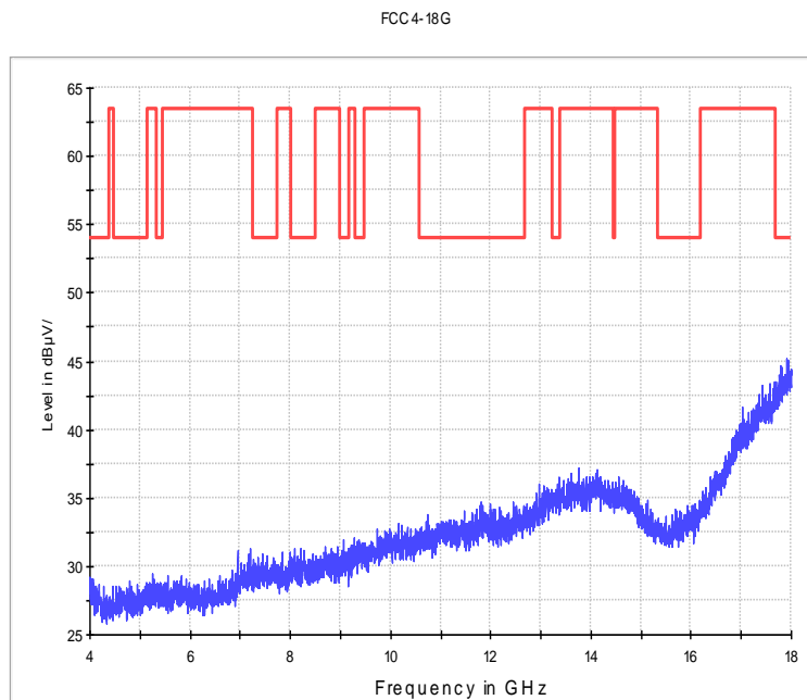
Fig.61. Radiated emission: GFSK, Channel 0, 4 GHz - 18 GHz
