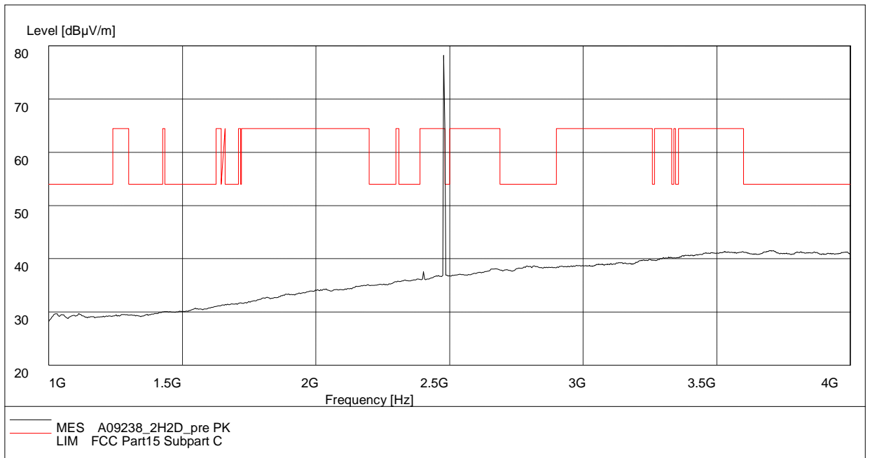
Fig.83. Radiated emission: \pi/4 DQPSK, Channel 78, 1 GHz - 4 GHz
