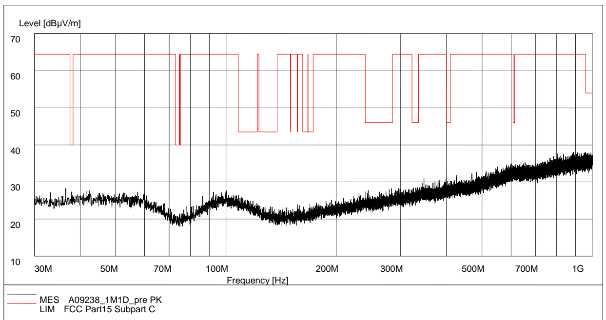
Fig.63. Radiated emission: GFSK, Channel 39, 30 MHz - 1 GHz
