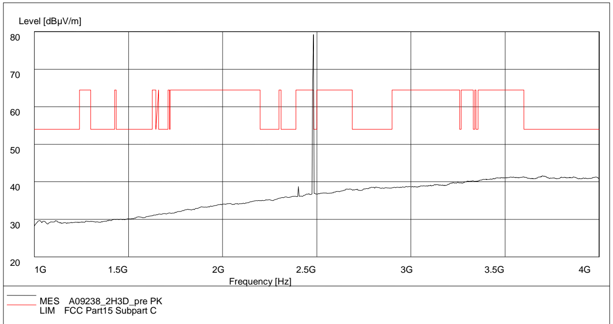
Fig.98. Radiated emission: 8DPSK, Channel 78, 1 GHz - 4 GHz
