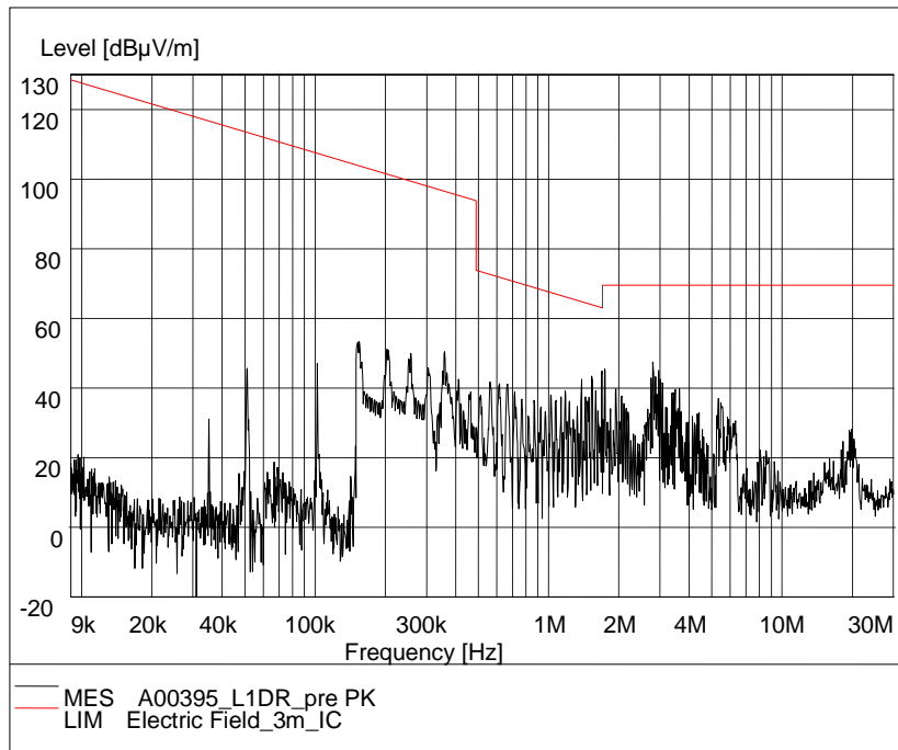
Fig.58. Radiated emission: GFSK, Channel 0, 9 KHz – 30MHz
