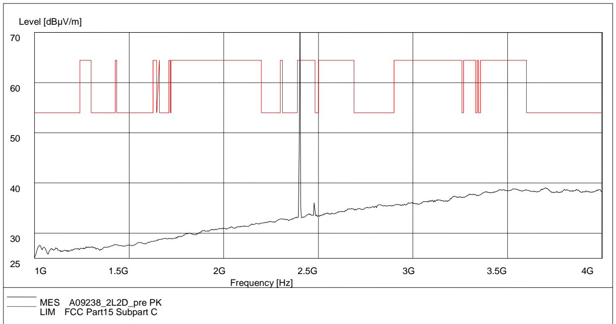
Fig.75. Radiated emission: \pi/4 DQPSK, Channel 0, 1 GHz - 4 GHz
