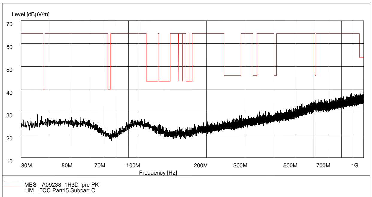
Fig.97. Radiated emission: 8DPSK, Channel 78, 30 MHz - 1 GHz
