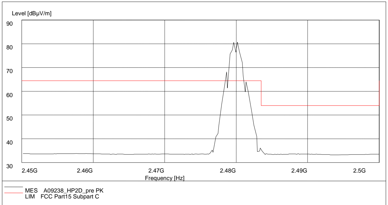
Fig.86. Radiated emission (Power): \pi/4 DQPSK, high channel
