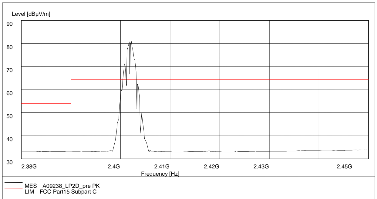
Fig.85. Radiated emission (Power): \pi/4 DQPSK, low channel
