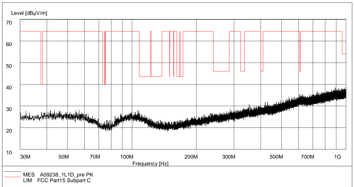
Fig.59. Radiated emission: GFSK, Channel 0, 30 MHz - 1 GHz
