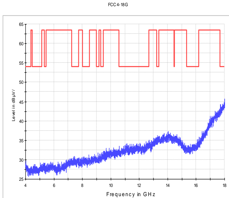
Fig.84. Radiated emission: \pi/4 DQPSK, Channel 78, 4 GHz - 18 GHz
