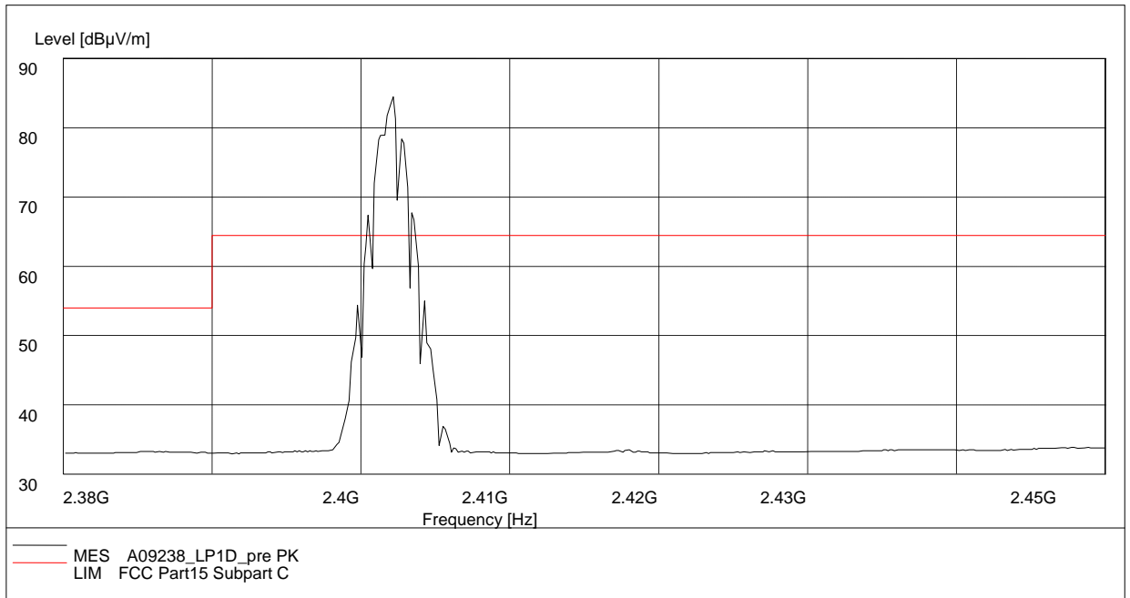
Fig.70. Radiated emission (Power): GFSK, low channel
