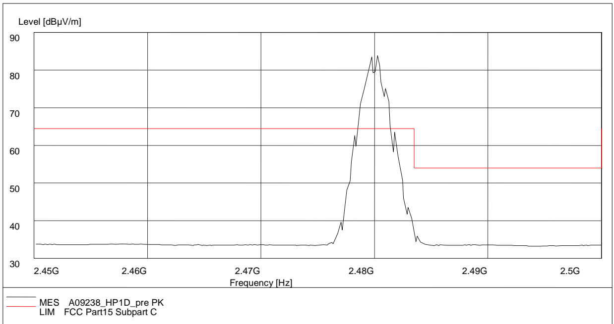
Fig.71. Radiated emission (Power) GFSK, high channel
