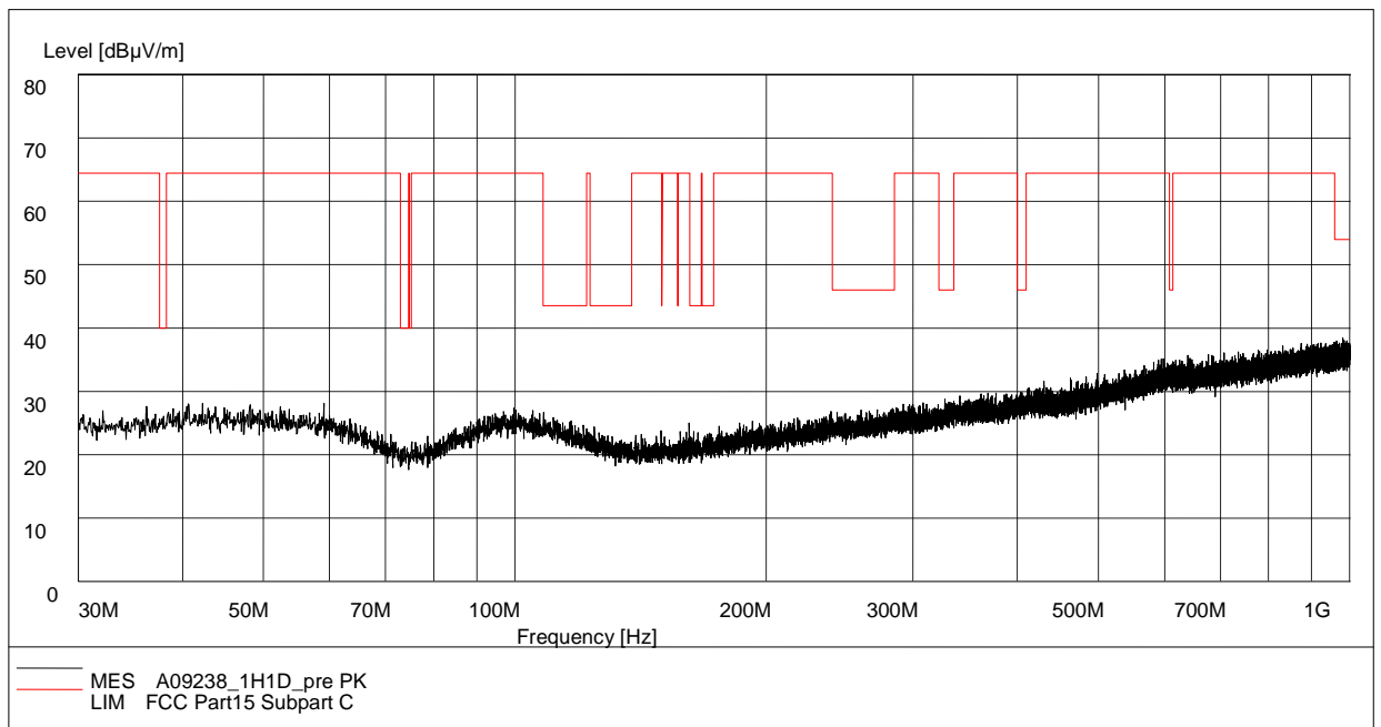
Fig.67. Radiated emission: GFSK, Channel 78, 30 MHz - 1 GHz
