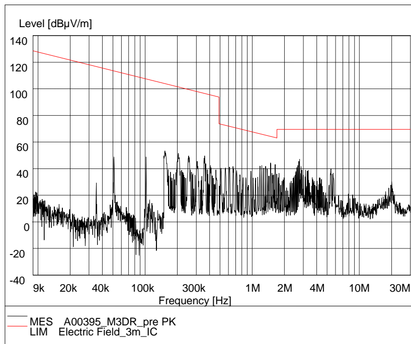
Fig.93. Radiated emission: 8DPSK, Channel 39, 9 KHz - 30MHz
