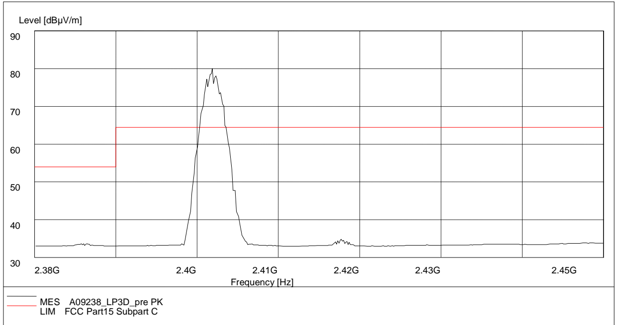
Fig.100. Radiated emission (Power): 8DPSK, low channel
