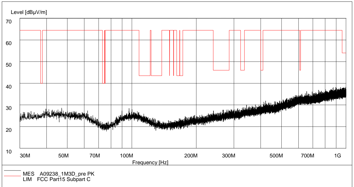
Fig.92. Radiated emission: 8DPSK, Channel 39, 30 MHz - 1 GHz
