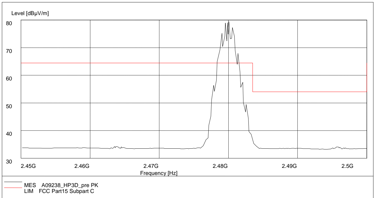
Fig.101. Radiated emission (Power): 8DPSK, high channel
