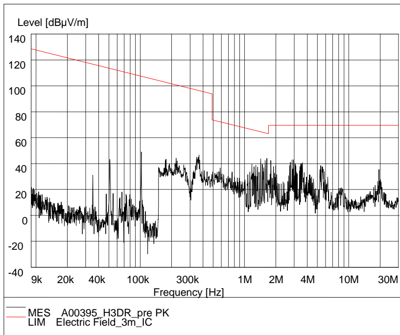
Fig.96. Radiated emission: 8DPSK, Channel 78, 9 KHz – 30MHz
