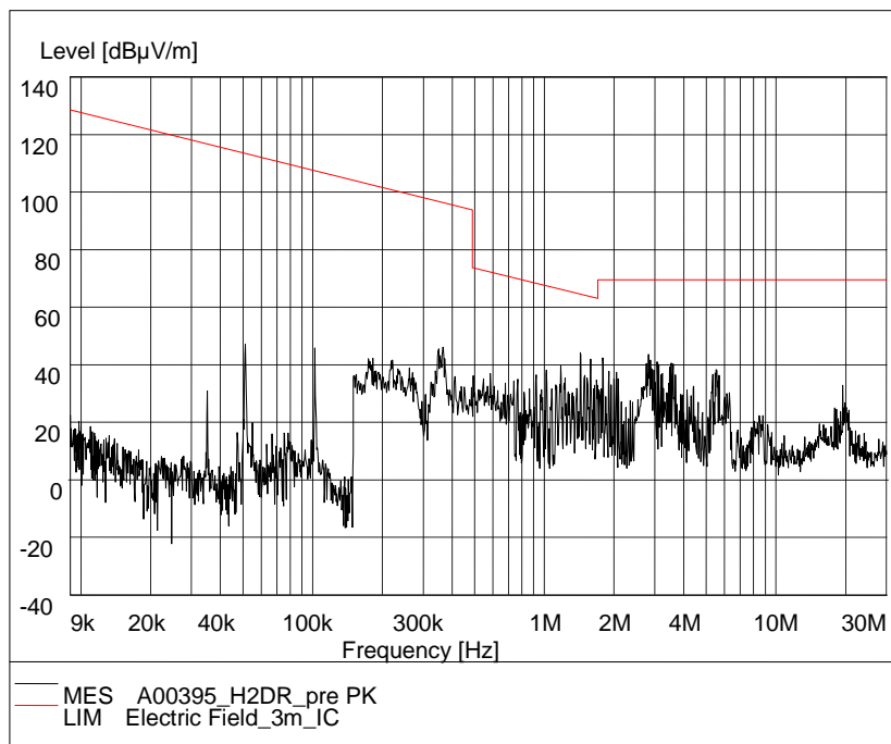
Fig.81. Radiated emission: \pi/4 DQPSK, Channel 39, 9 KHz – 30MHz
