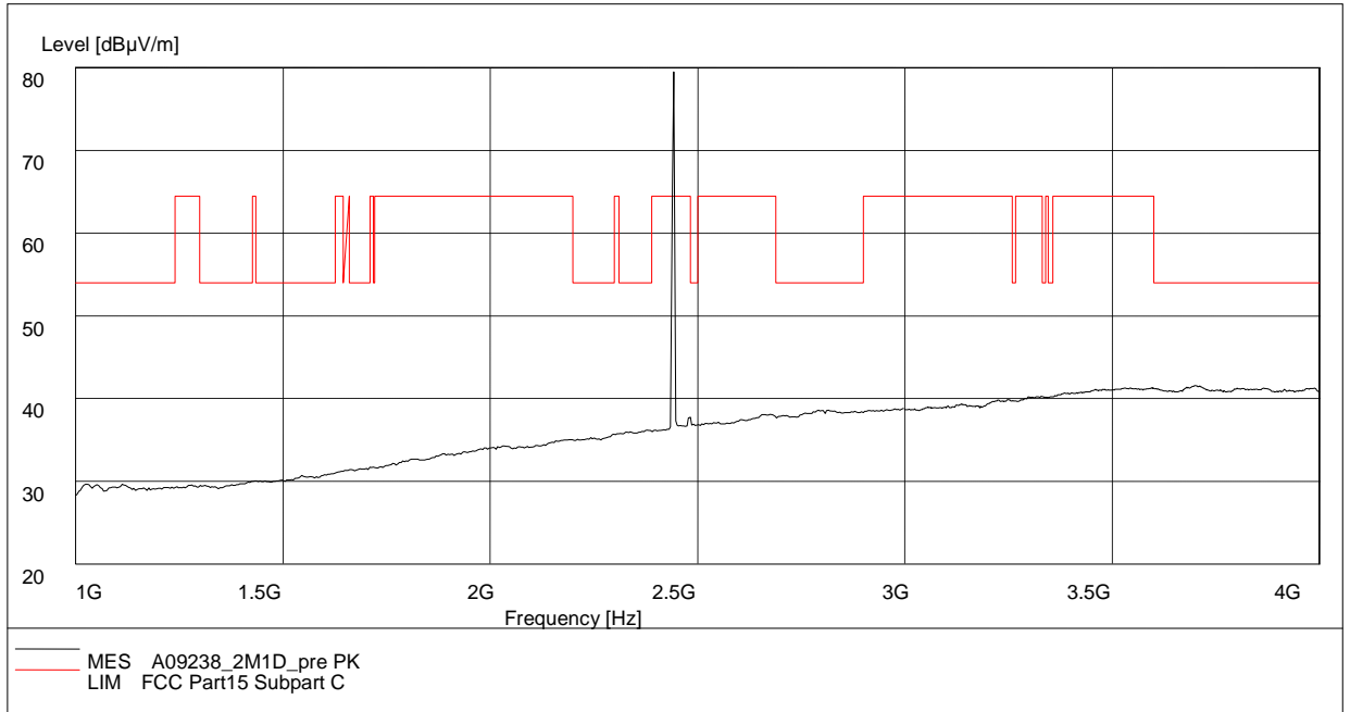
Fig.64. Radiated emission: GFSK, Channel 39, 1 GHz - 4 GHz
