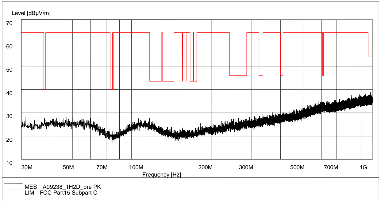
Fig.82. Radiated emission: \pi/4 DQPSK, Channel 78, 30 MHz - 1 GHz
