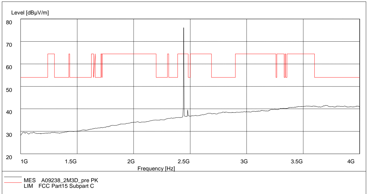
Fig.94. Radiated emission: 8DPSK, Channel 39, 1 GHz - 4 GHz
