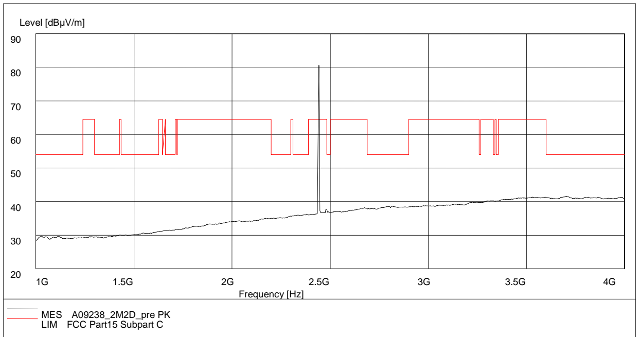
Fig.79. Radiated emission: \pi/4 DQPSK, Channel 39, 1 GHz - 4 GHz
