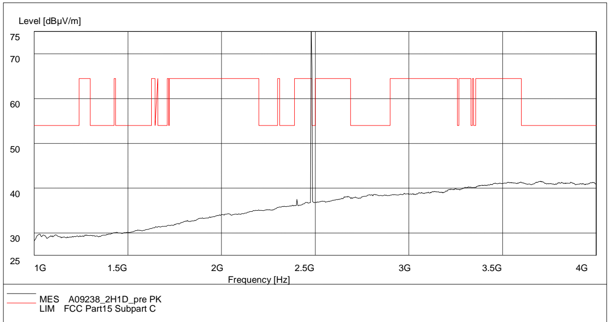
Fig.68. Radiated emission: GFSK, Channel 78, 1 GHz - 4 GHz
