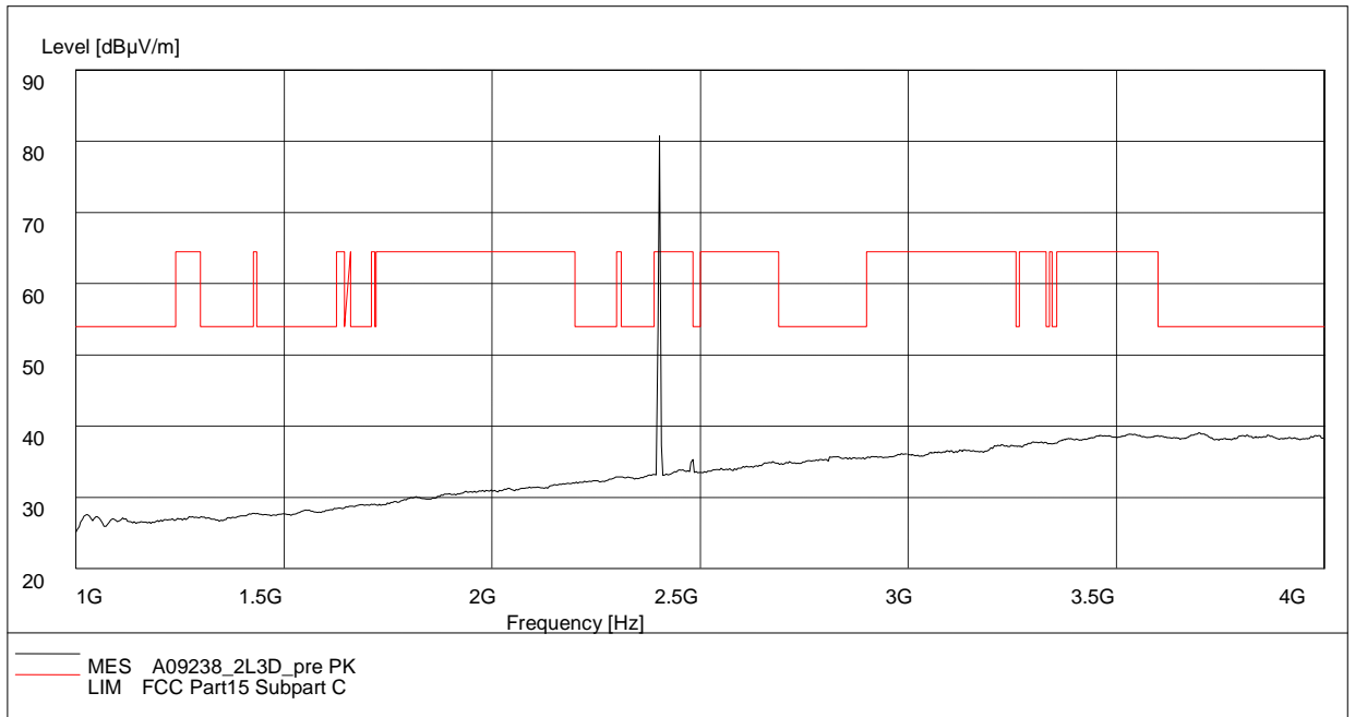
Fig.90. Radiated emission: 8DPSK, Channel 0, 1 GHz - 4 GHz
