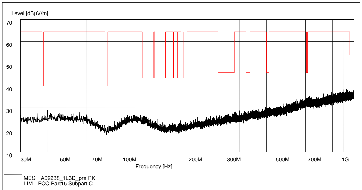
Fig.89. Radiated emission: 8DPSK, Channel 0, 30 MHz - 1 GHz
