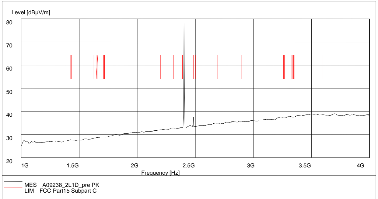
Fig.60. Radiated emission: GFSK, Channel 0, 1 GHz - 4 GHz
