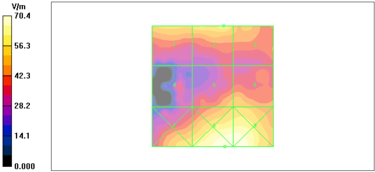
Figure 22 HAC RF E-Field GSM 1900 Channel 512
