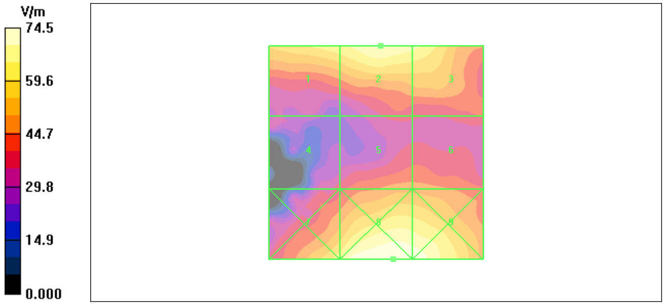
Figure 20 HAC RF E-Field GSM 1900 Channel 810
