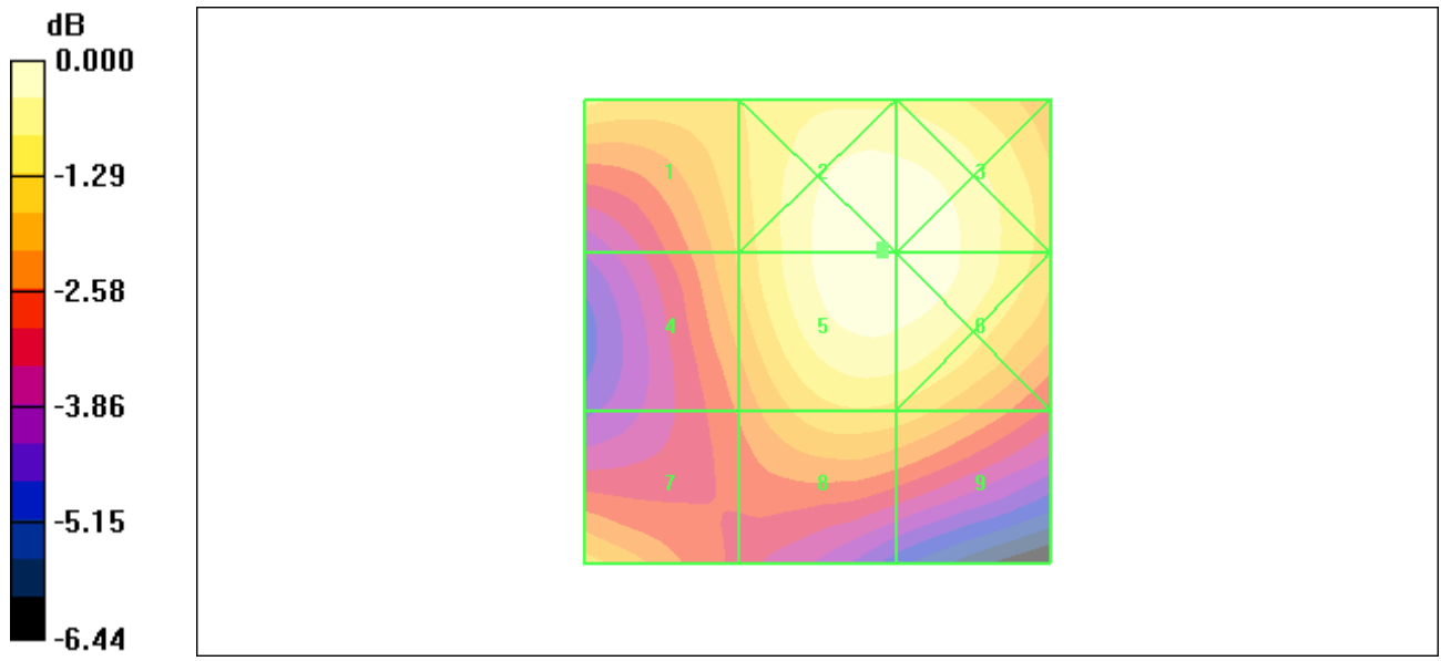
Figure 26 HAC RF H-Field GSM 1900 Channel 512
