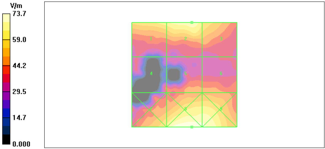
Figure 21 HAC RF E-Field GSM 1900 Channel 661
