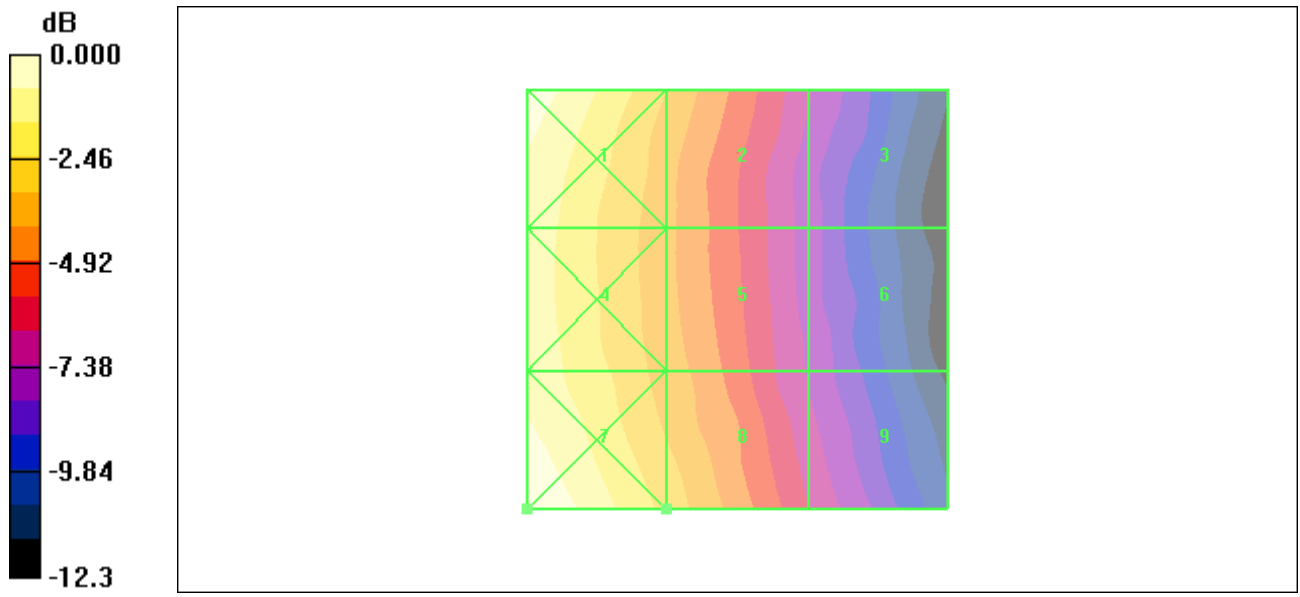
Figure 19 HAC RF H-Field GSM 850 Channel 251
