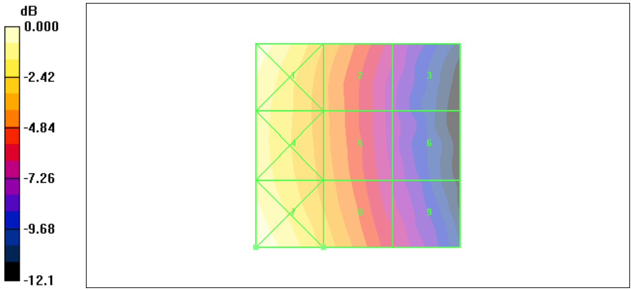
Figure 40 HAC RF H-Field WCDMA Band V Channel 4233
