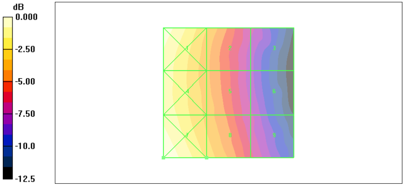
Figure 41 HAC RF H-Field WCDMA Band V Channel 4183
