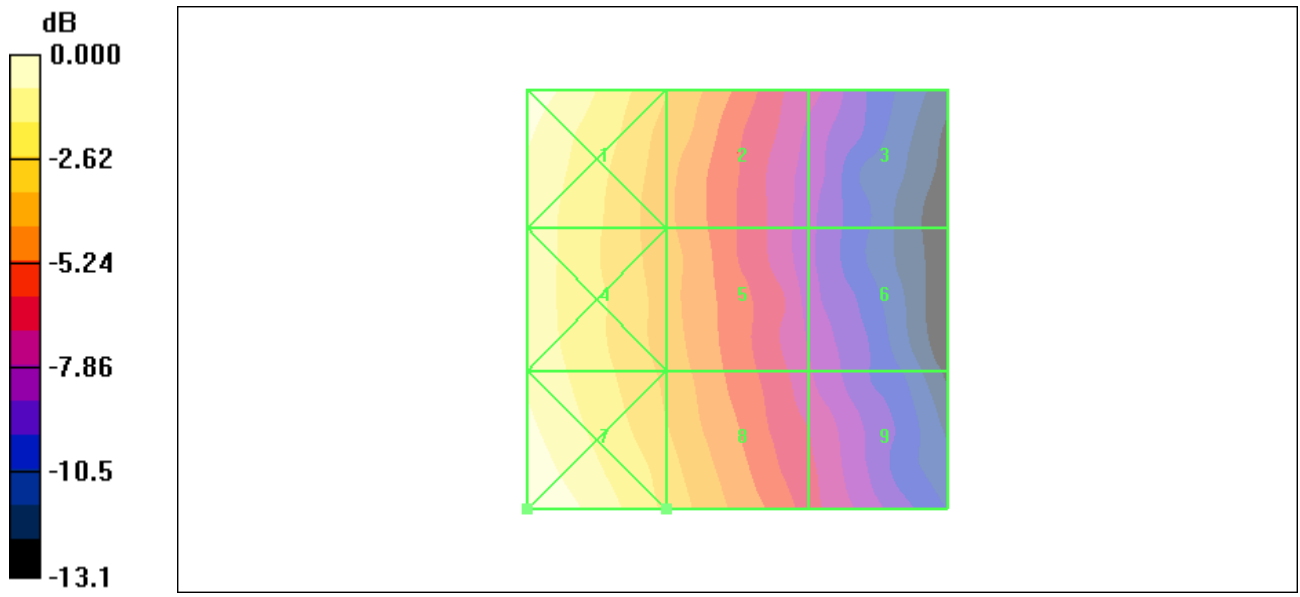
Figure 18 HAC RF H-Field GSM 850 Channel 128
