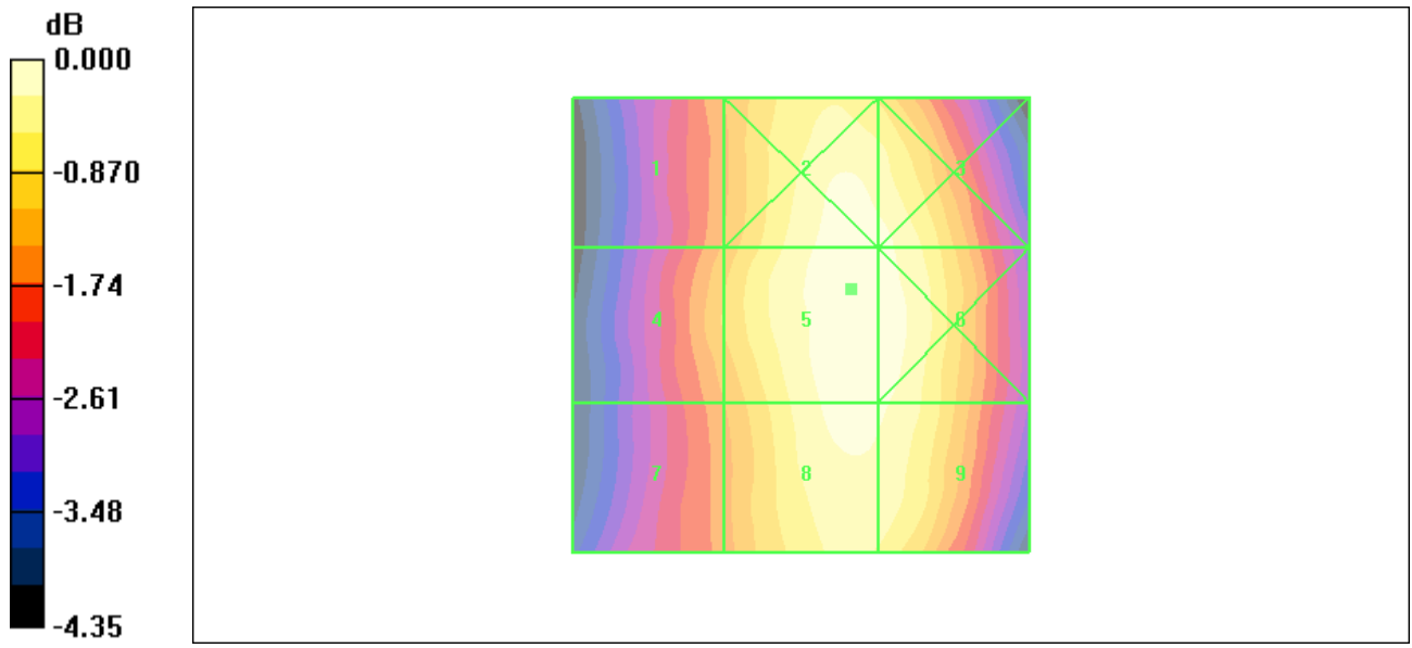
Figure 38 HAC RF E-Field WCDMA Band V Channel 4132
