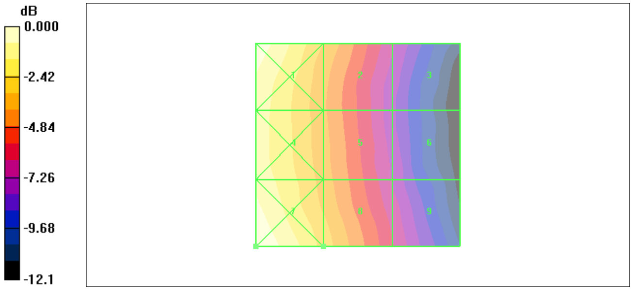
Figure 16 HAC RF H-Field GSM 850Channel 251
