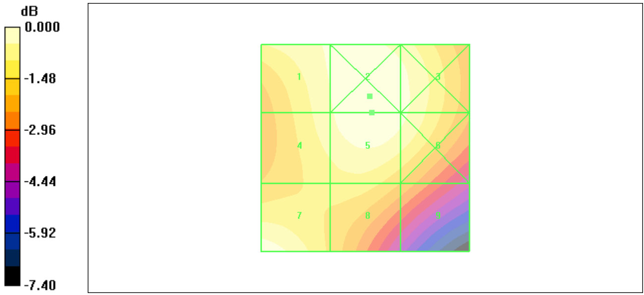
Figure 34 HAC RF H-Field WCDMA Band IV Channel 1312
