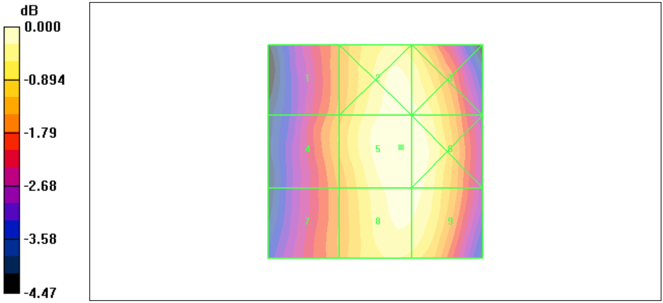
Figure 37 HAC RF E-Field WCDMA Band V Channel 4183
