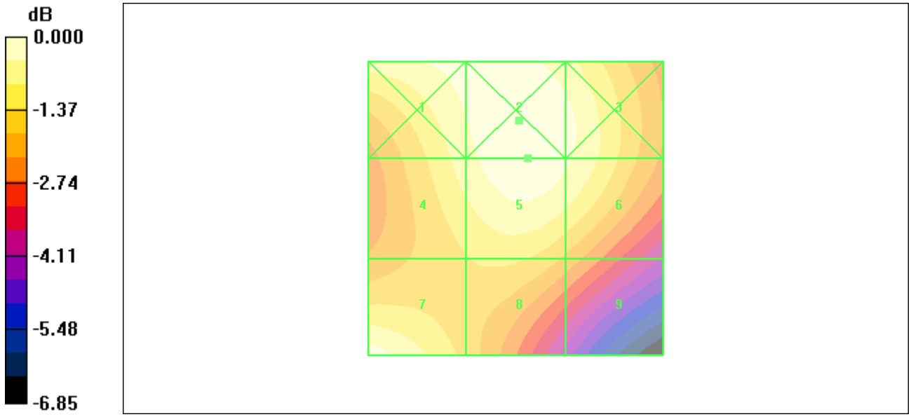
Figure 32 HAC RF H-Field WCDMA Band IV Channel 1513
