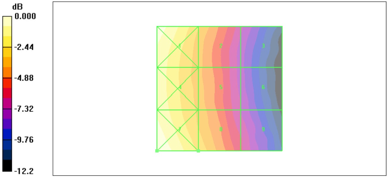
Figure 43 HAC RF H-Field WCDMA Band V Channel 4132
