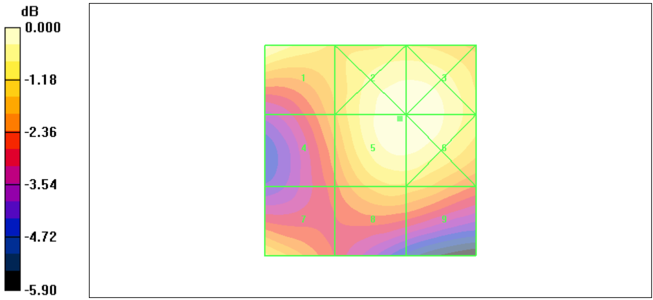
Figure 25 HAC RF H-Field GSM 1900 Channel 661
