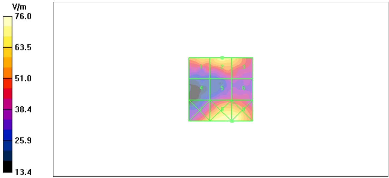
Figure 23 HAC RF E-Field GSM 1900 Channel 810
