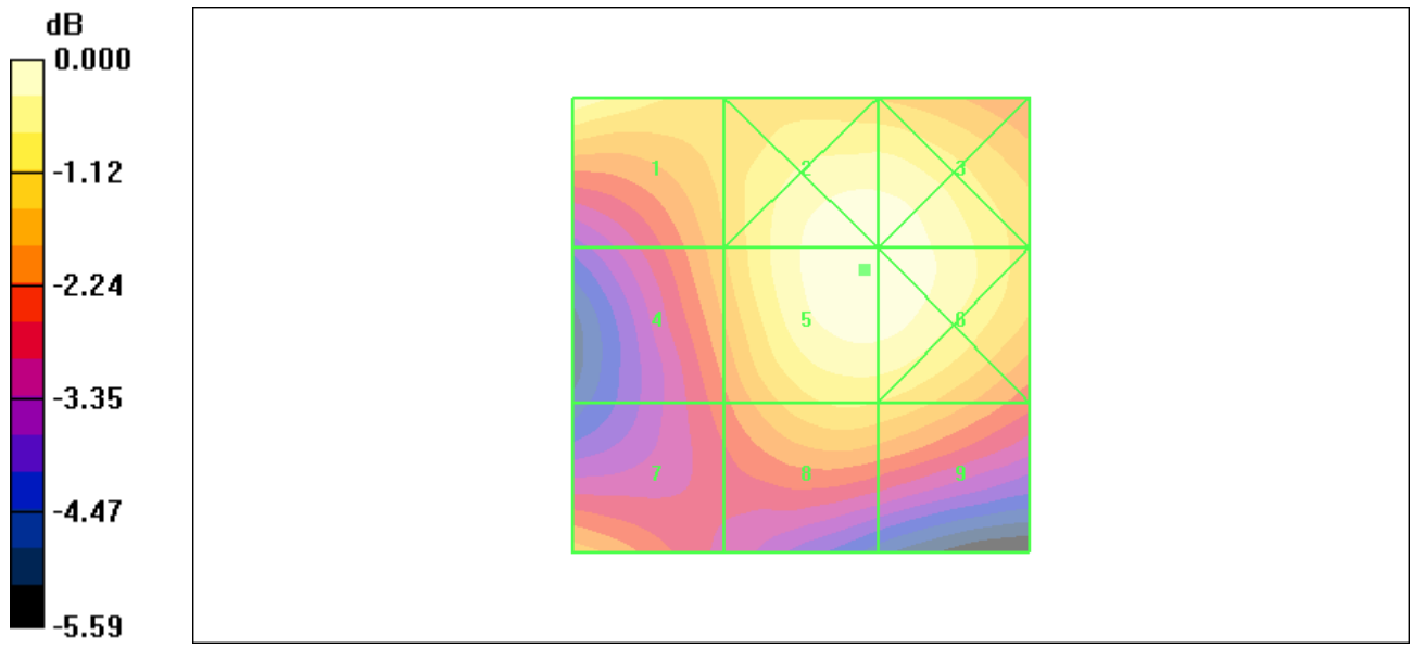
Figure 27 HAC RF H-Field GSM 1900 Channel 810
