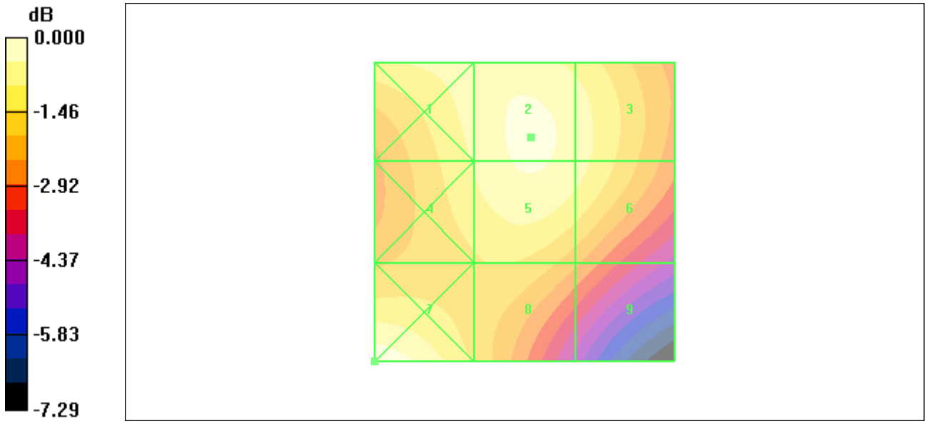
Figure 33 HAC RF H-Field WCDMA Band IV Channel 1413
