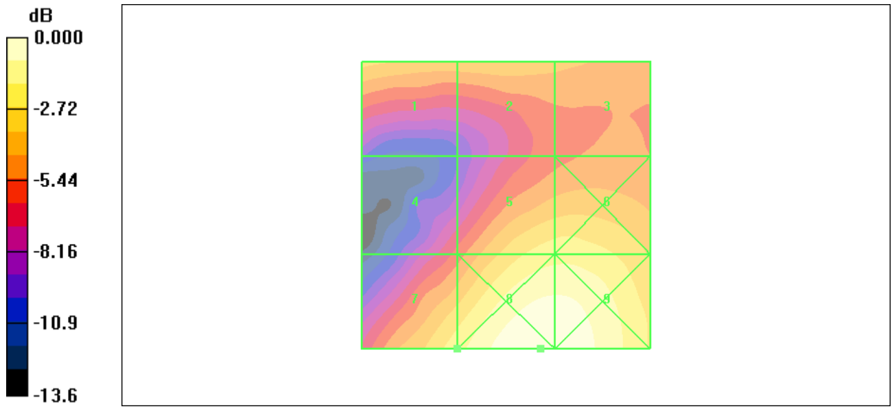
Figure 28 HAC RF E-Field WCDMA Band IV Channel 1513
