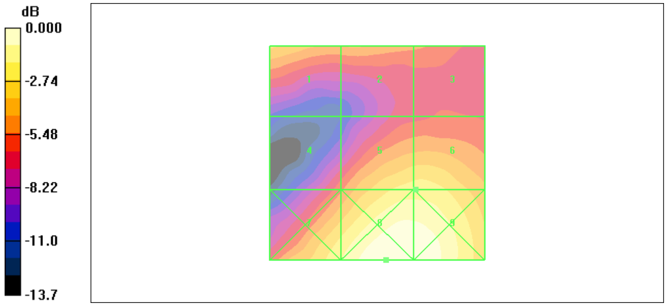
Figure 30 HAC RF E-Field WCDMA Band IV Channel 1312
