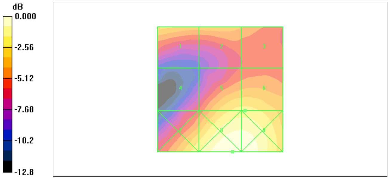
Figure 29 HAC RF E-Field WCDMA Band IV Channel 1413
