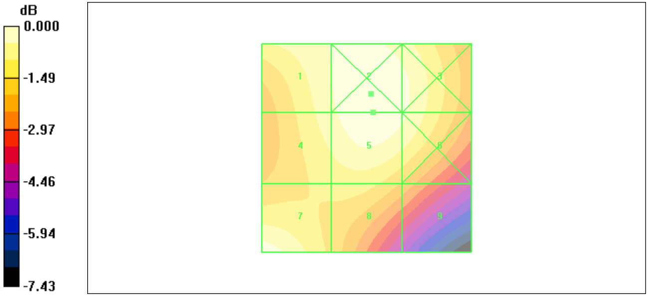
Figure 35 HAC RF H-Field WCDMA Band IV Channel 1312
