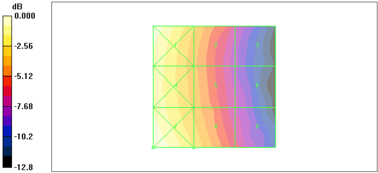
Figure 42 HAC RF H-Field WCDMA Band V Channel 4132
