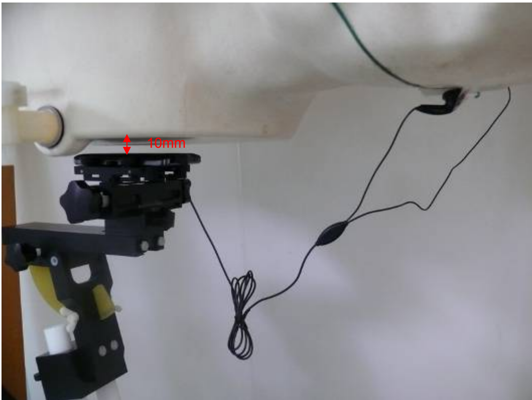
Picture 21: Back Side with Stereo Headset 1, the distance from handset to the bottom of the Phantom is 10mm (Battery 2)
