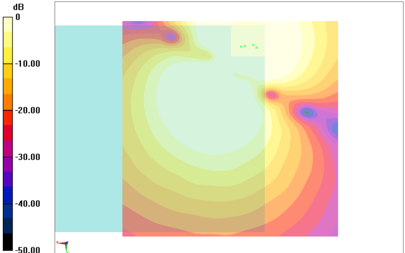
Fig B.6 T-Coil GSM 1900
