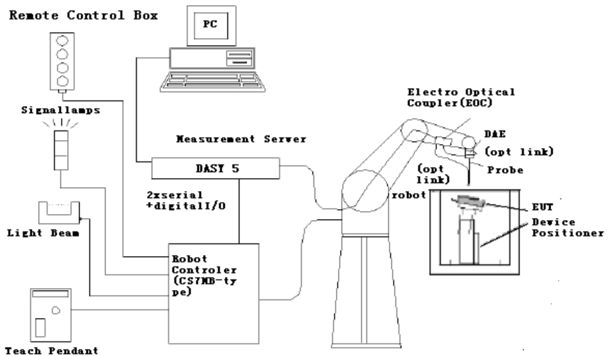
Figure 6.1 HAC Test Measurement Set-up
