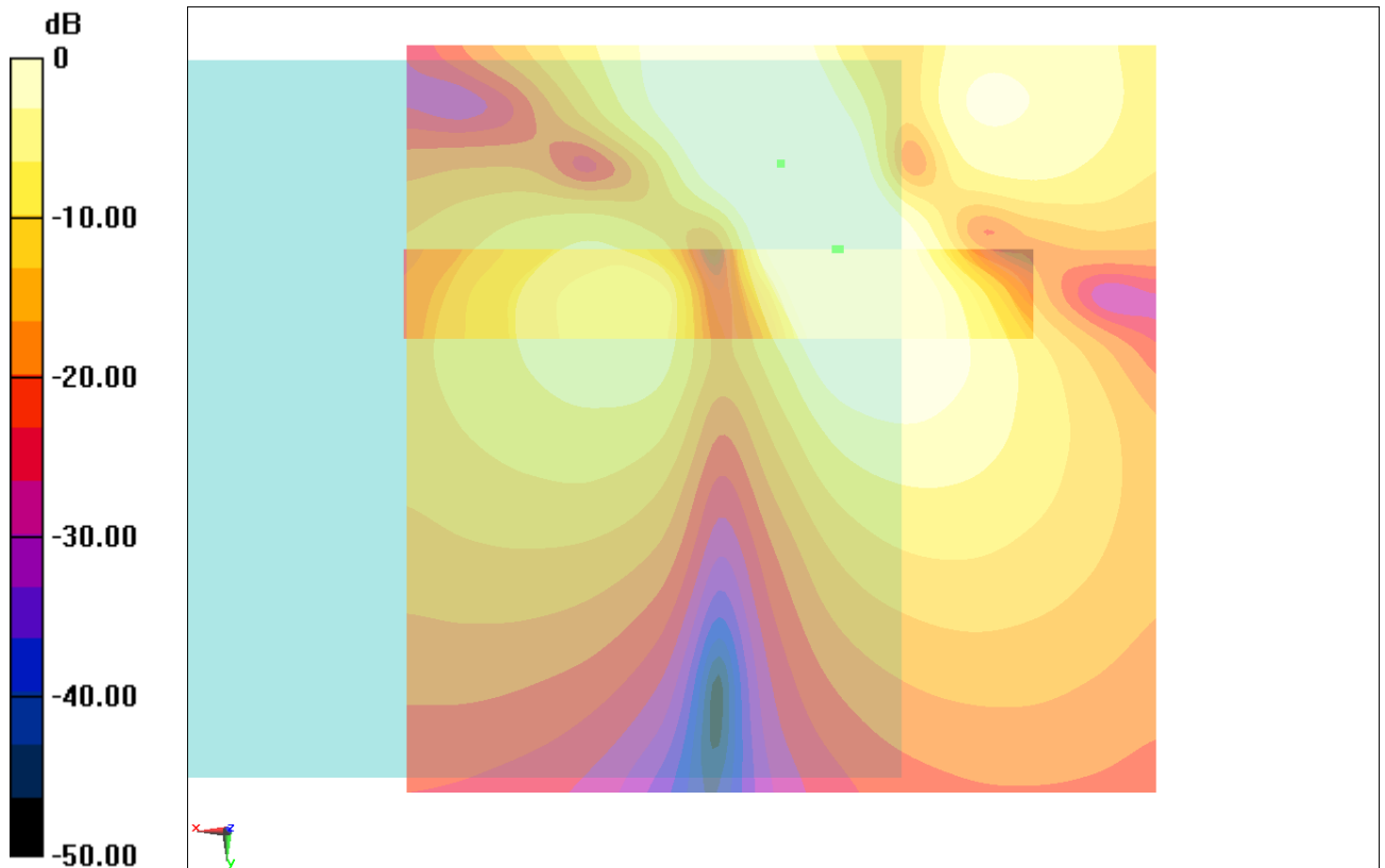
Fig B.10 T-Coil WCDMA 1900
