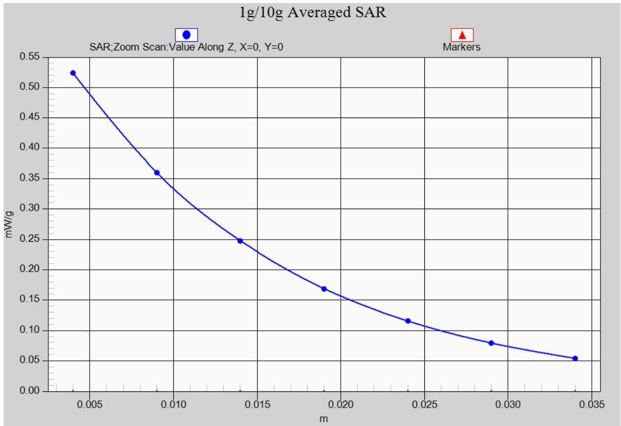
Fig. 78-1 Z-Scan at power reference point (WCDMA1900 CH9400)
