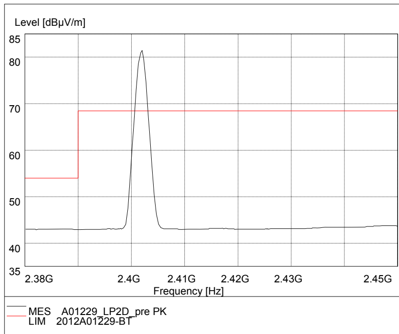
Fig.79. Radiated emission (Power): \pi/4 DQPSK, low channel Fig.80.
