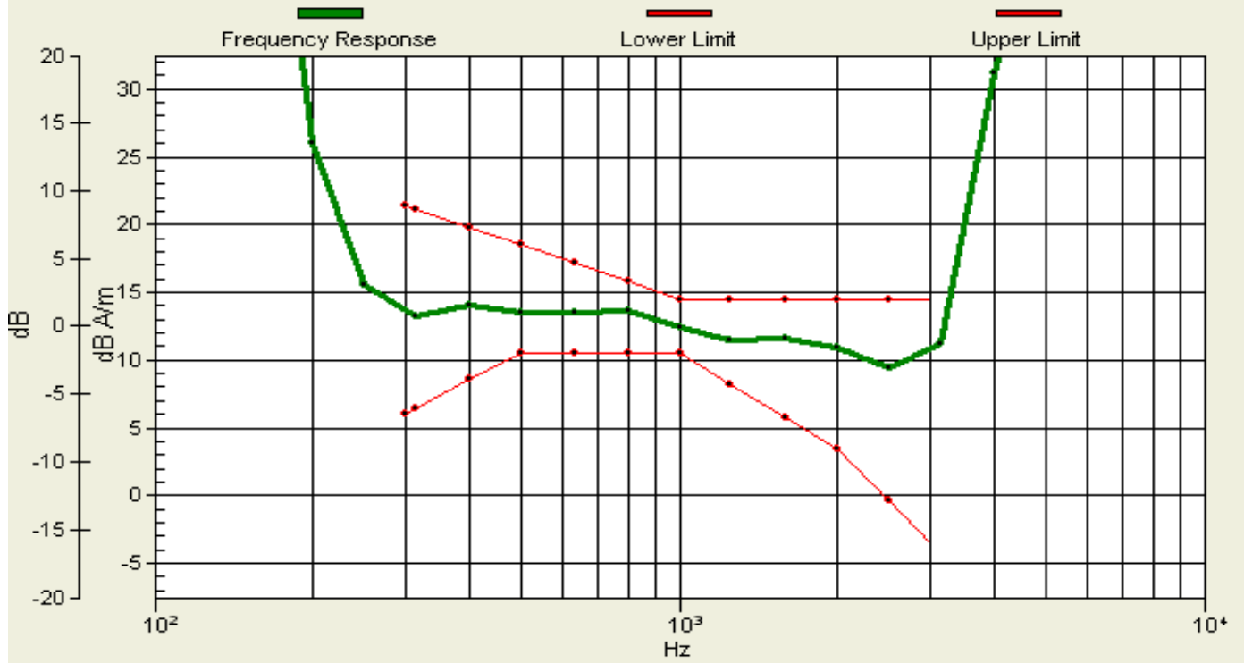
Scans/z (axial) wideband at best S/N/ABM Freq Resp(x,y,z,f)
