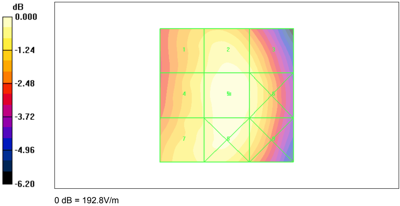
Figure 15 HAC RF E-Field GSM 850 Channel 190
