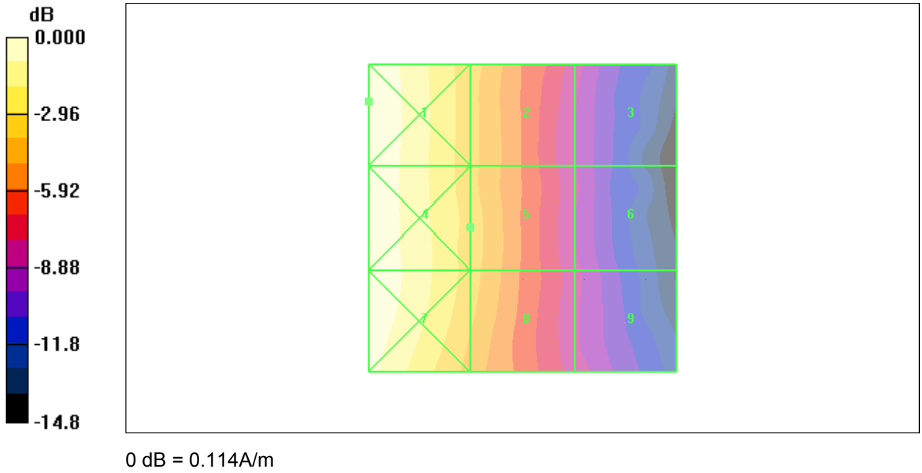
Figure 42 HAC RF H-Field WCDMA Band V Channel 4132
