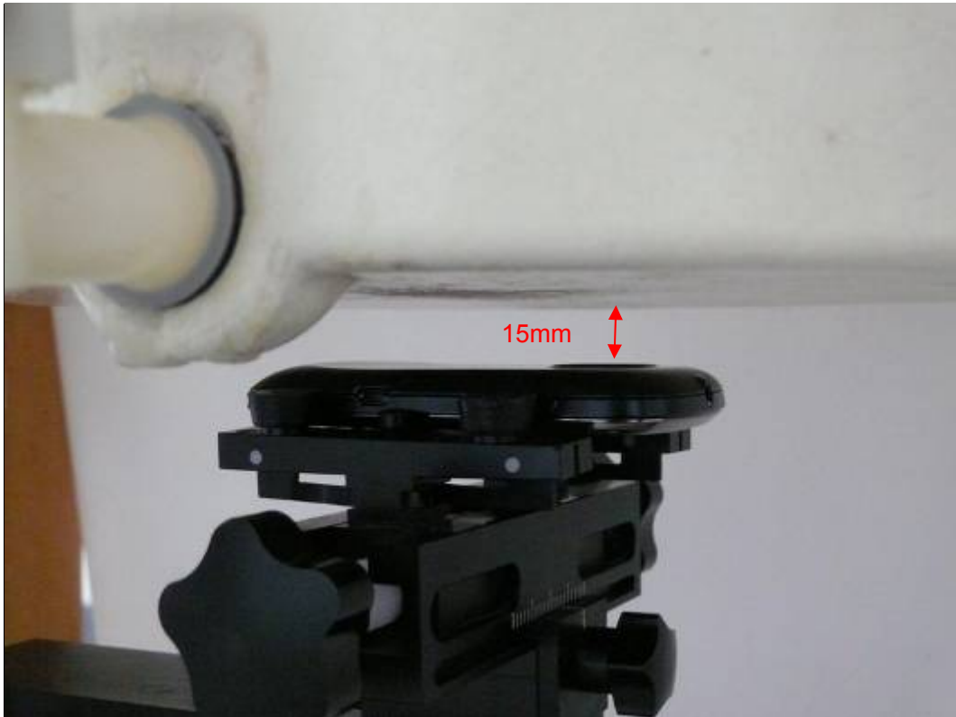
Picture 13: Body, The EUT display towards ground, the distance from EUT to the bottom of the Phantom is 15mm (Battery 2)
