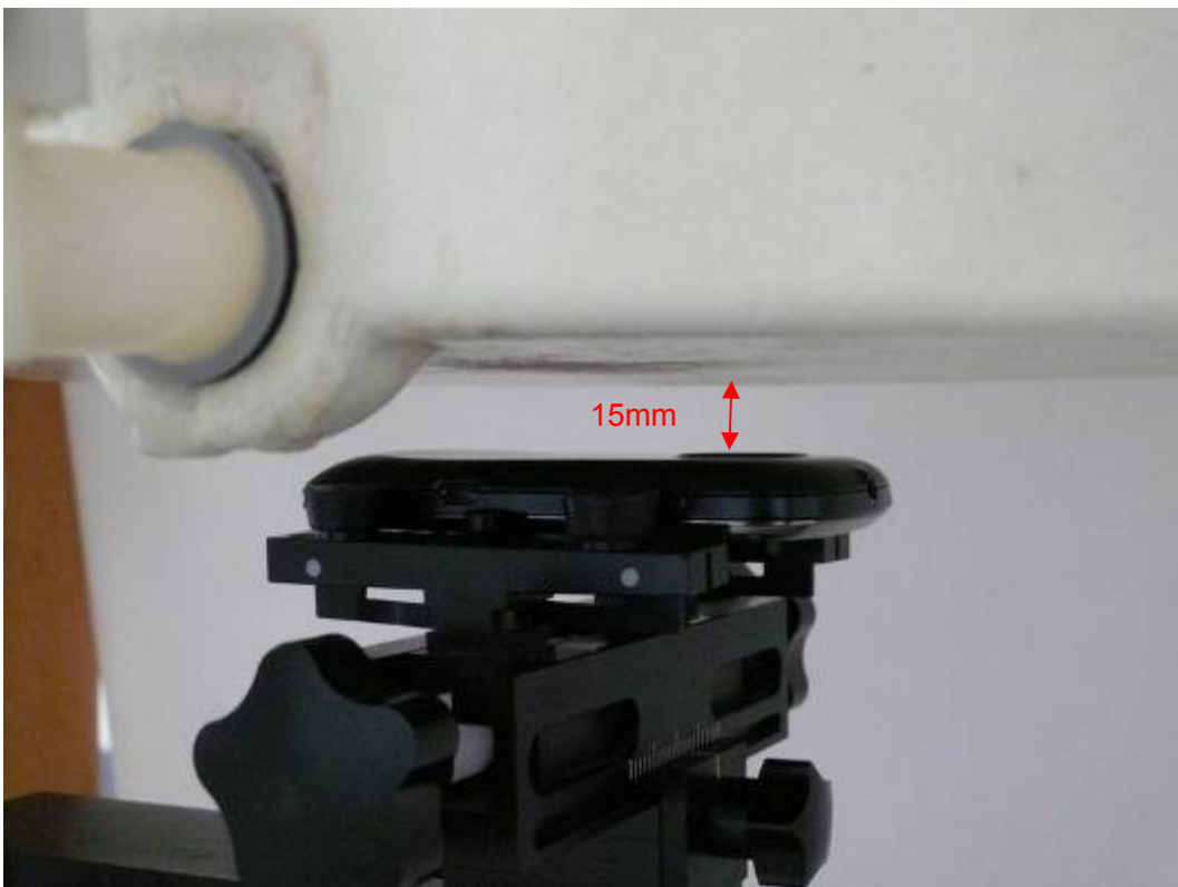
Picture 12: Body, The EUT display towards ground, the distance from EUT to the bottom of the Phantom is 15mm (Battery 1)
