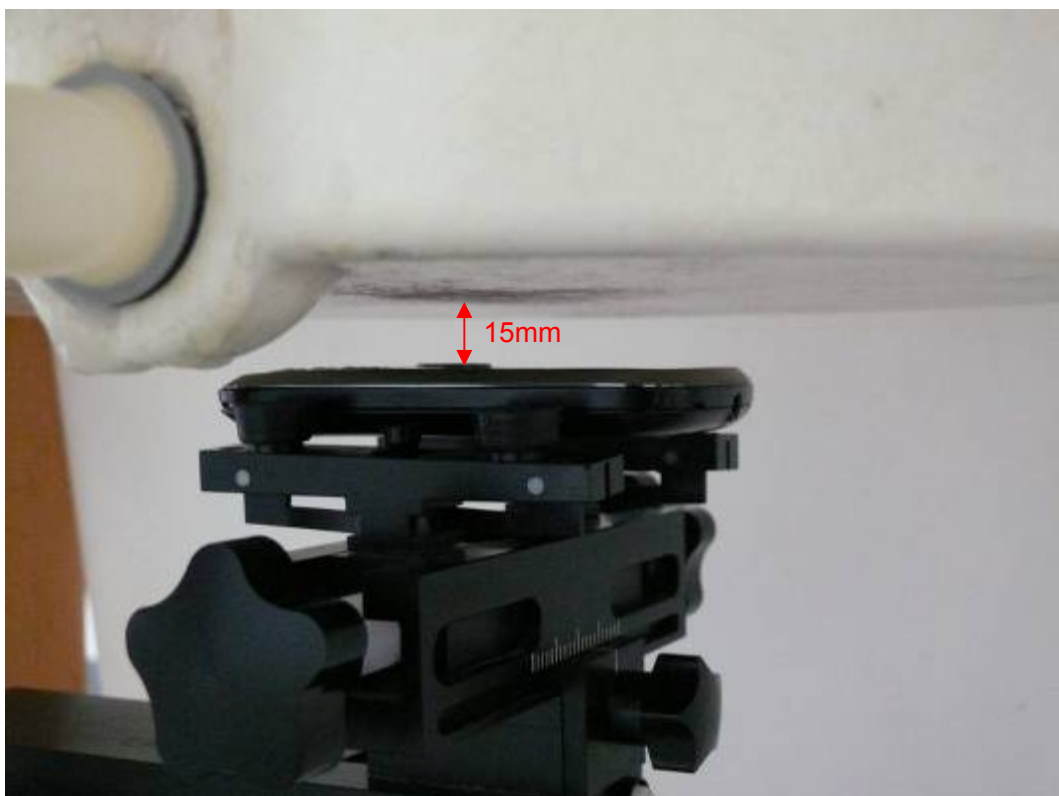
Picture 14: Body, The EUT display towards phantom, the distance from EUT to the bottom of the Phantom is 15mm (Battery 1)
